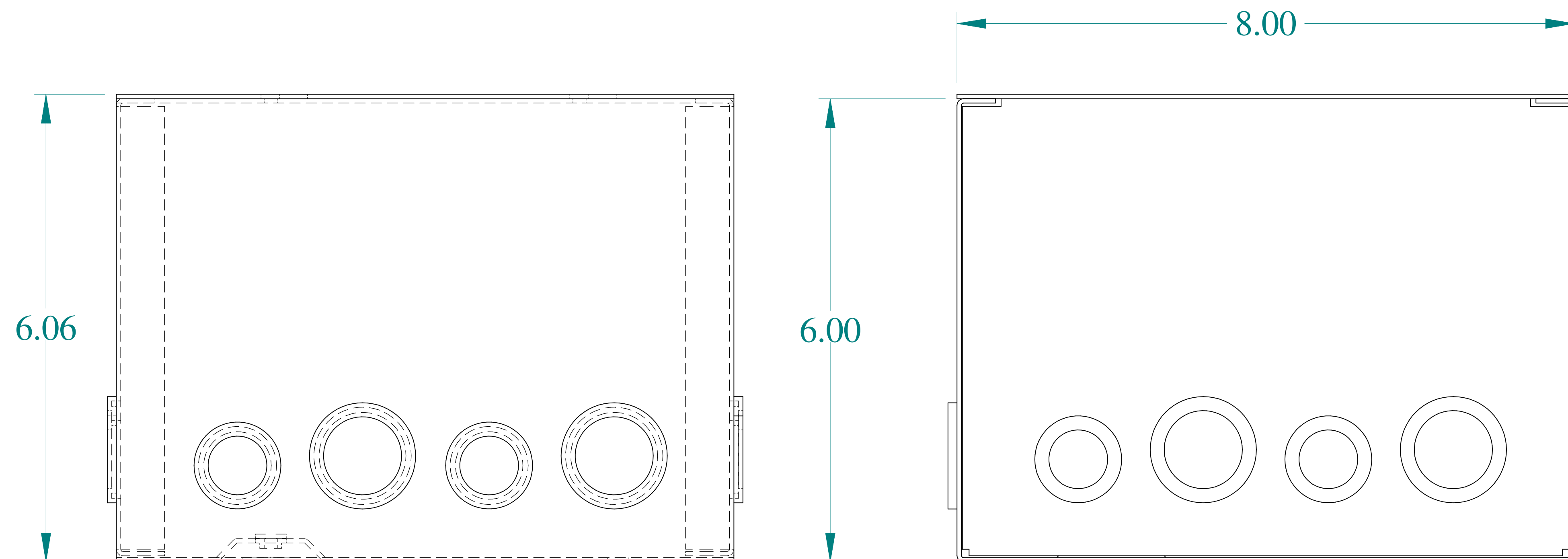
FRONT VIEW
