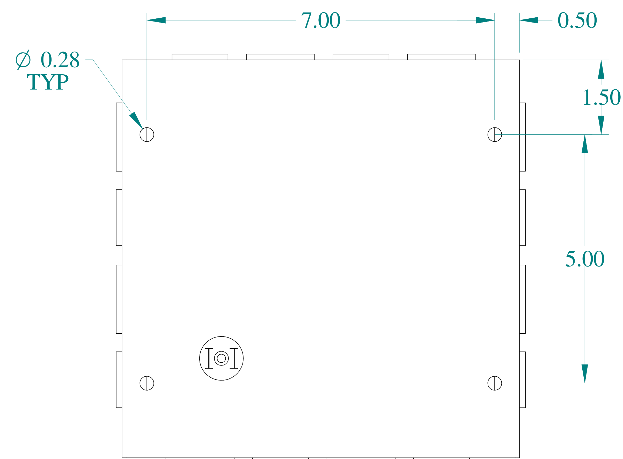
BOTTOM VIEW
