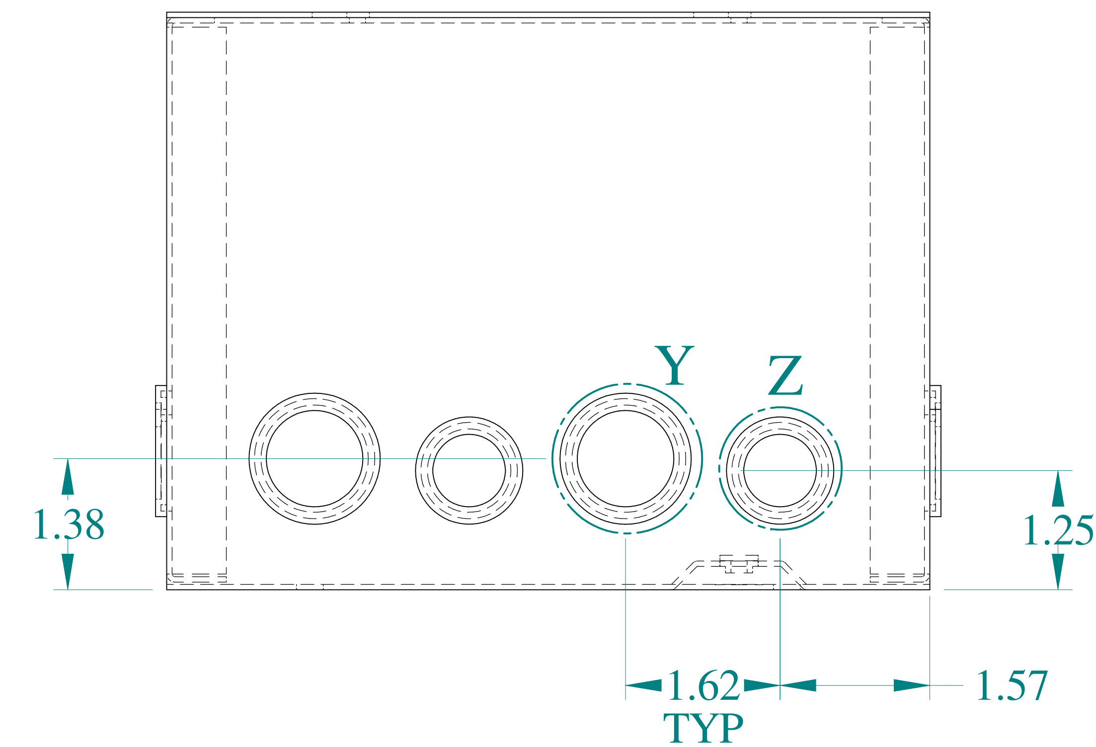
SIDE VIEW
