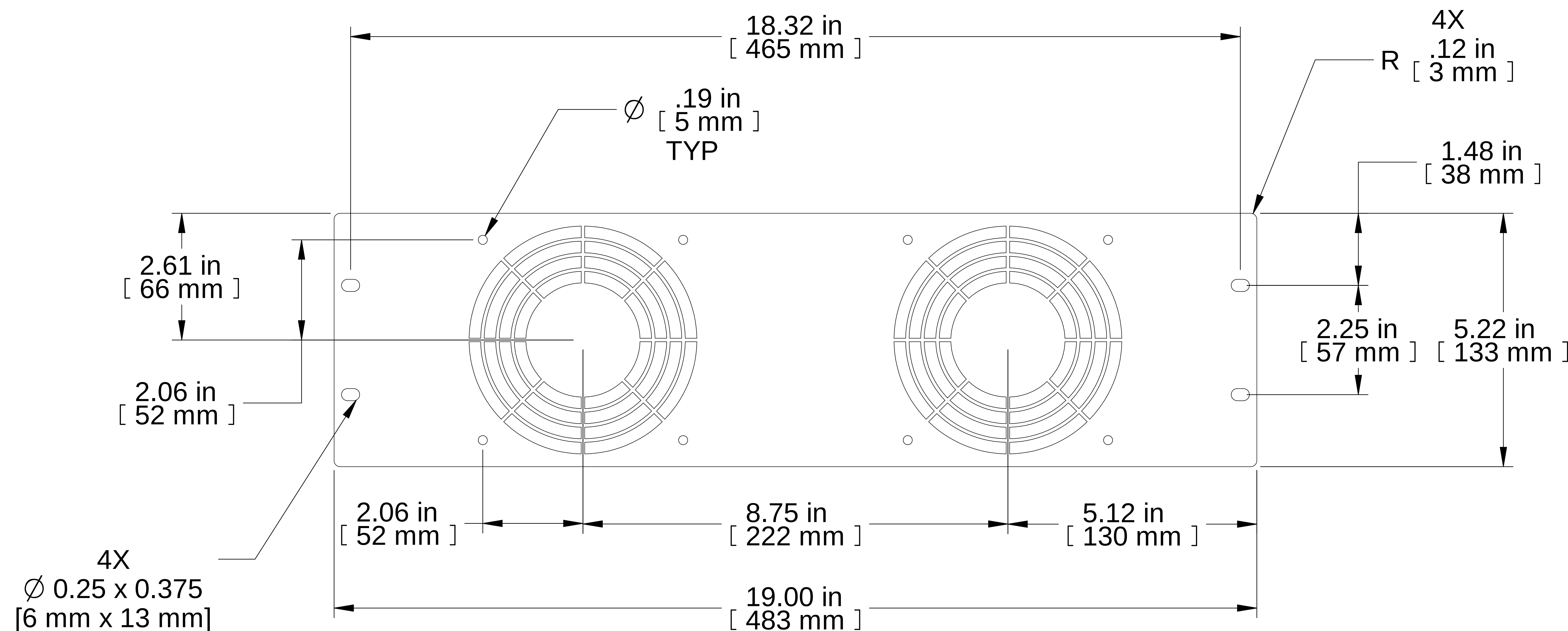
FRONT VIEW
