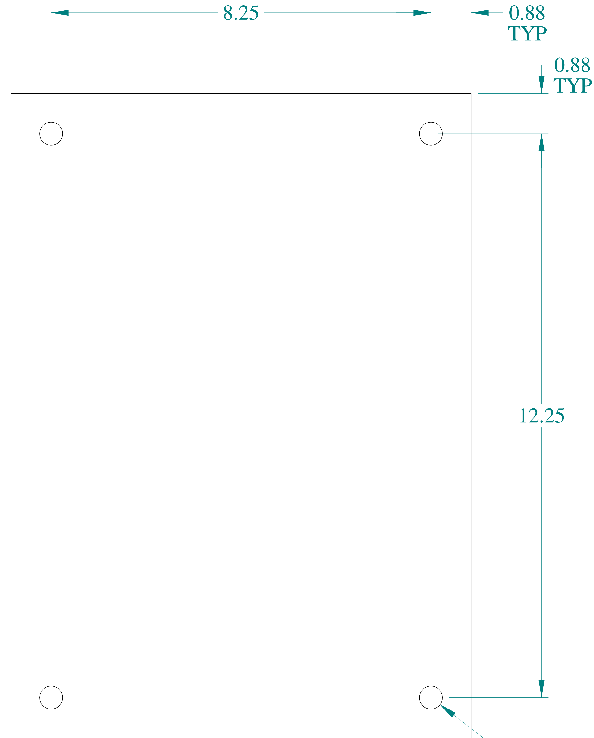
FRONT VIEW
