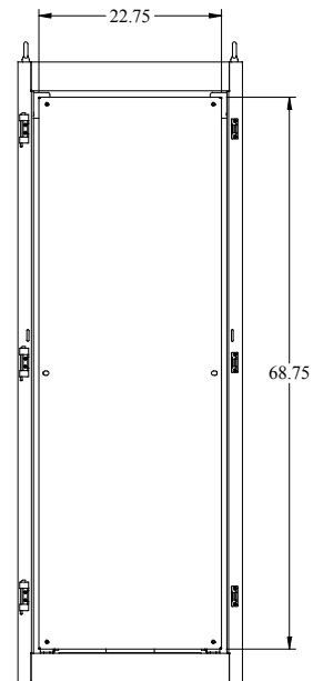
FRONT DOOR REMOVED
