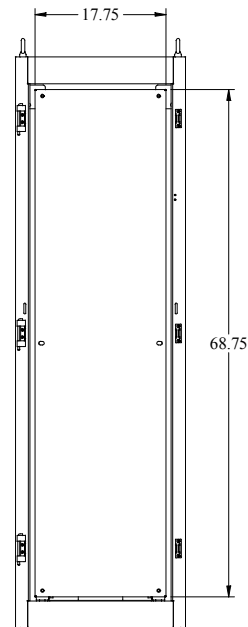
FRONT DOORREMOVED
