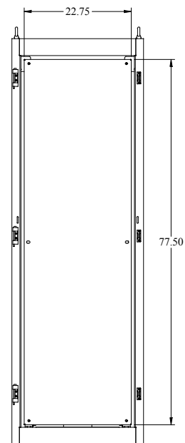
FRONT DOOR REMOVED
