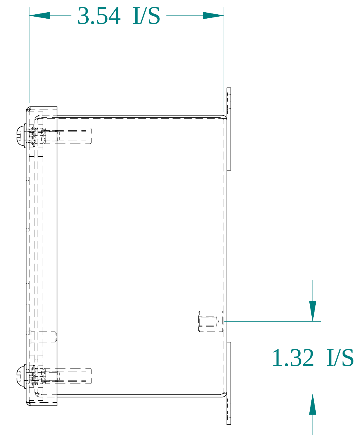
SIDE VIEW
