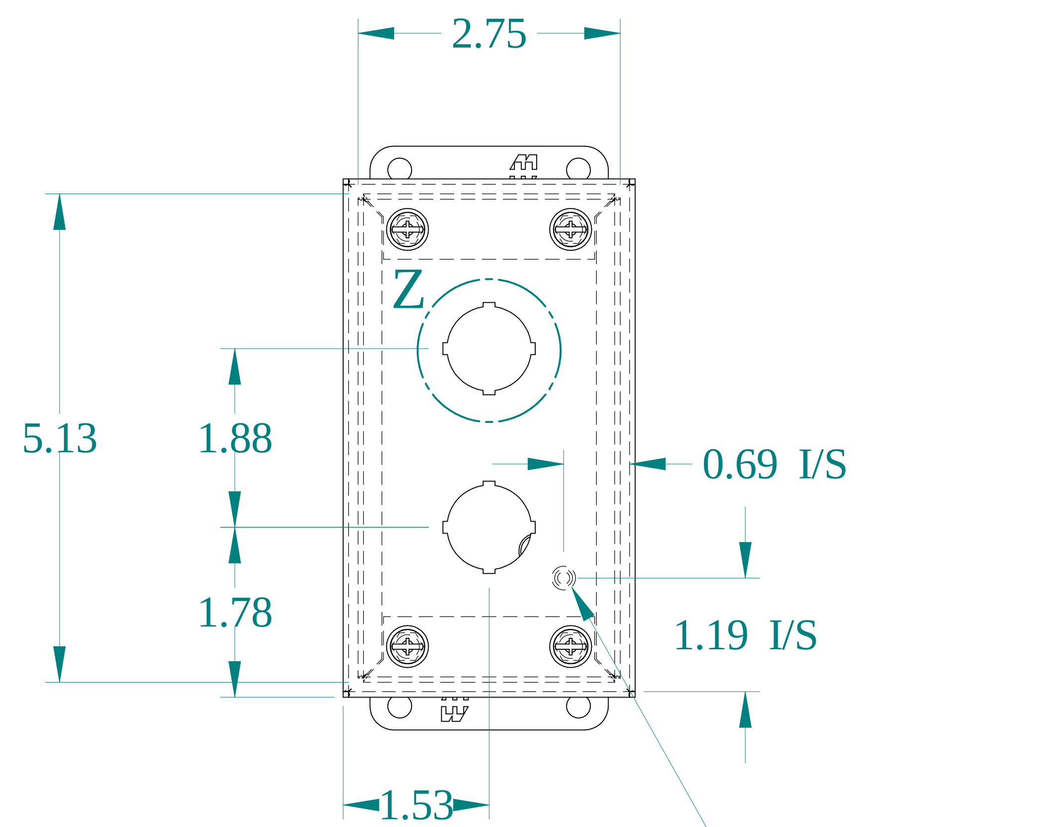
FRONT VIEW
