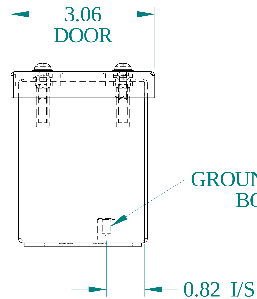
BOTTOM VIEW
