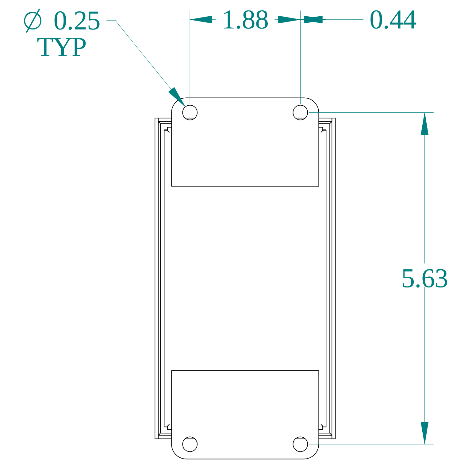
BACK VIEW
