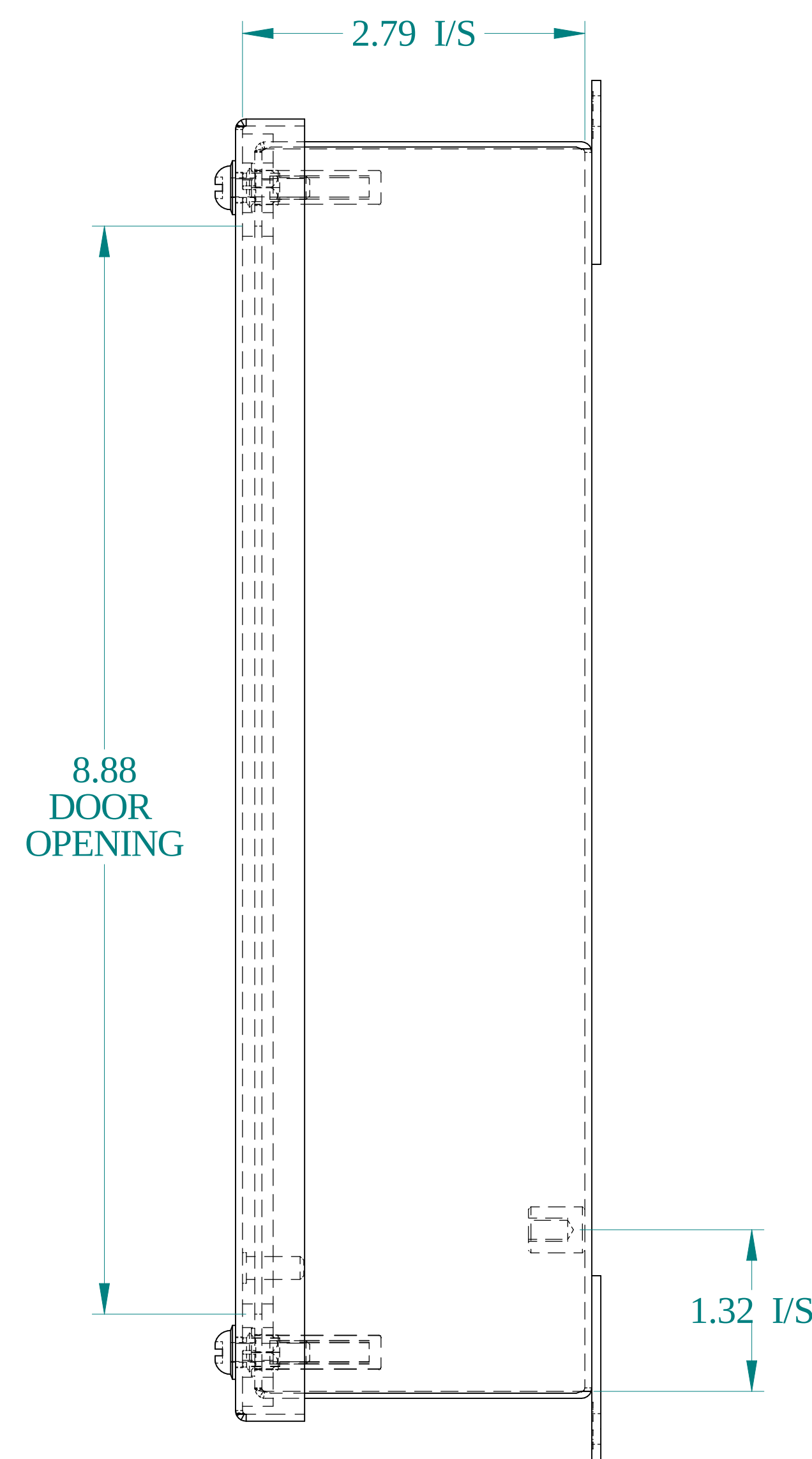
SIDE VIEW
