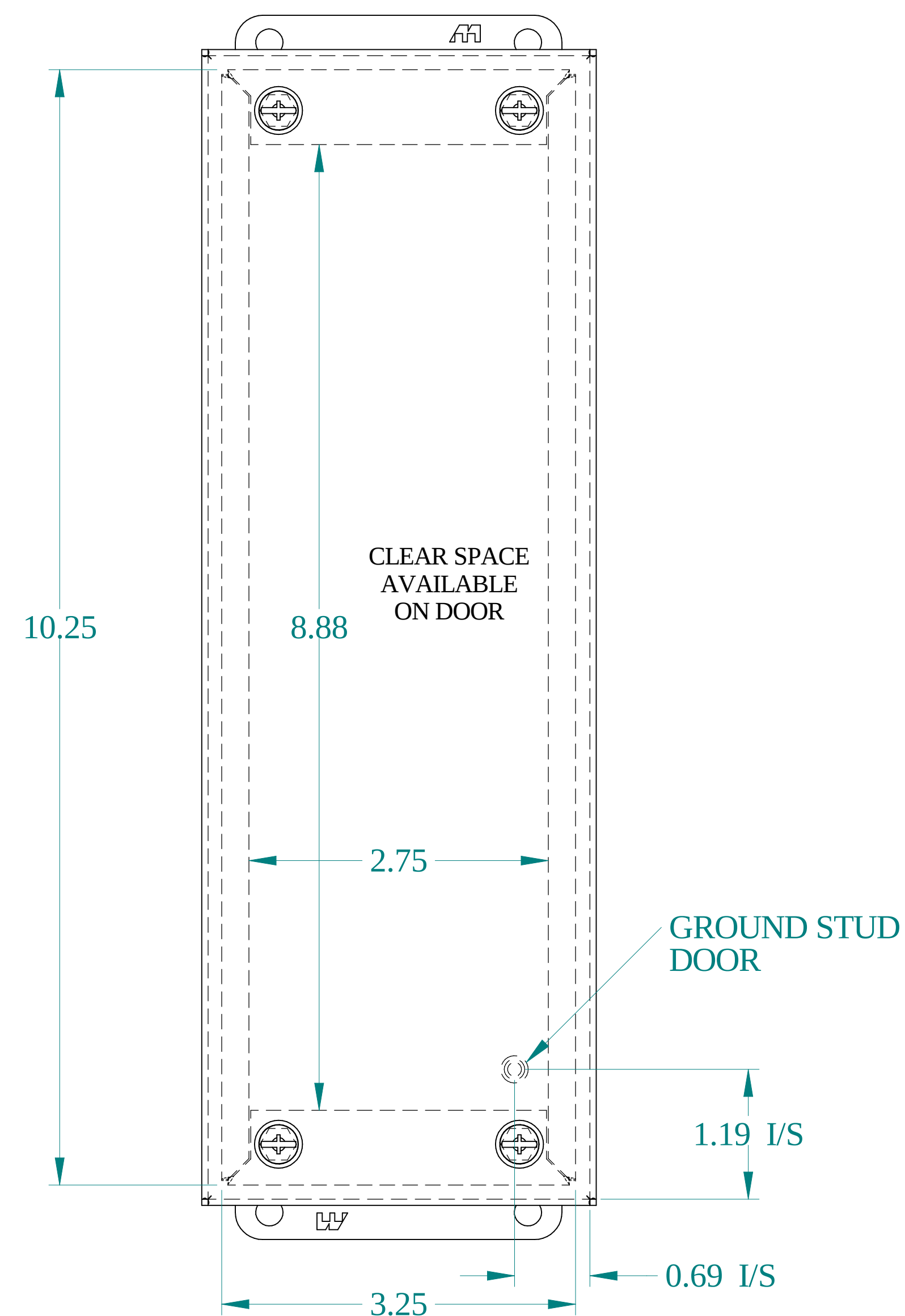
FRONT VIEW
