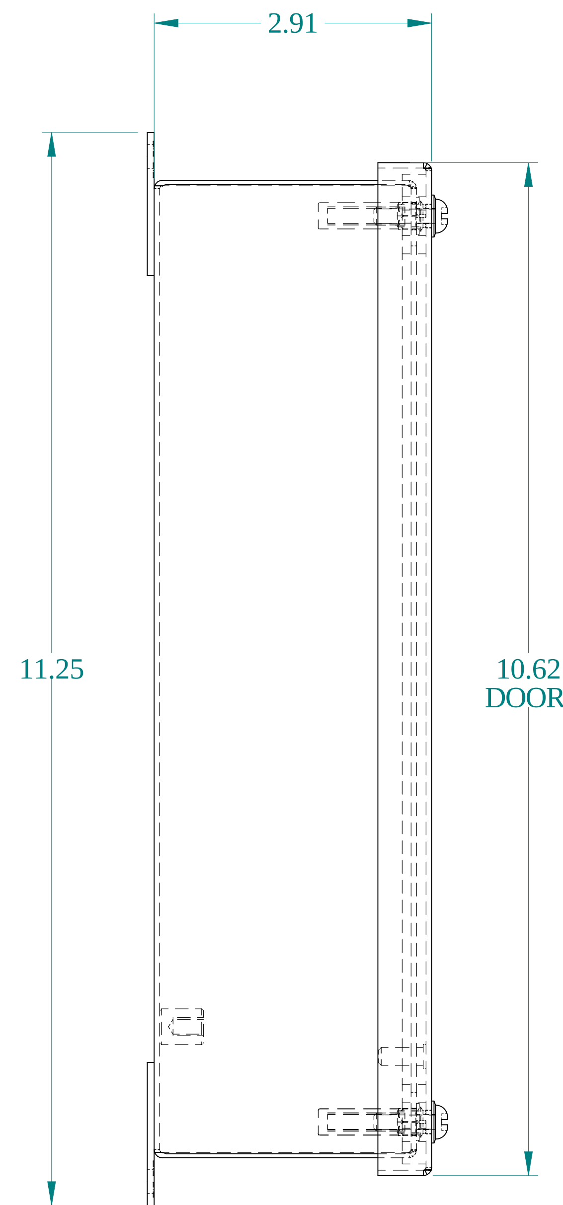
SIDE VIEW
