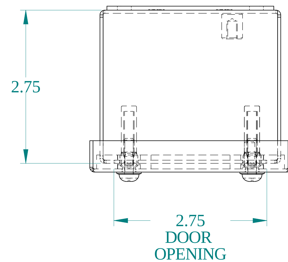
TOP VIEW
