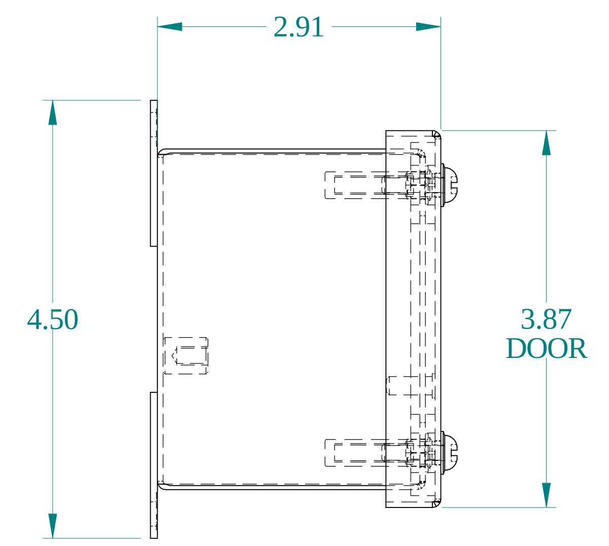
SIDE VIEW
