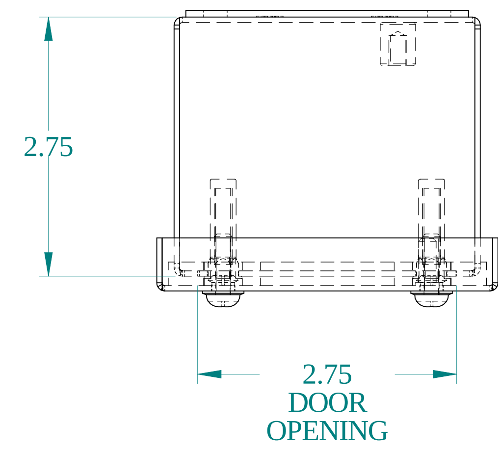
TOP VIEW
