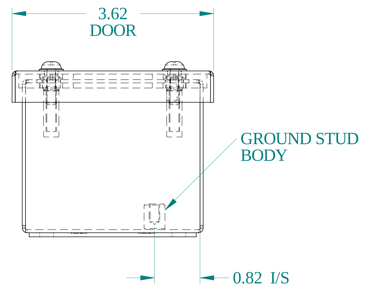
BOTTOM VIEW
