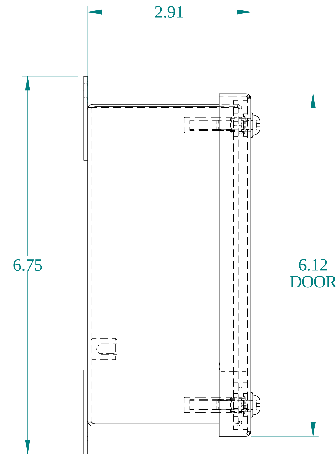
SIDE VIEW
