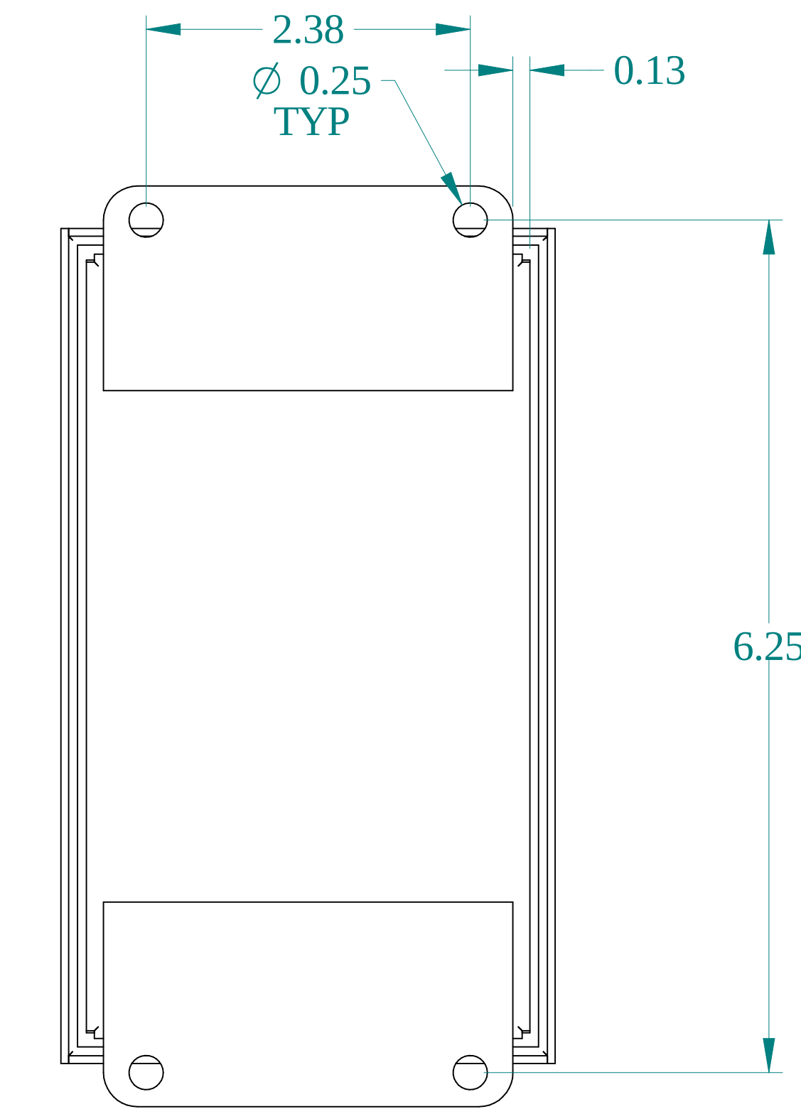
BACK VIEW
