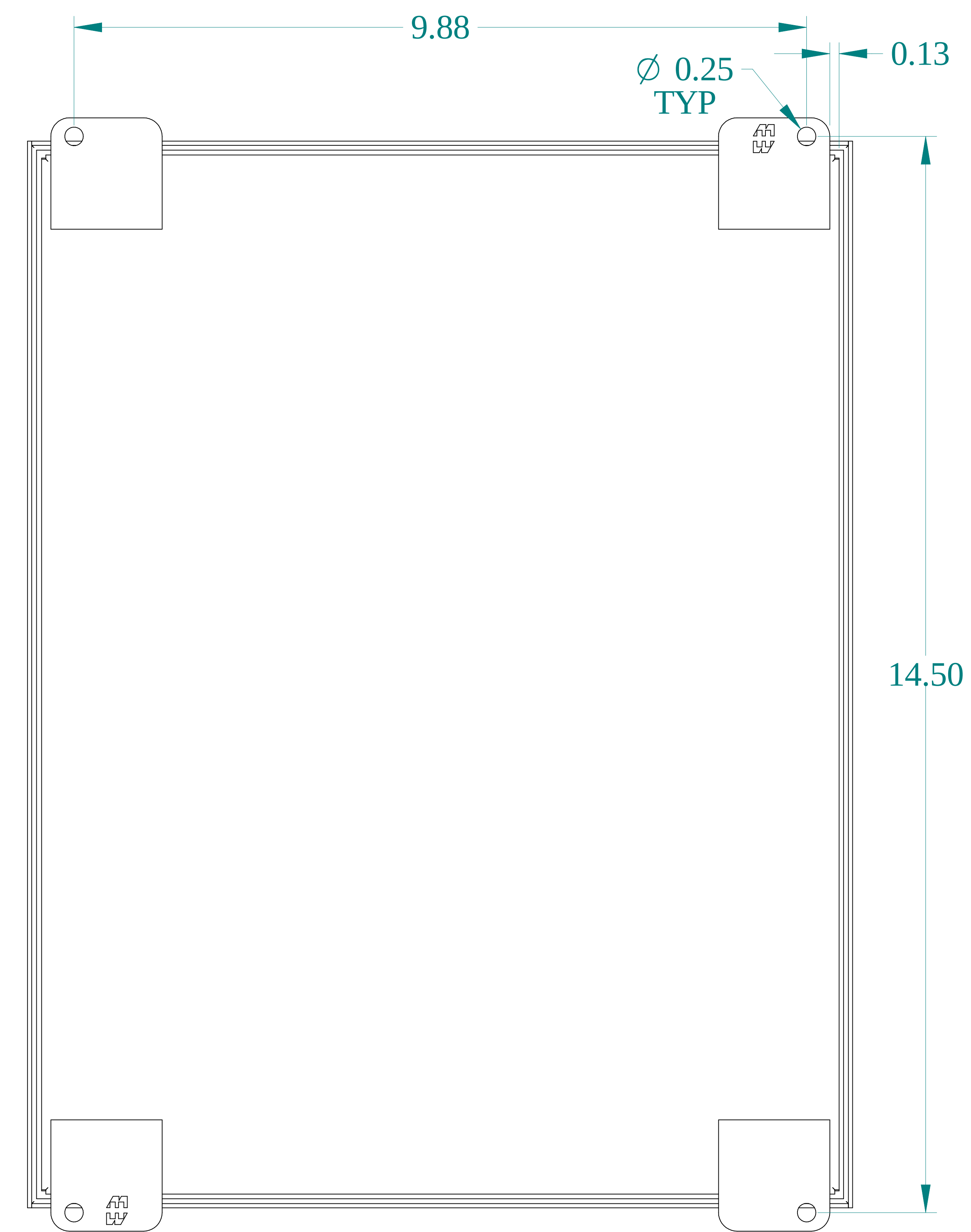
BACK VIEW
