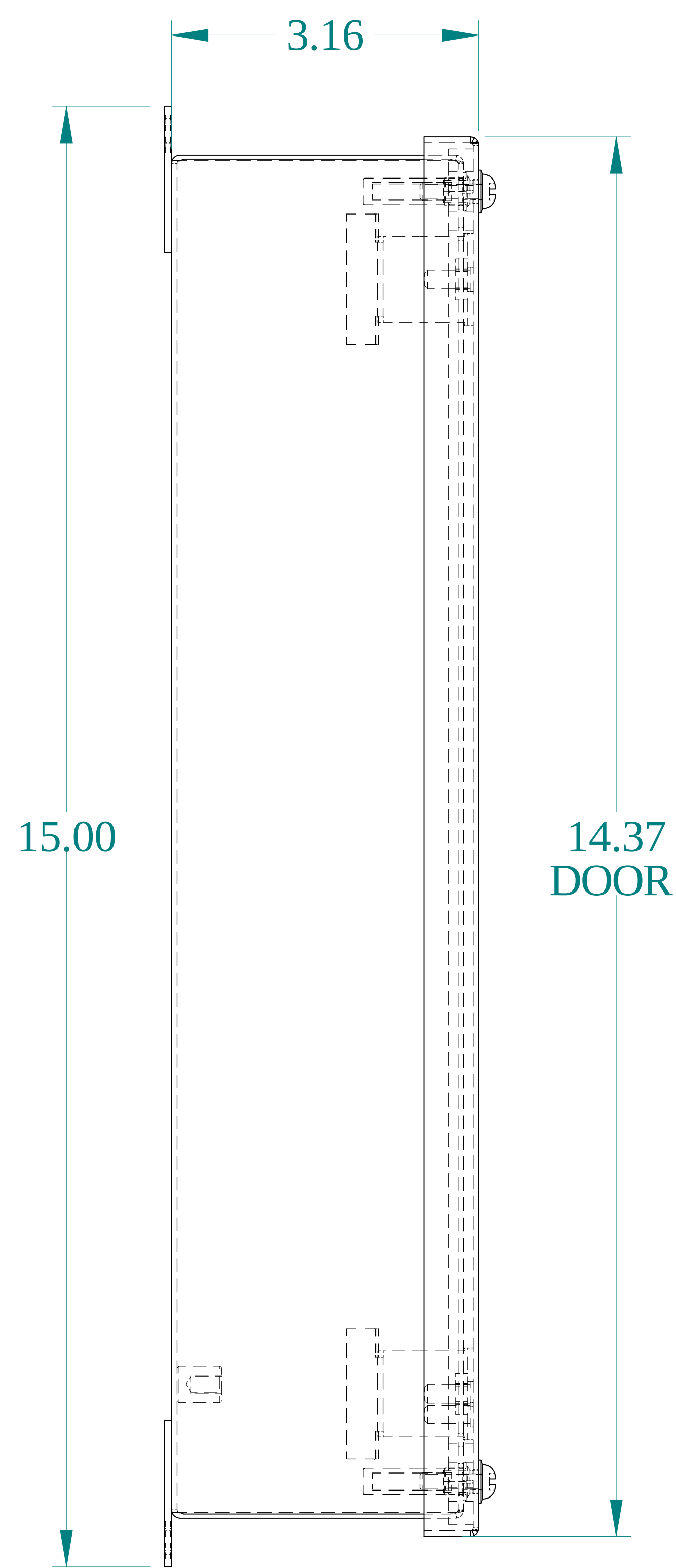
SIDE VIEW
