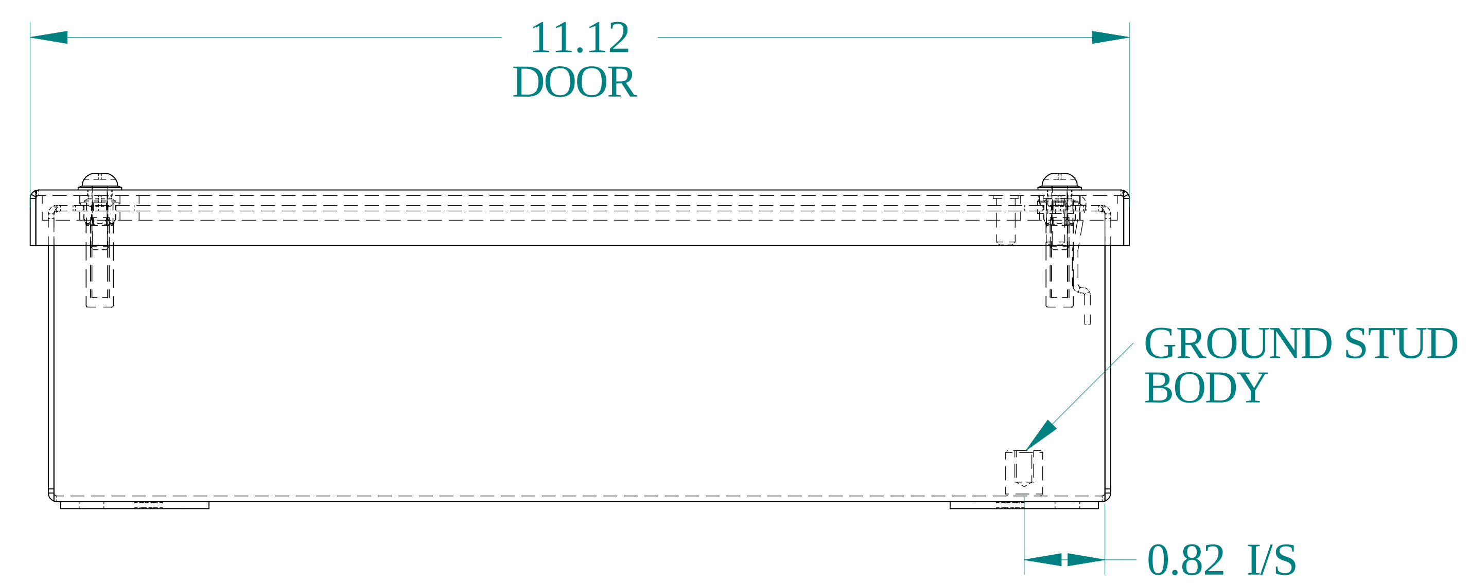
BOTTOM VIEW
