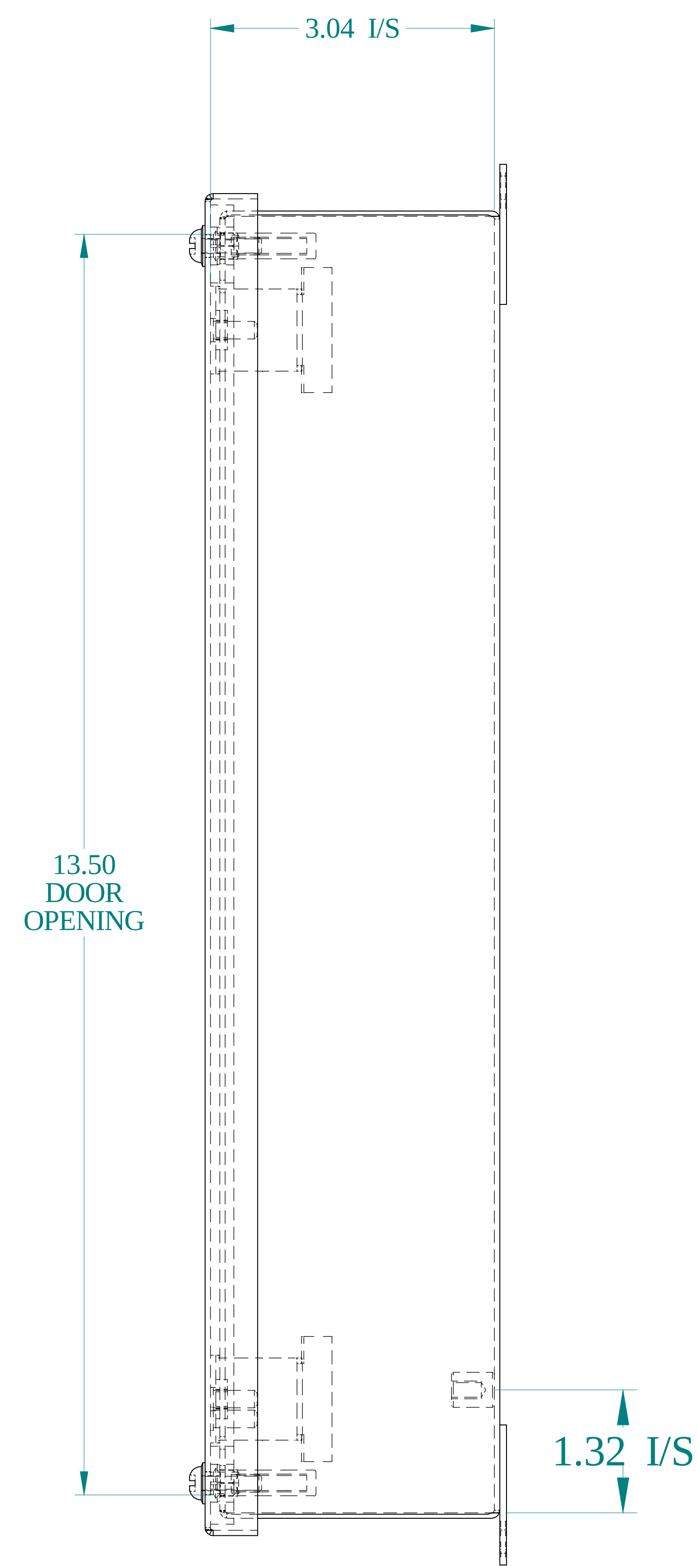
SIDE VIEW
