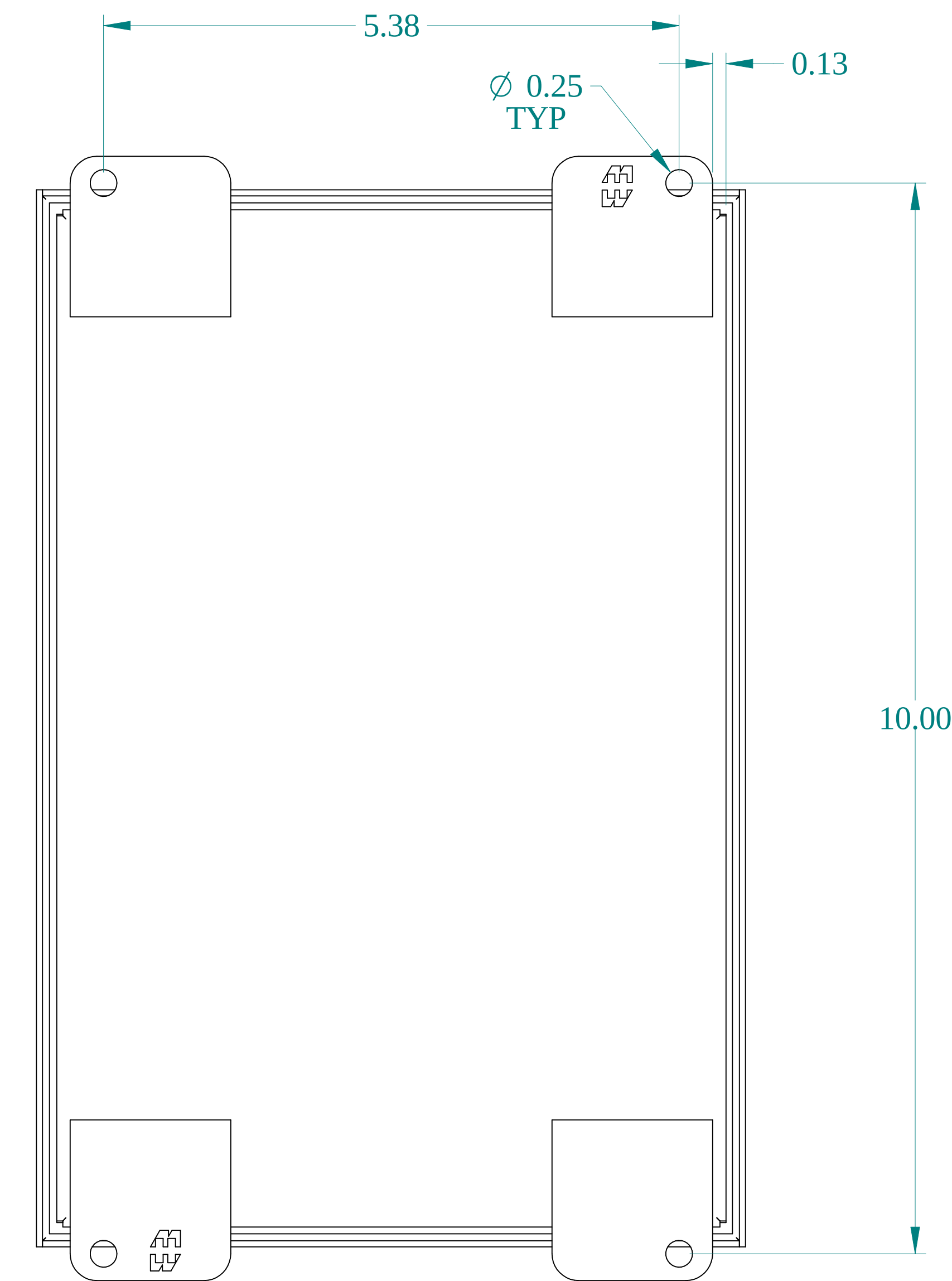
BACK VIEW
