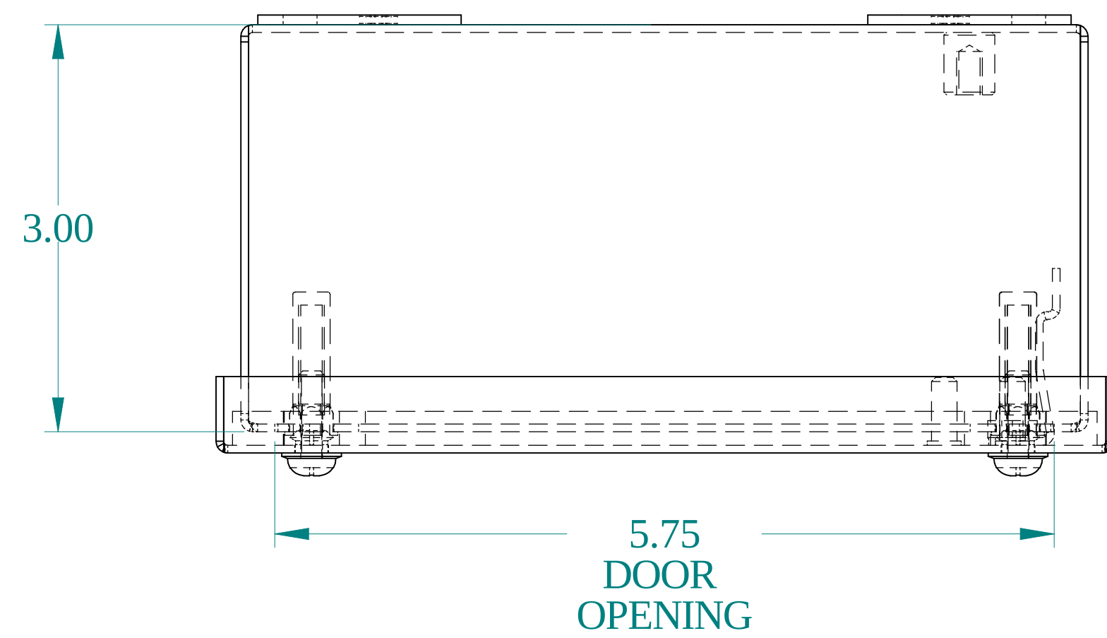
TOP VIEW
