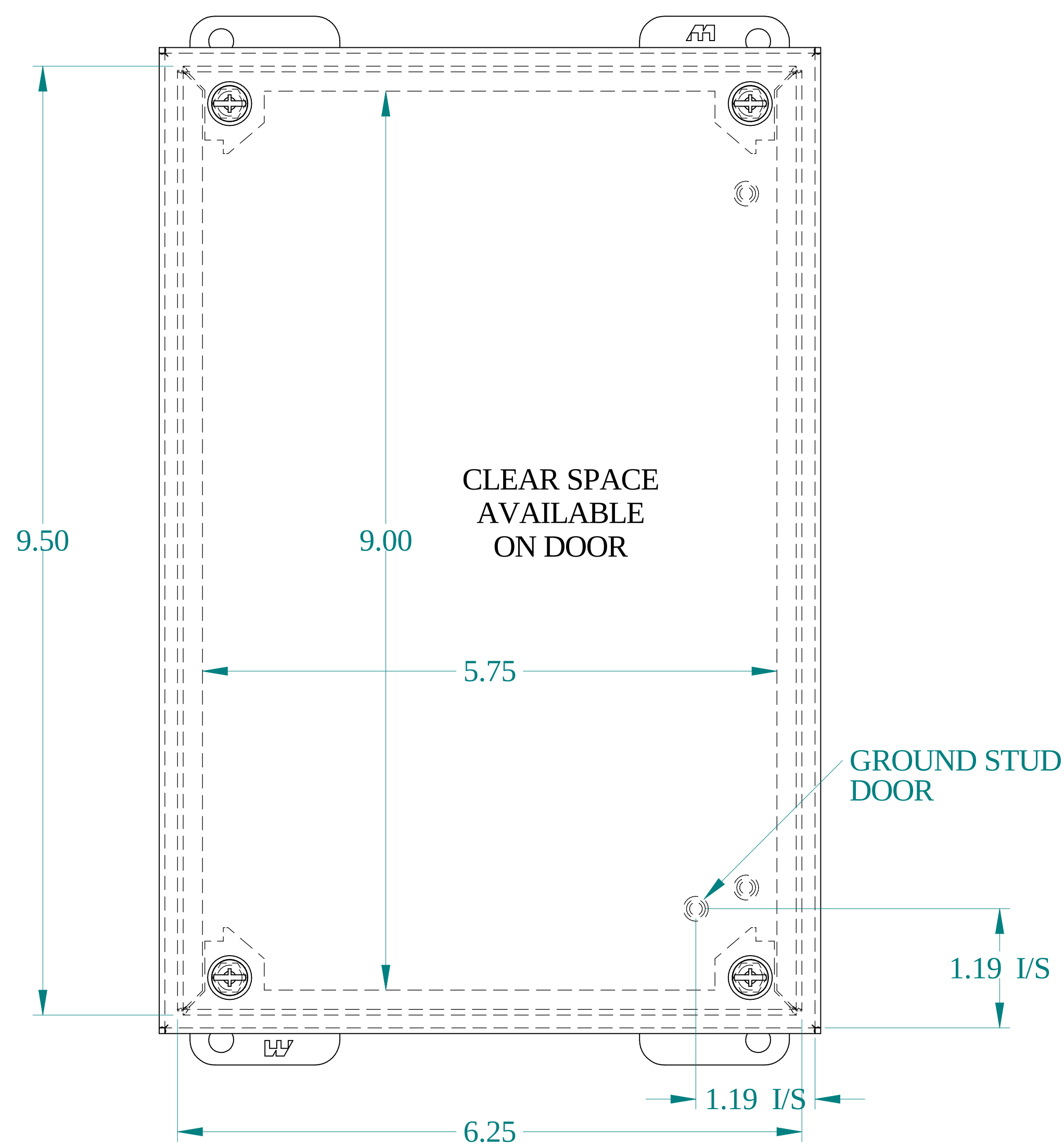
FRONT VIEW
