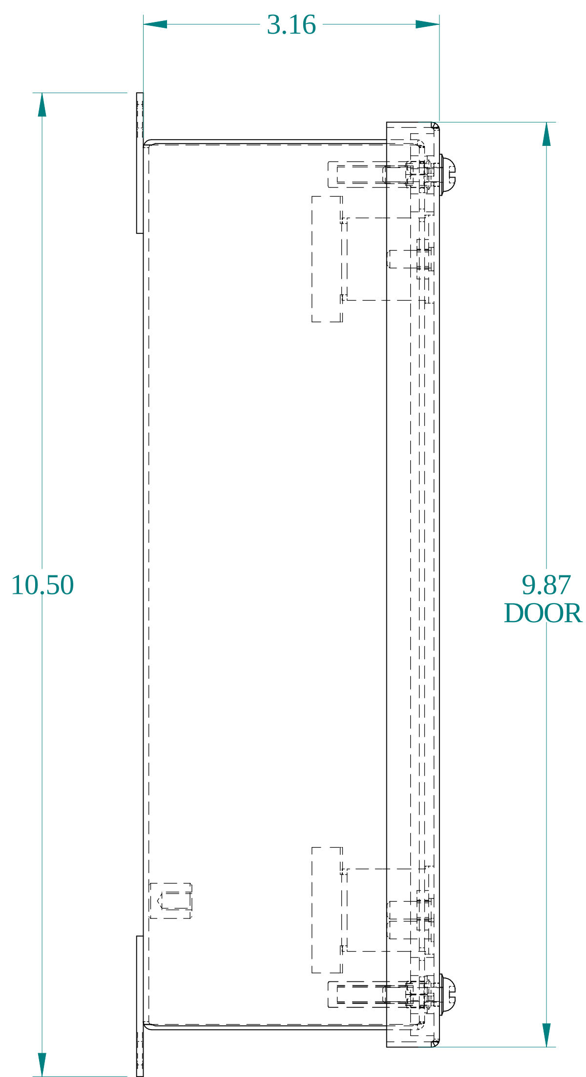
SIDE VIEW
