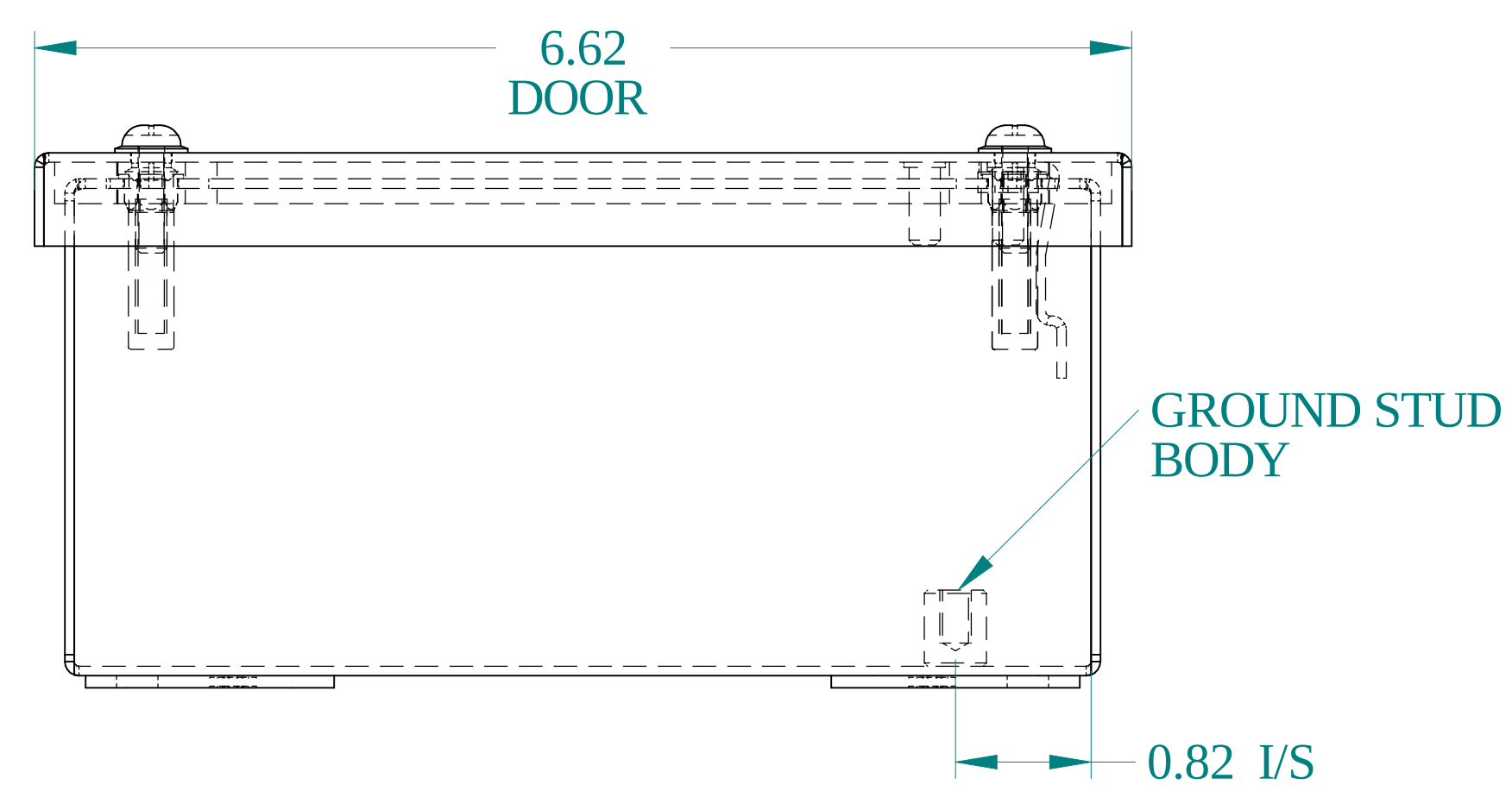
BOTTOM VIEW
