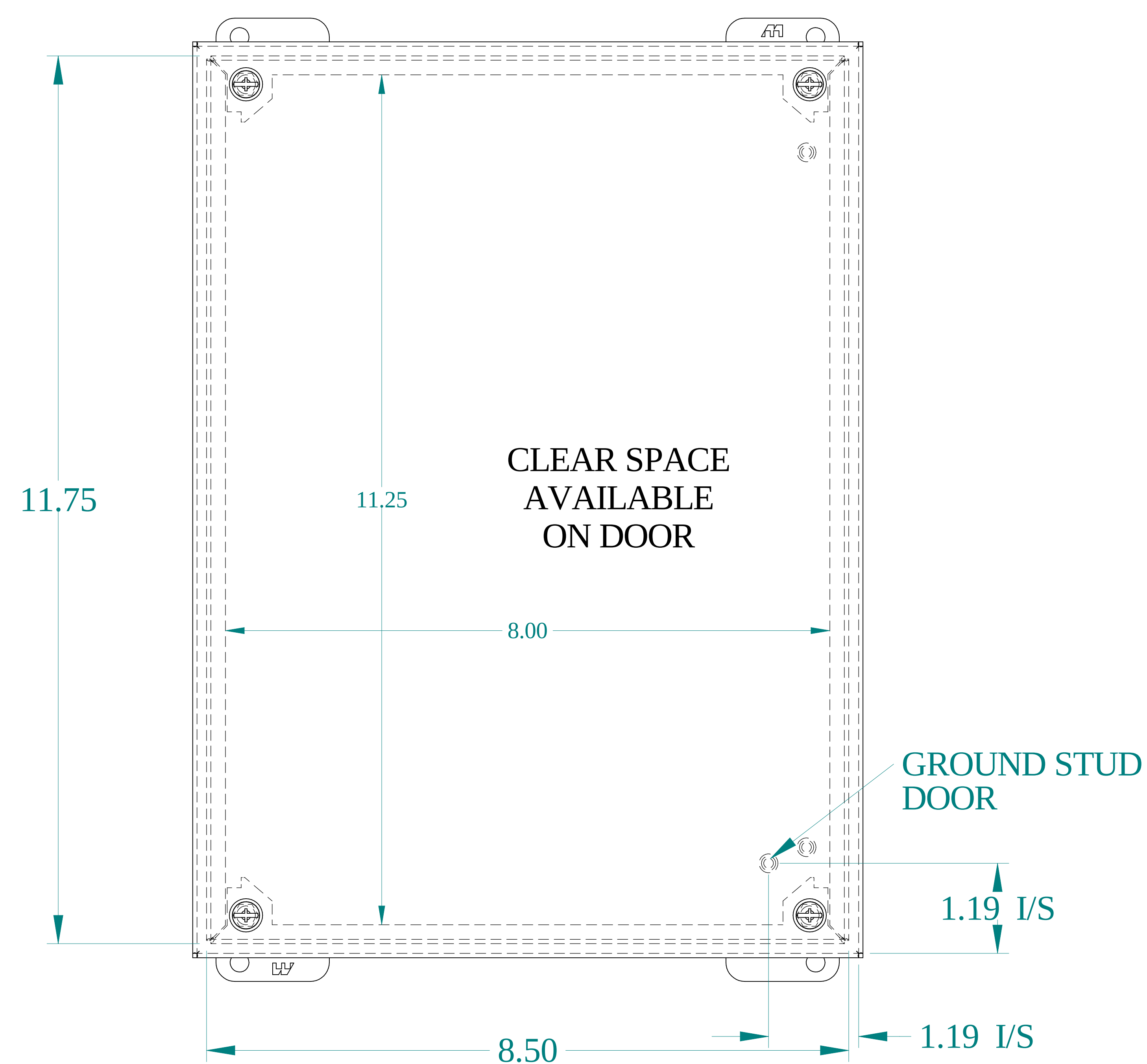
FRONT VIEW
