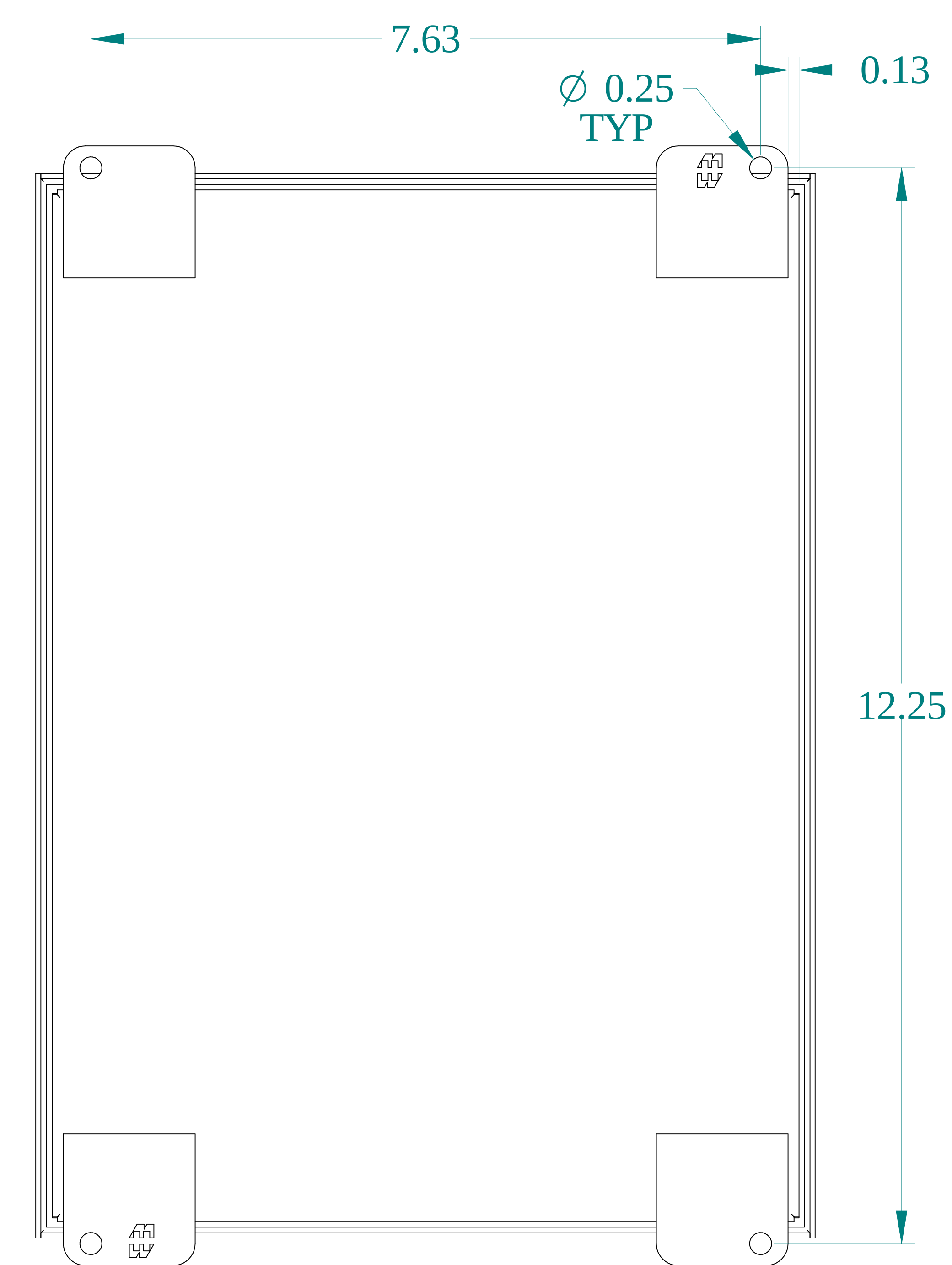
BACK VIEW
