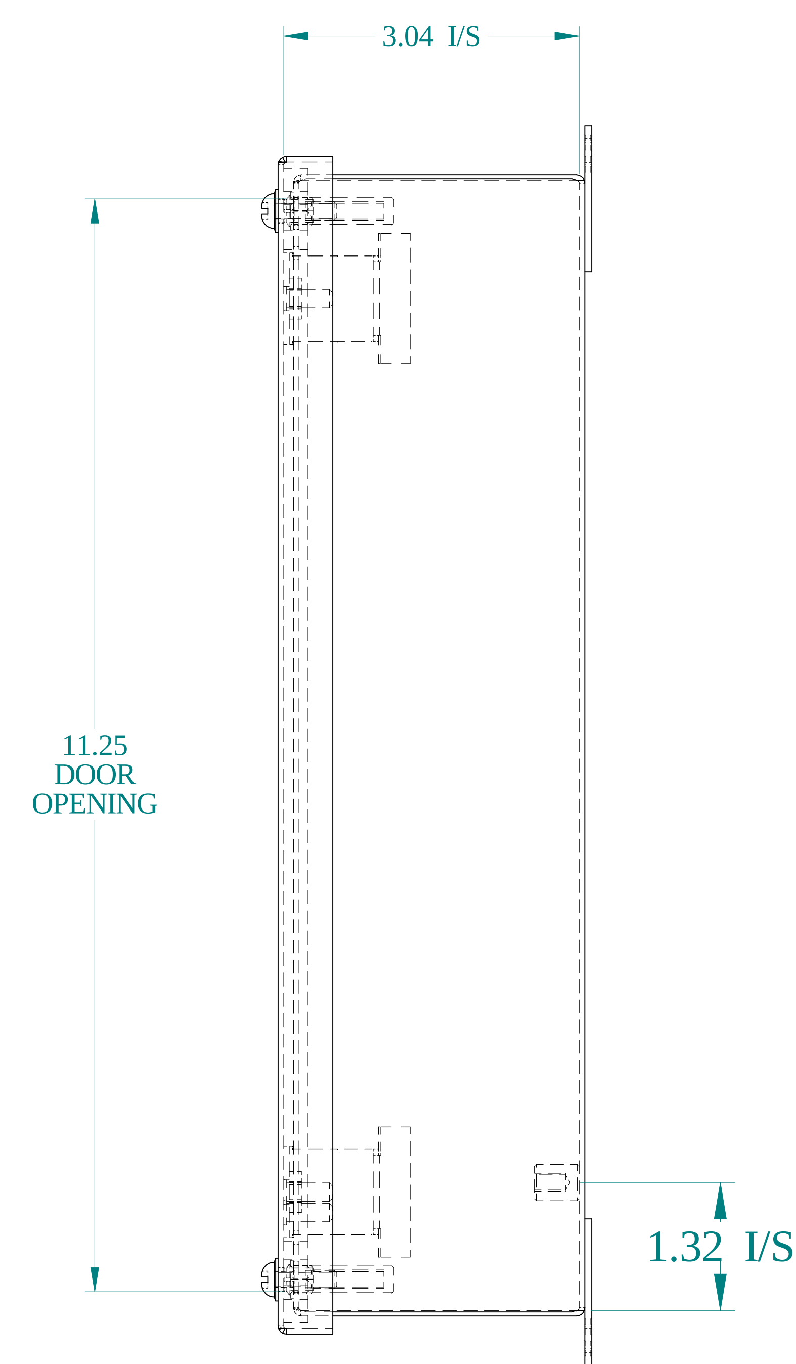
SIDE VIEW
