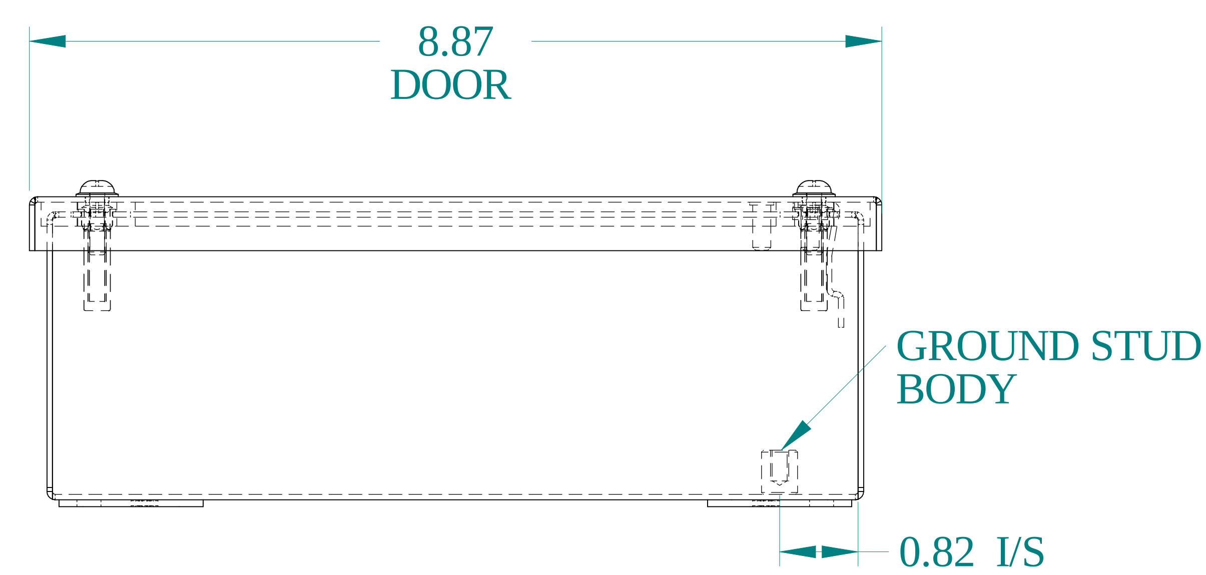
BOTTOM VIEW
