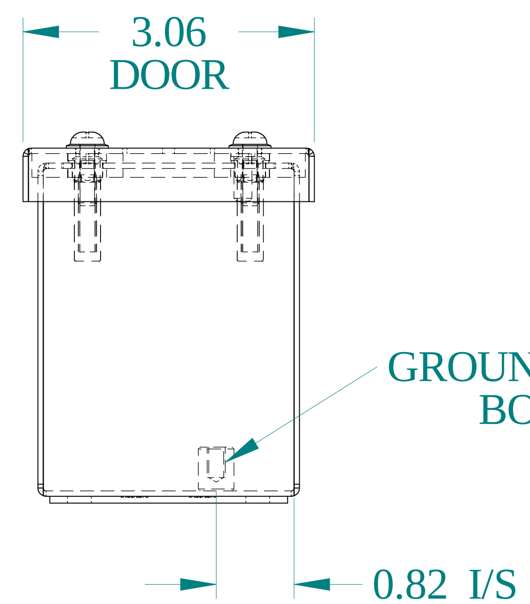
BOTTOM VIEW
