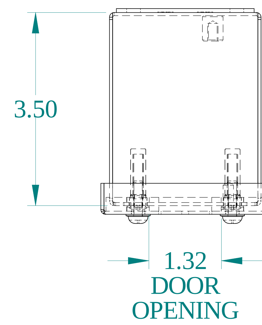
TOP VIEW
