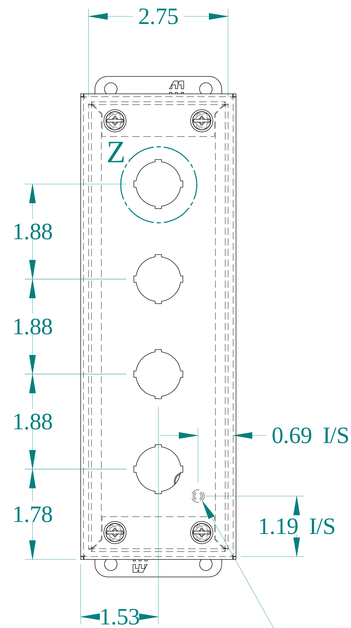
FRONT VIEW
