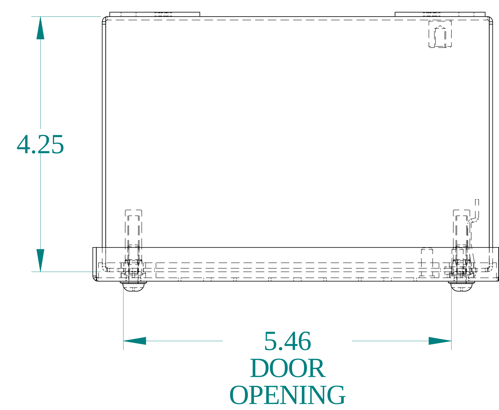
TOP VIEW
