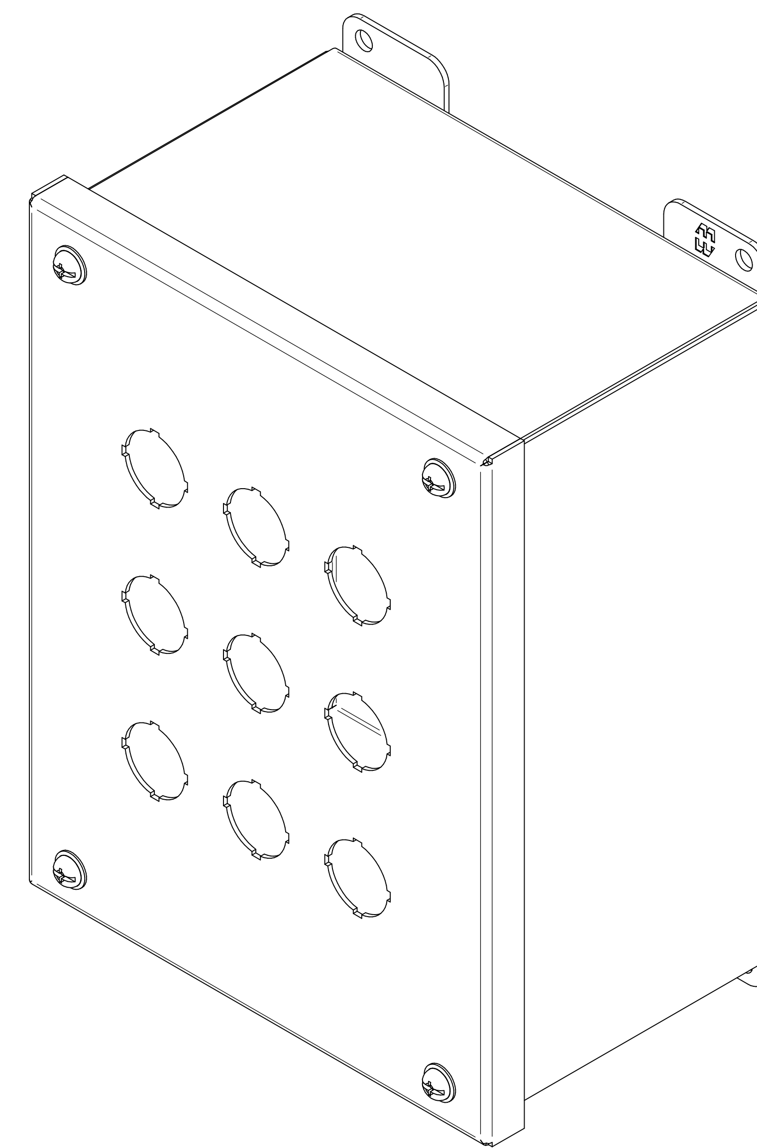
ISOMETRIC VIEWS
