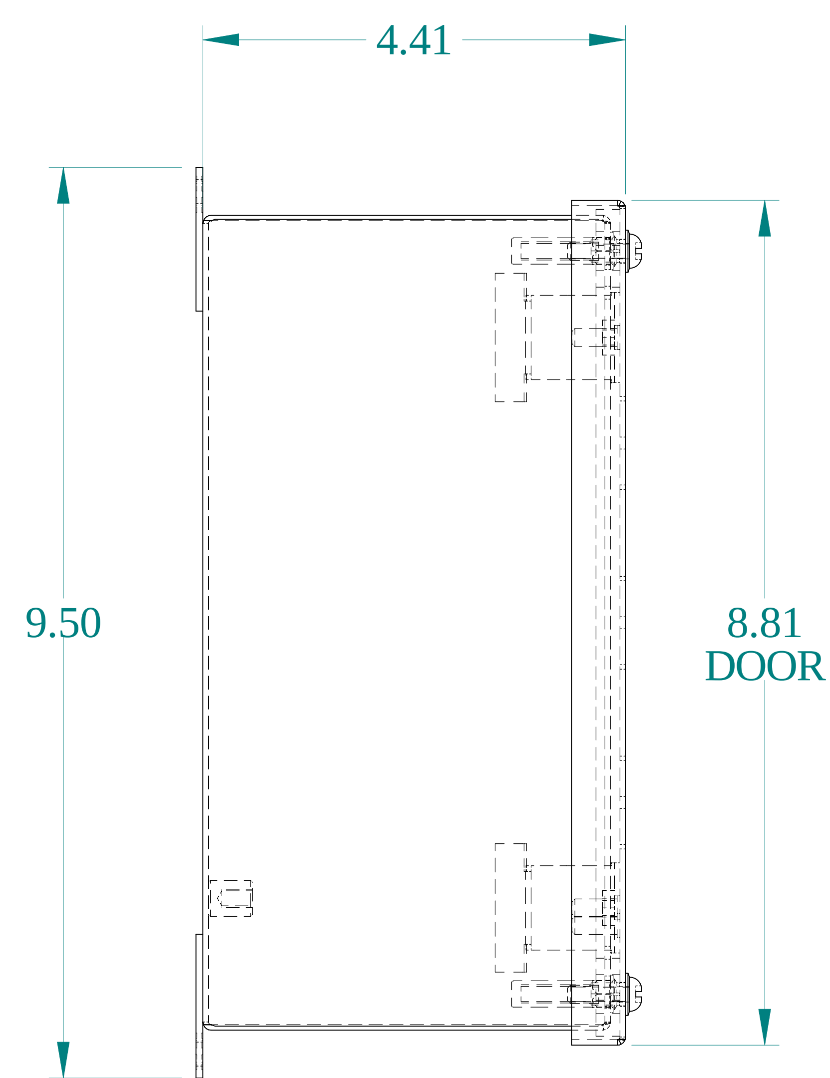
SIDE VIEW
