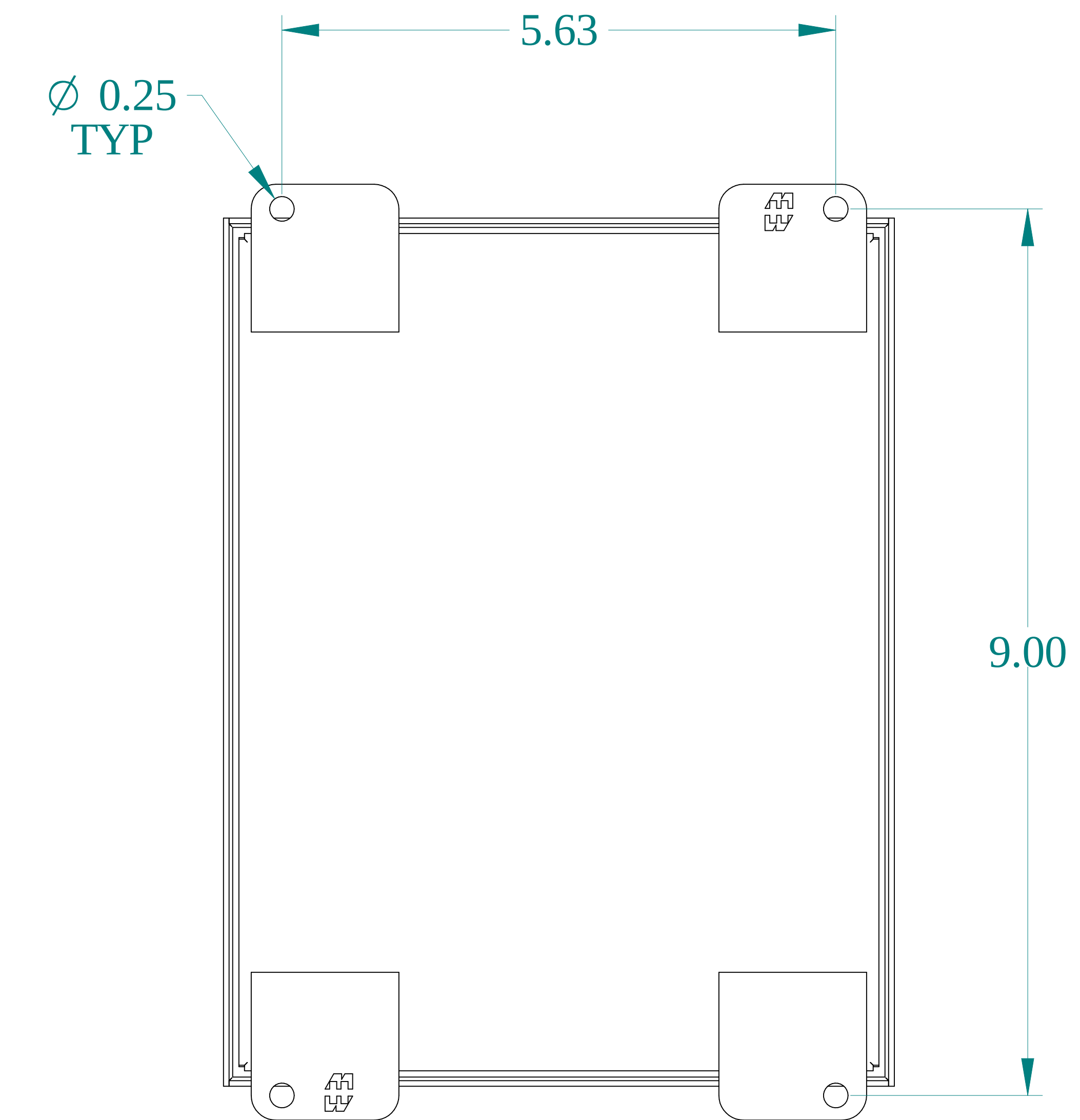
BACK VIEW
