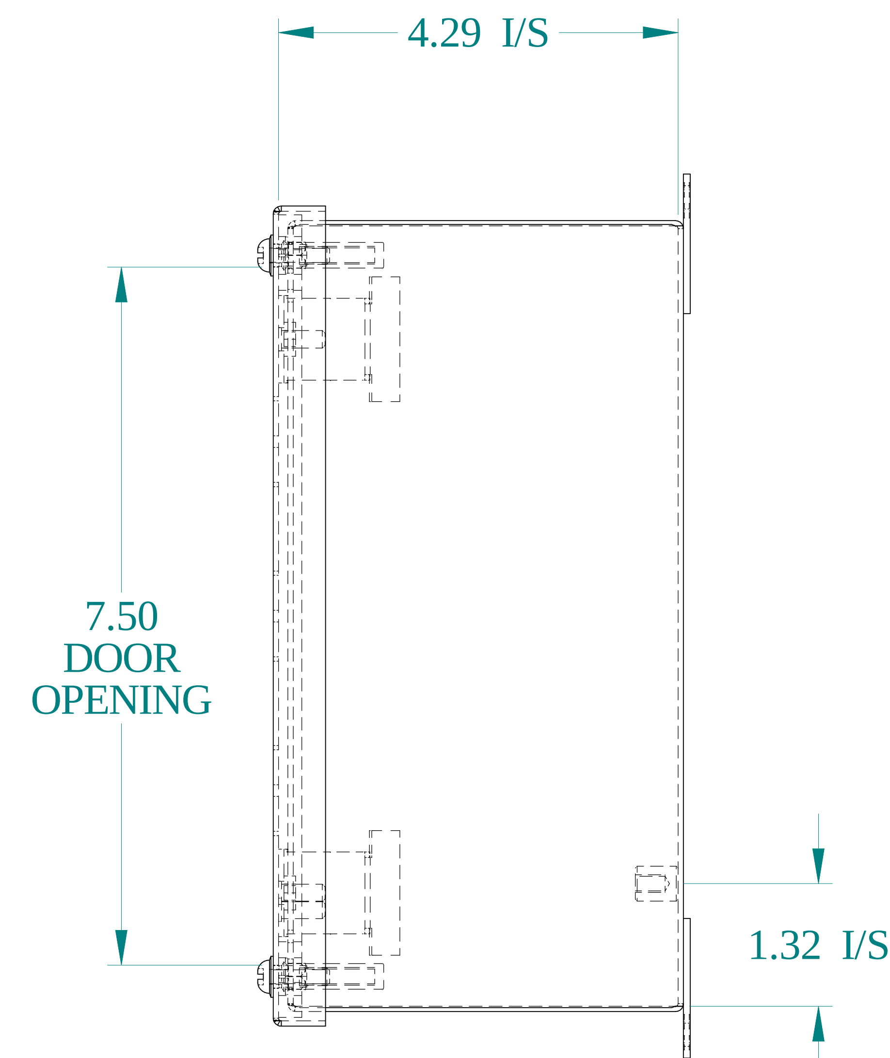
SIDE VIEW
