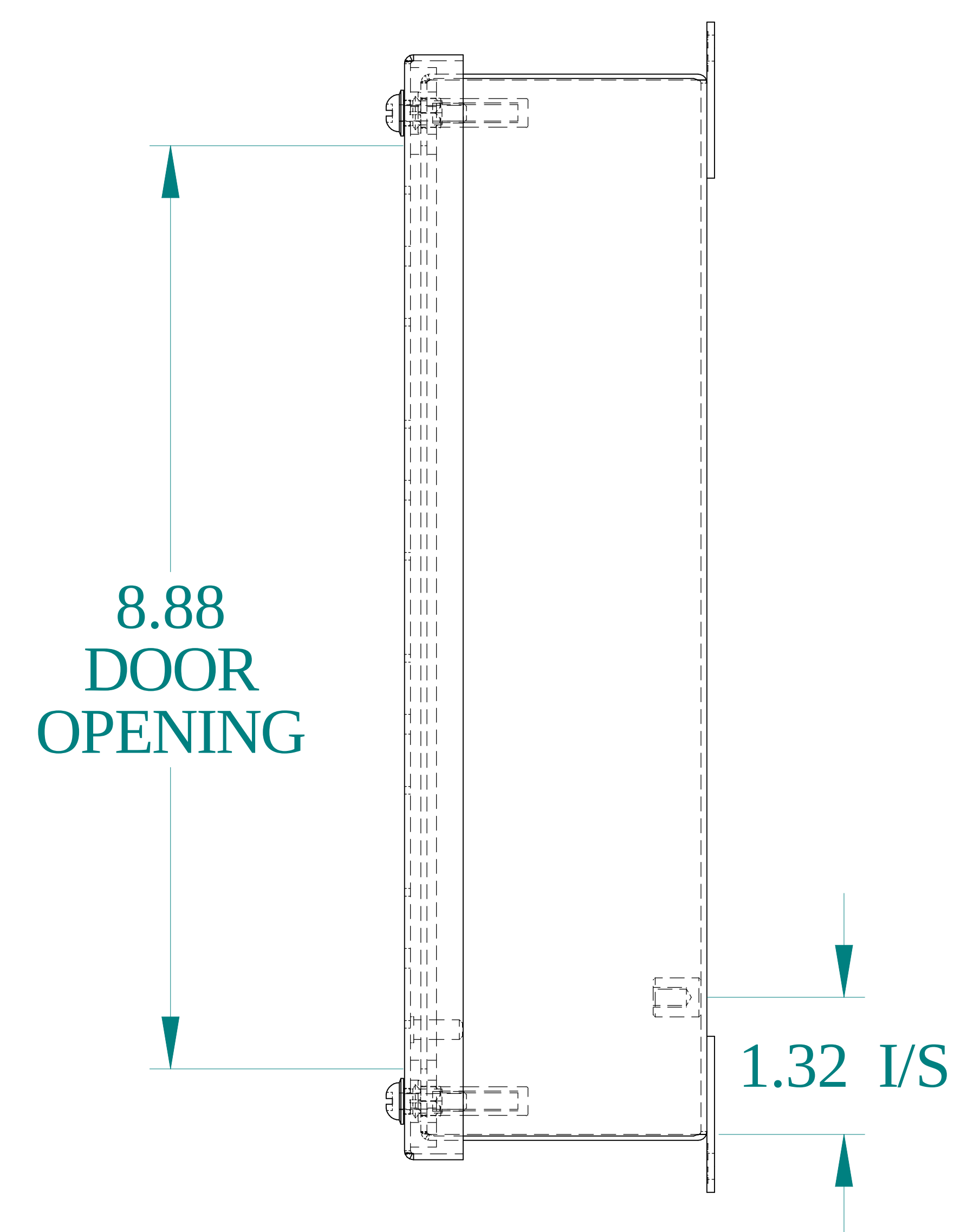
SIDE VIEW
