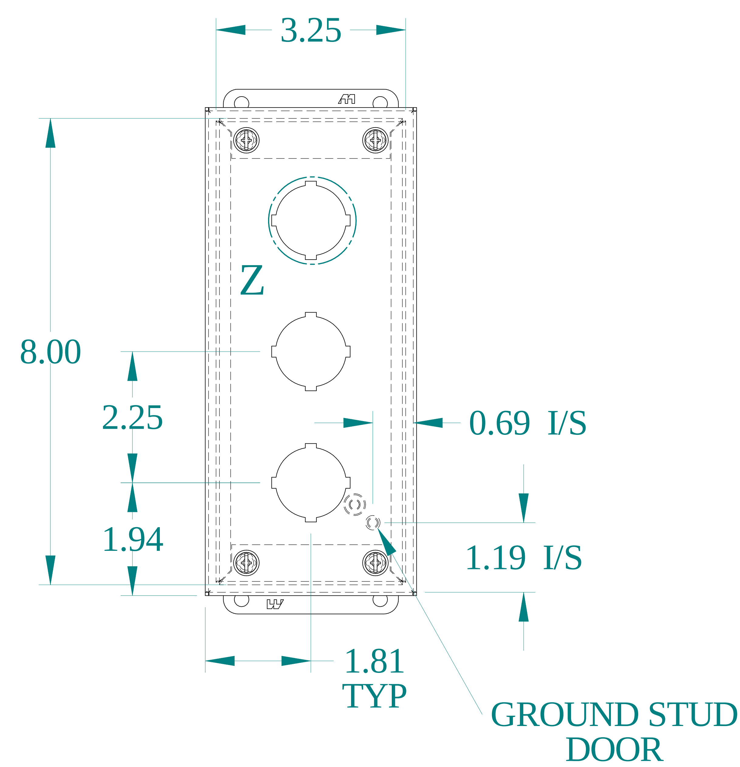
FRONT VIEW
