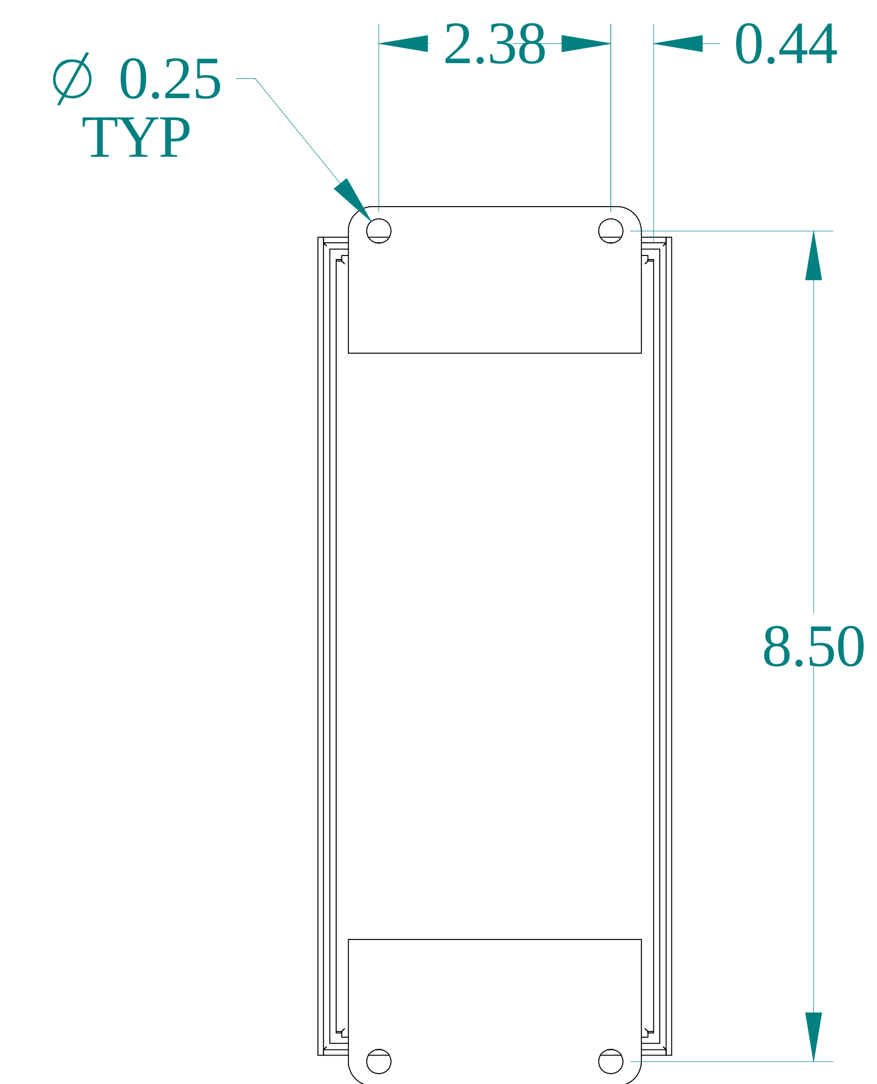
BACK VIEW
