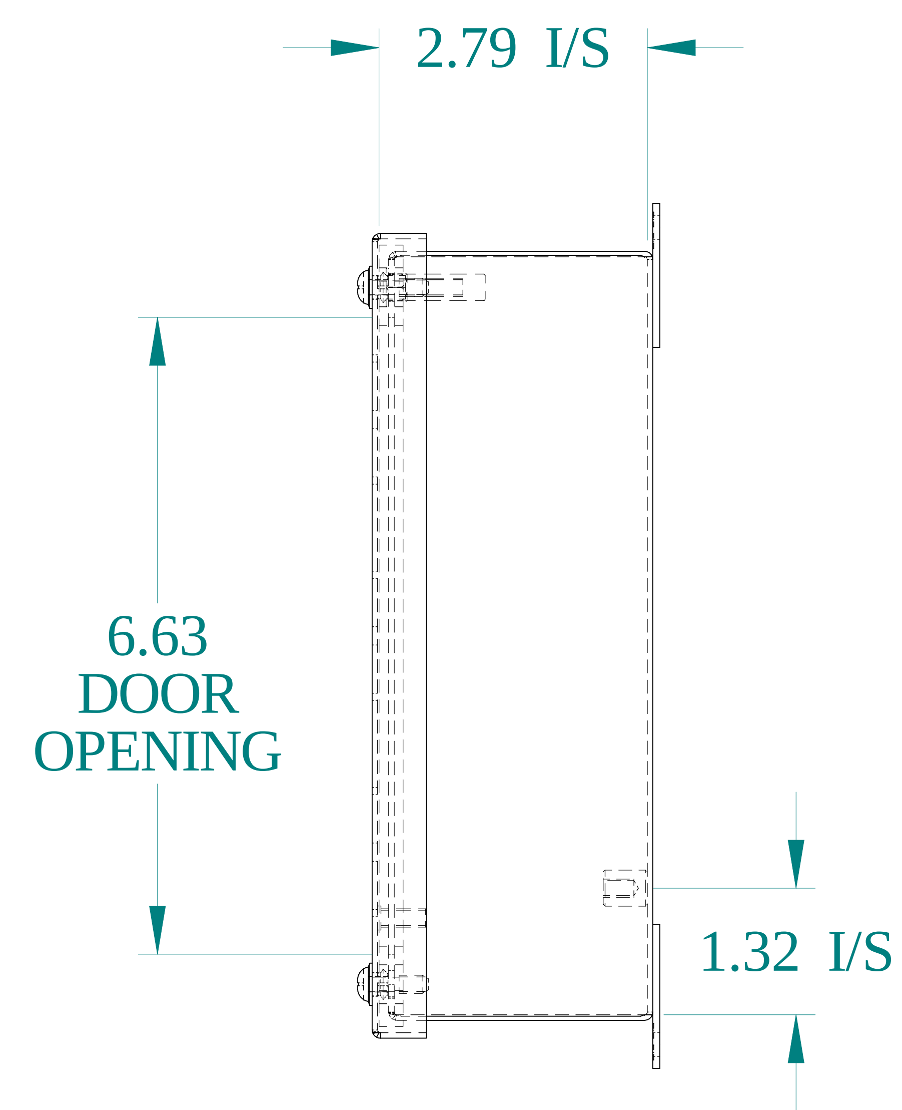
SIDE VIEW
