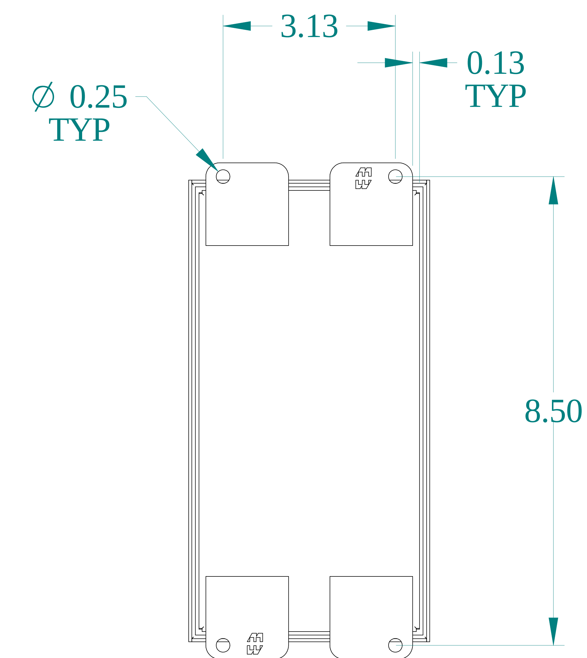
BACK VIEW
