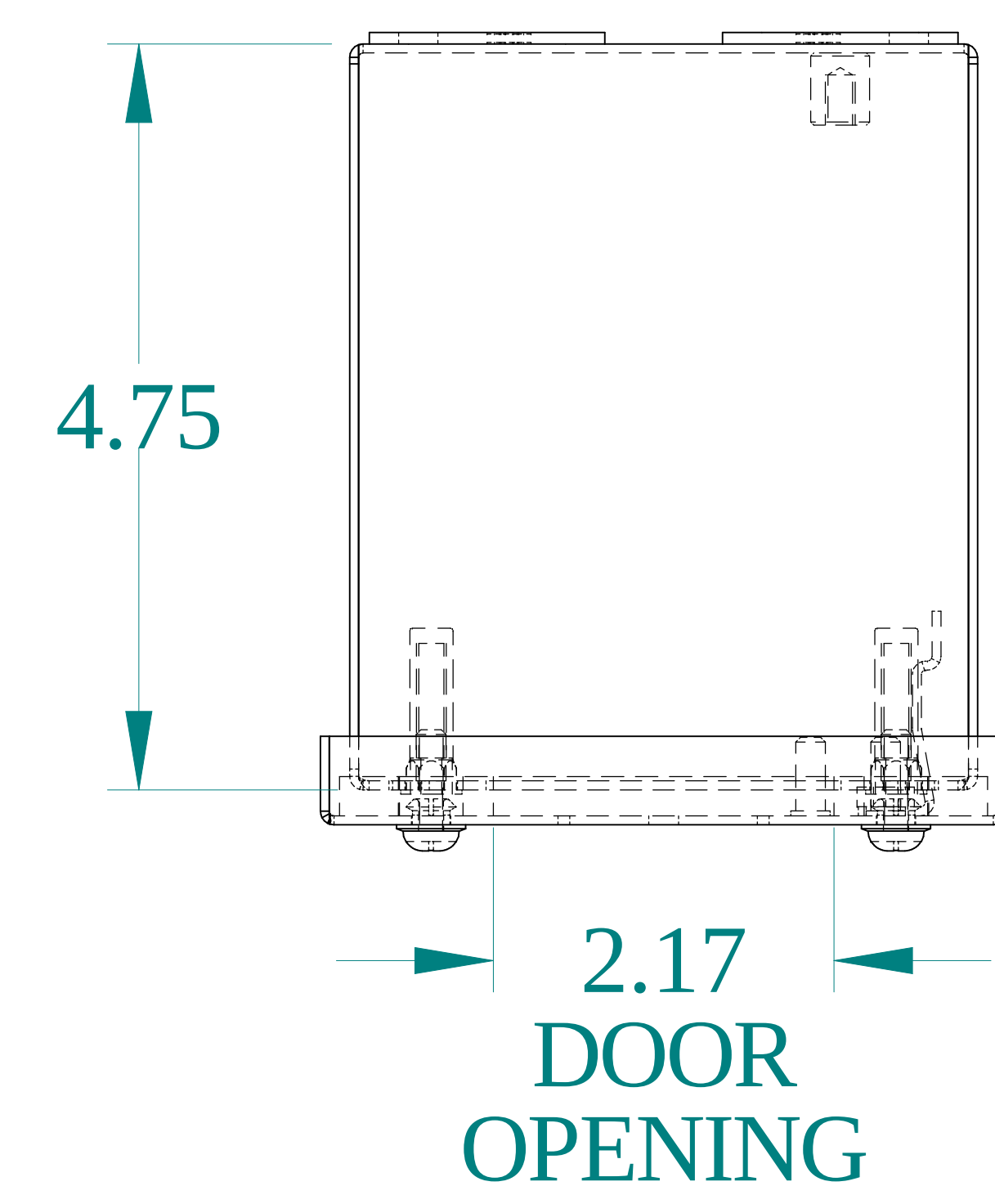
TOP VIEW
