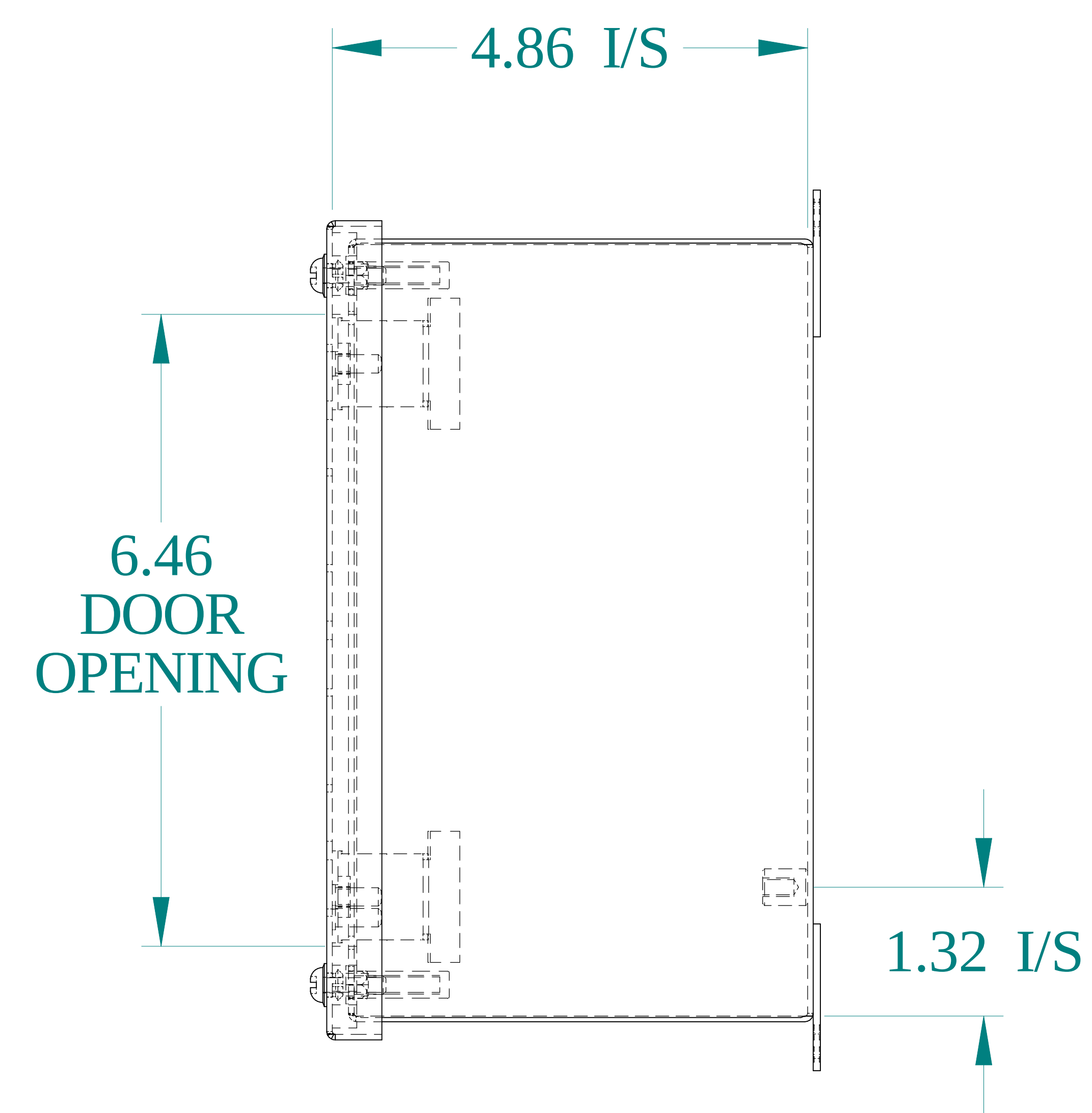
SIDE VIEW
