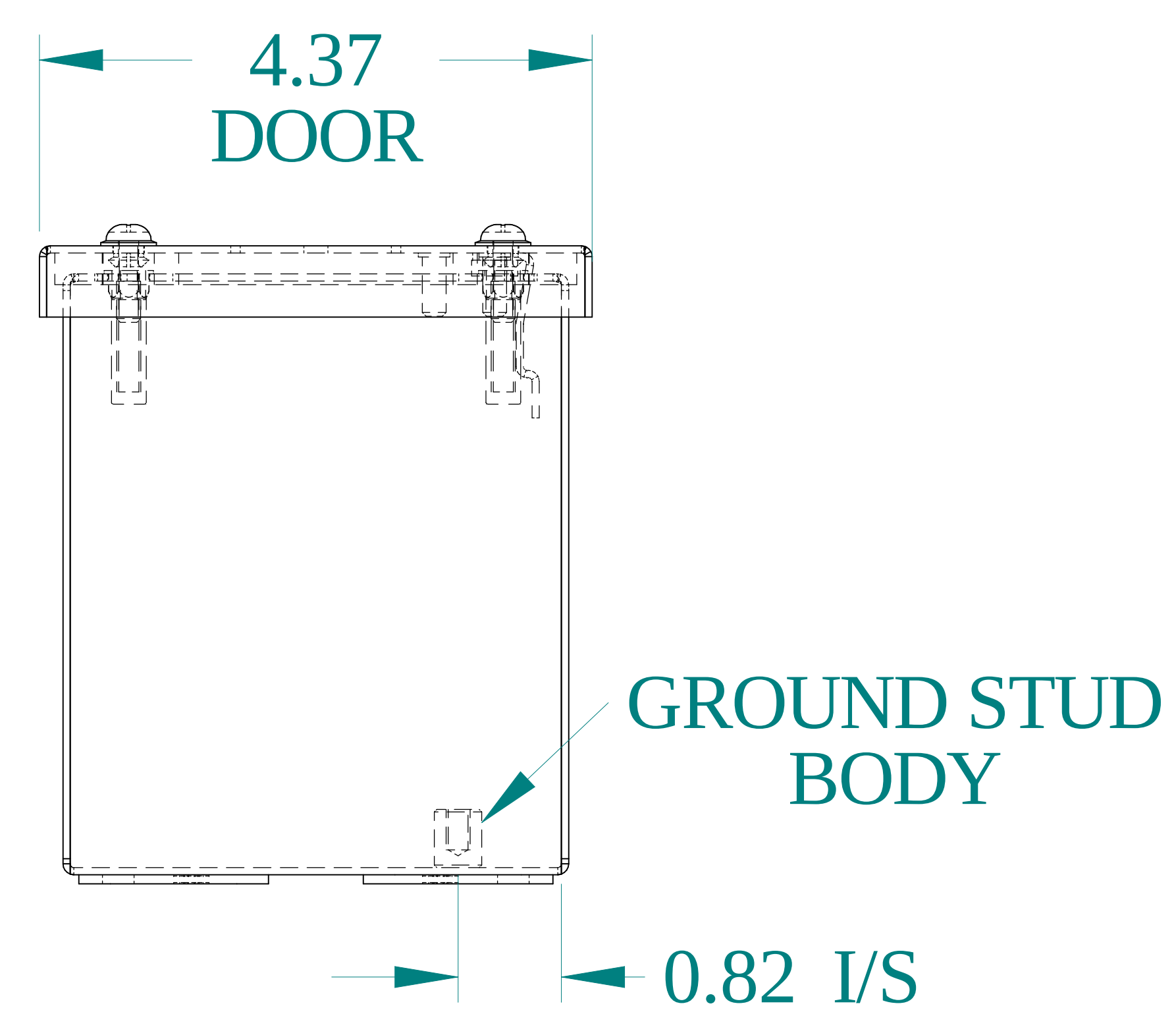
BOTTOM VIEW
