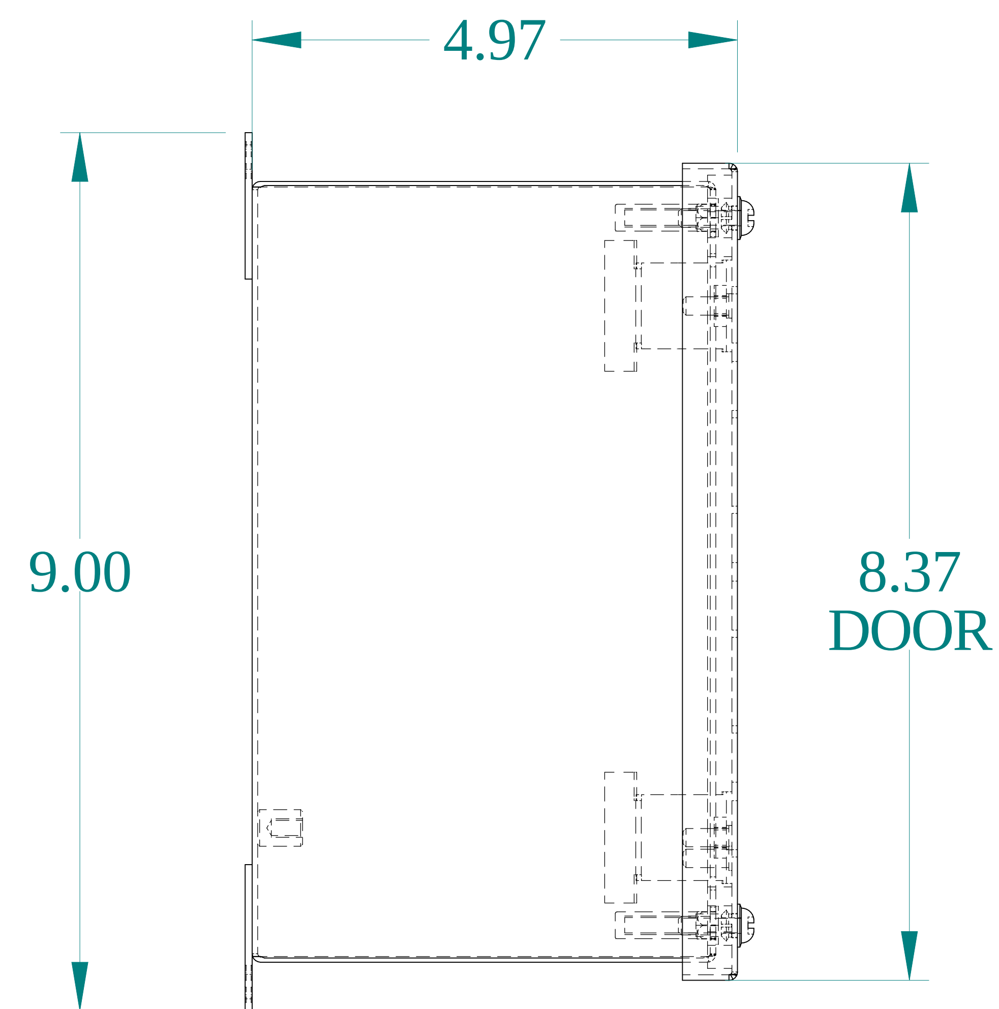
SIDE VIEW
