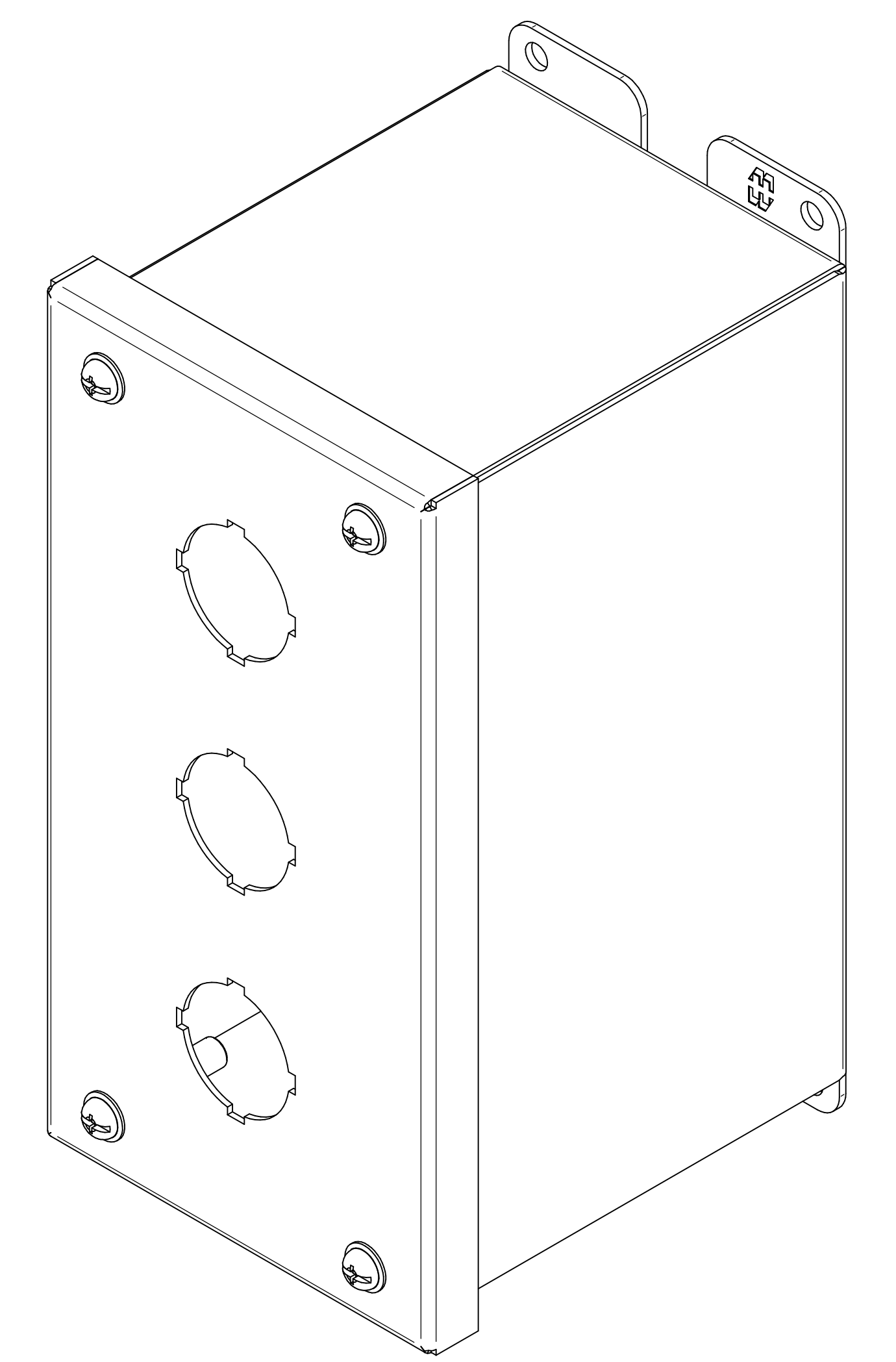
ISOMETRIC VIEWS
