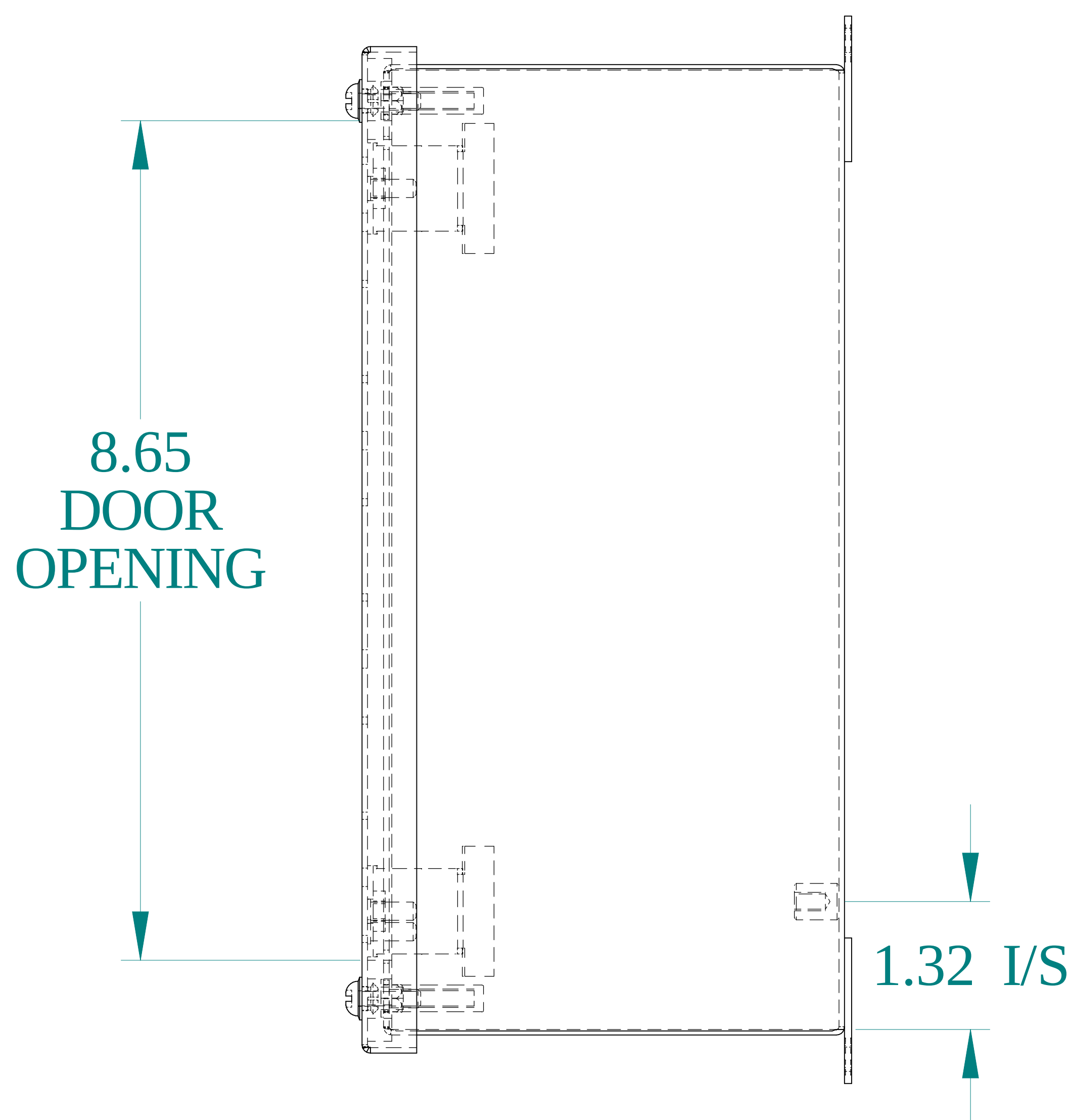
SIDE VIEW
