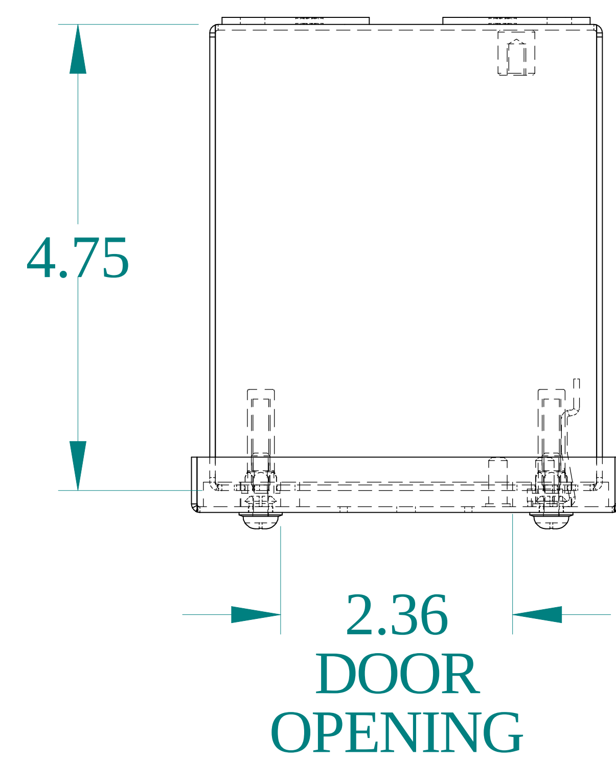
TOP VIEW
