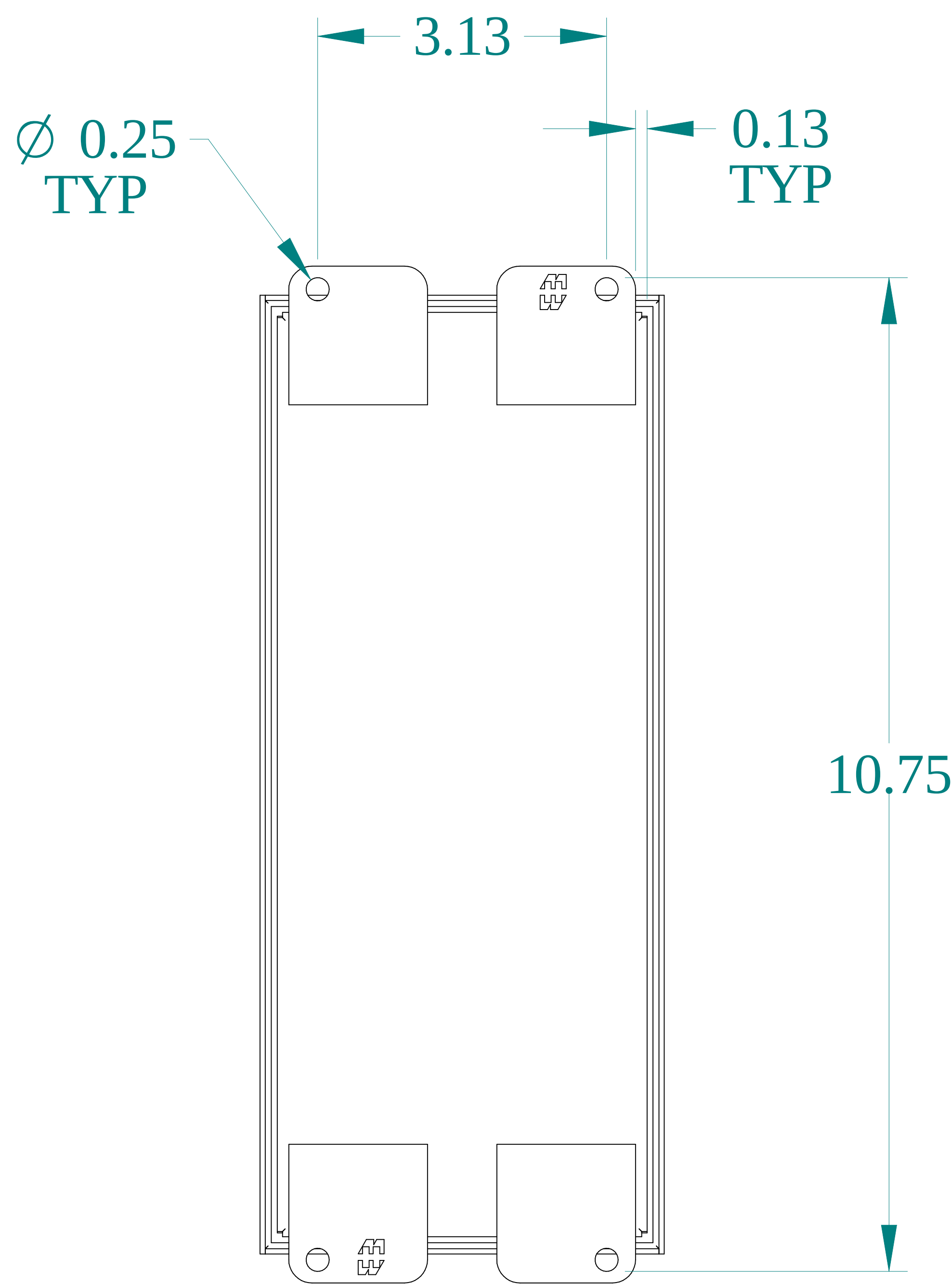
BACK VIEW
