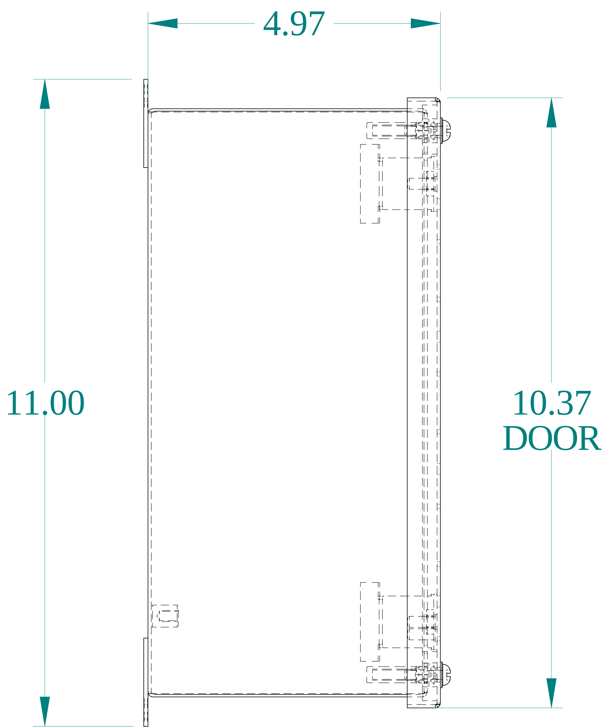
SIDE VIEW
