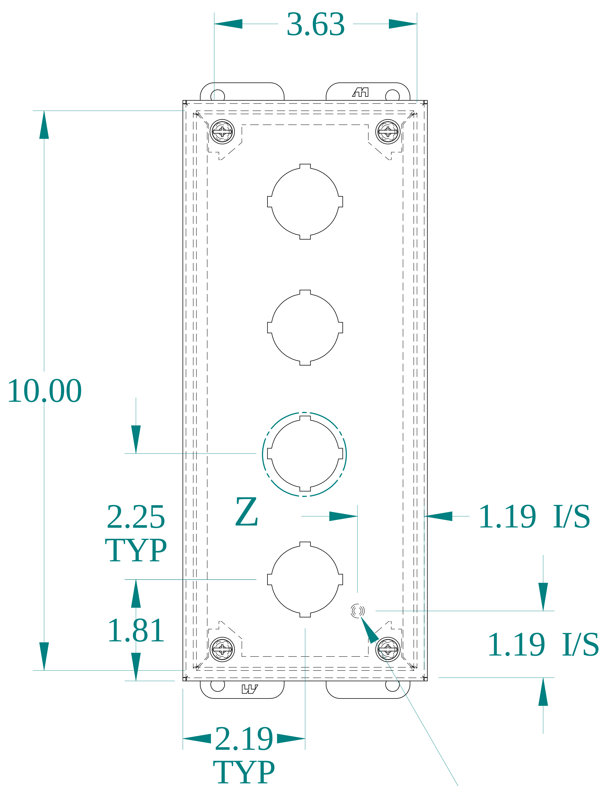
FRONT VIEW
