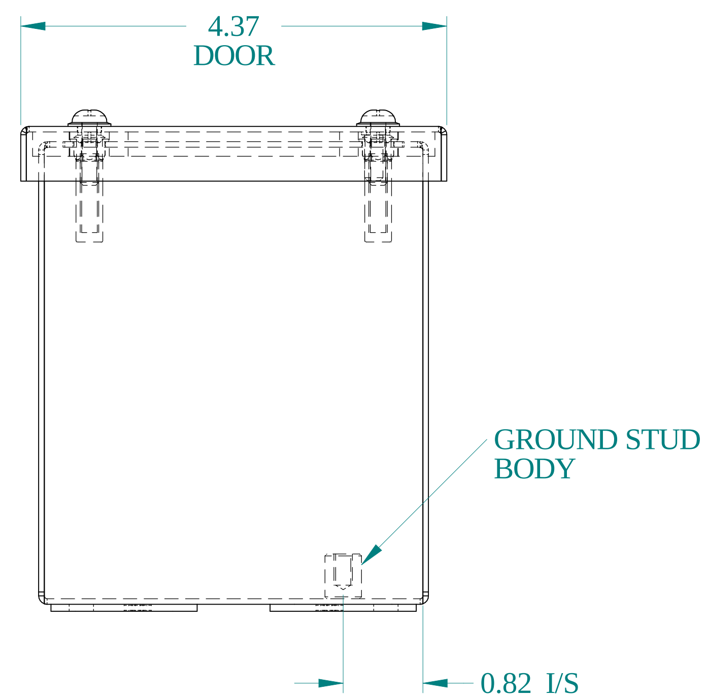
BOTTOM VIEW
