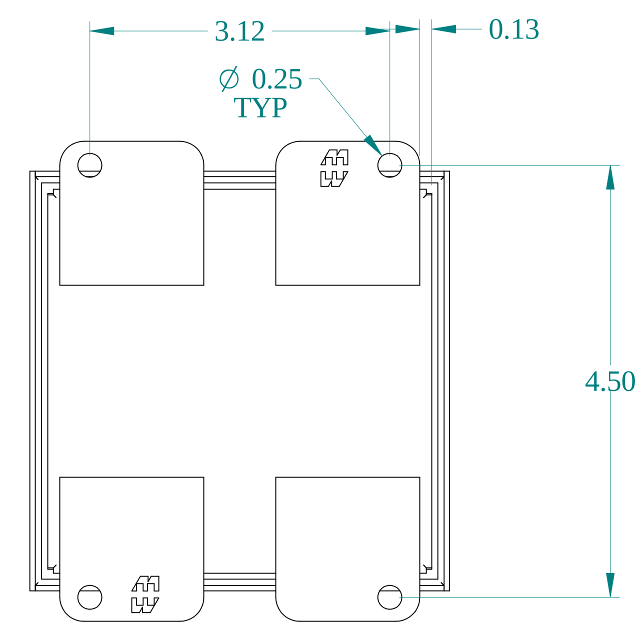
BACK VIEW
