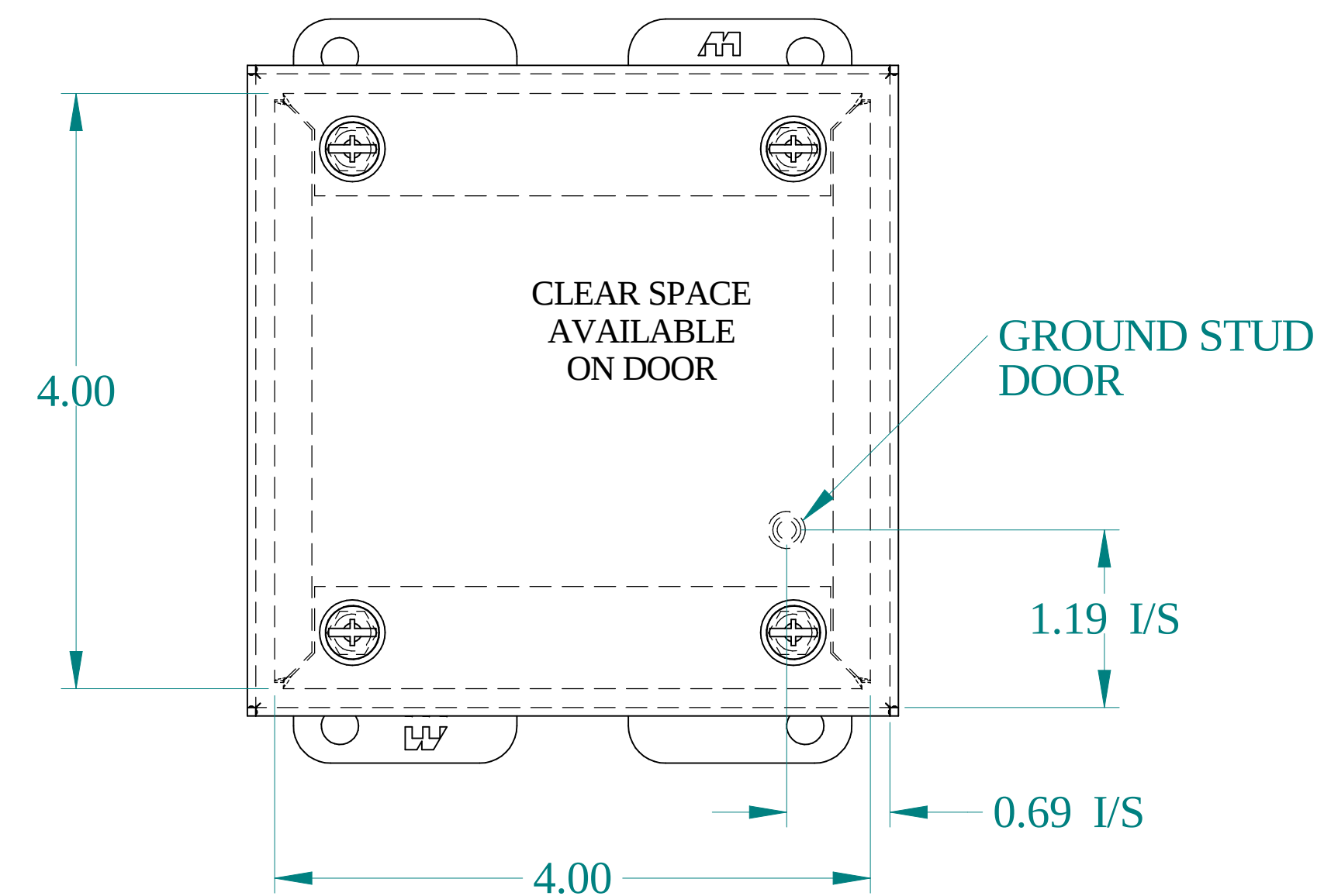
FRONT VIEW
