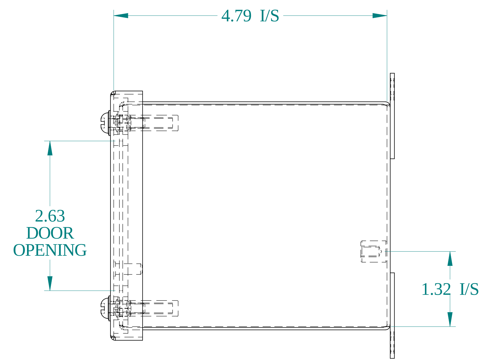
SIDE VIEW
