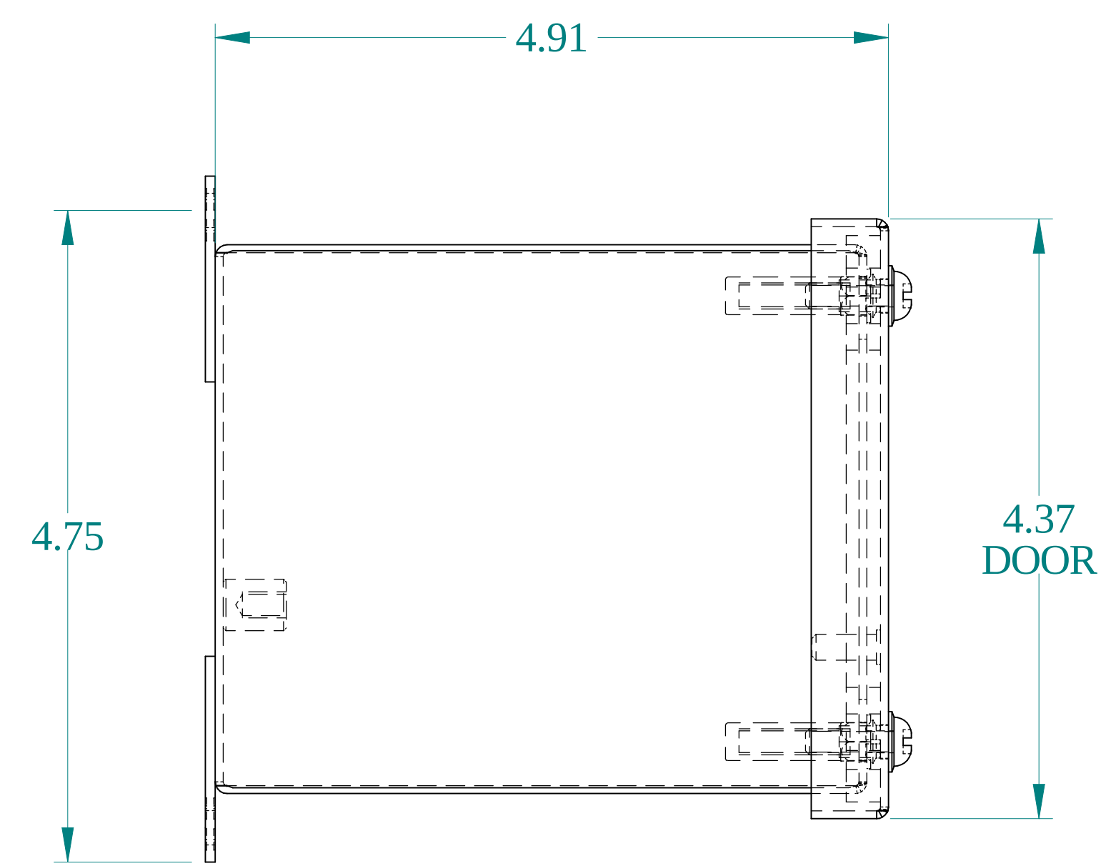
SIDE VIEW
