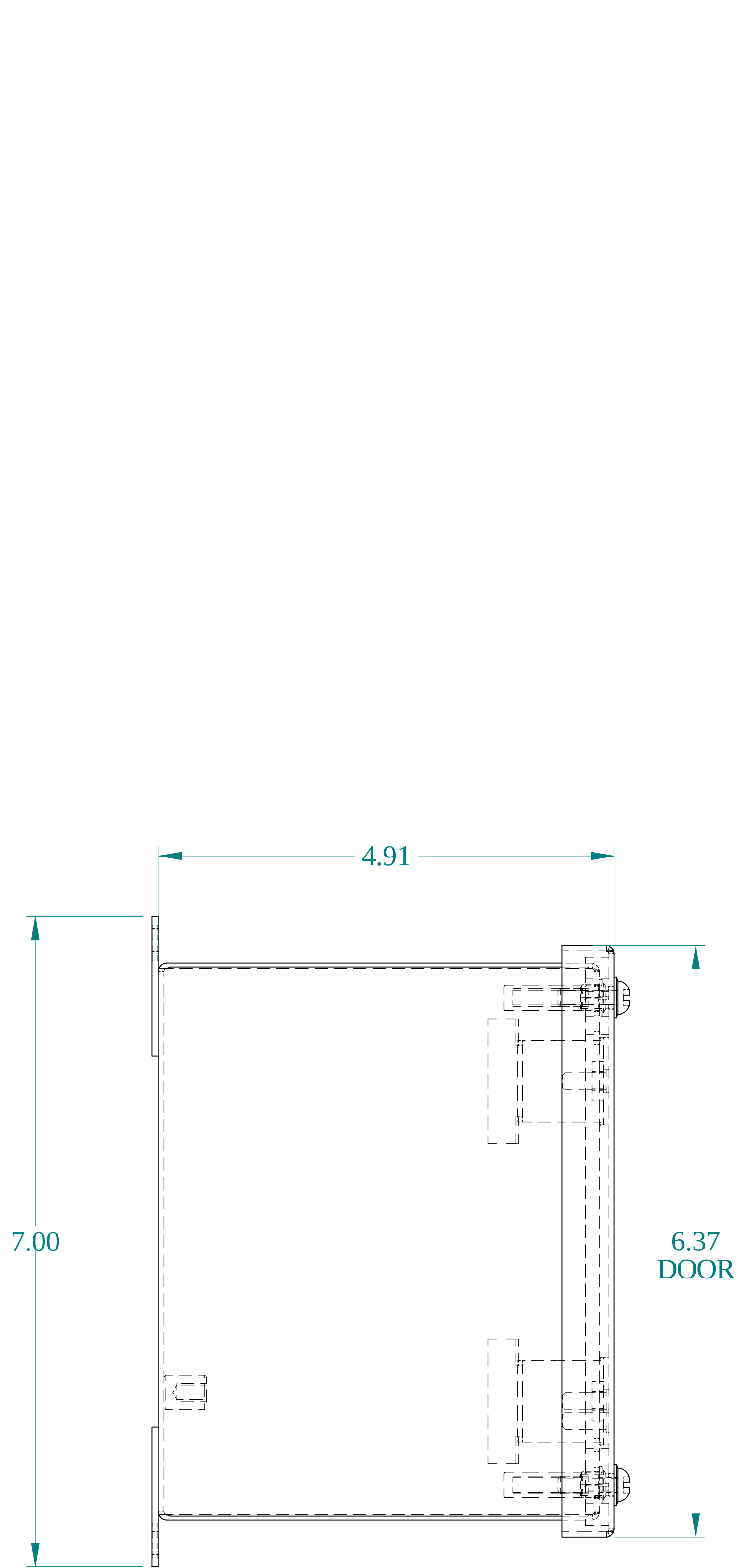
SIDE VIEW
