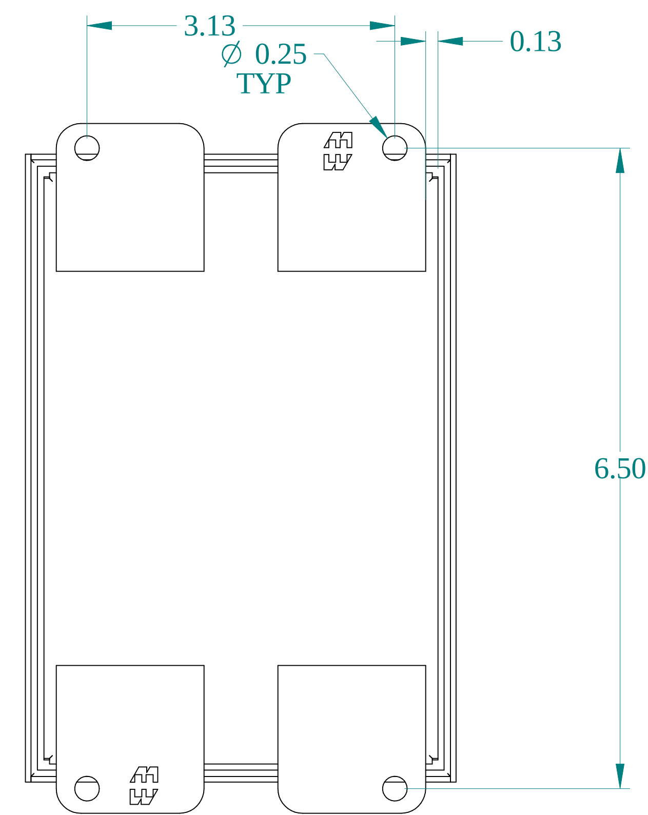
BACK VIEW
