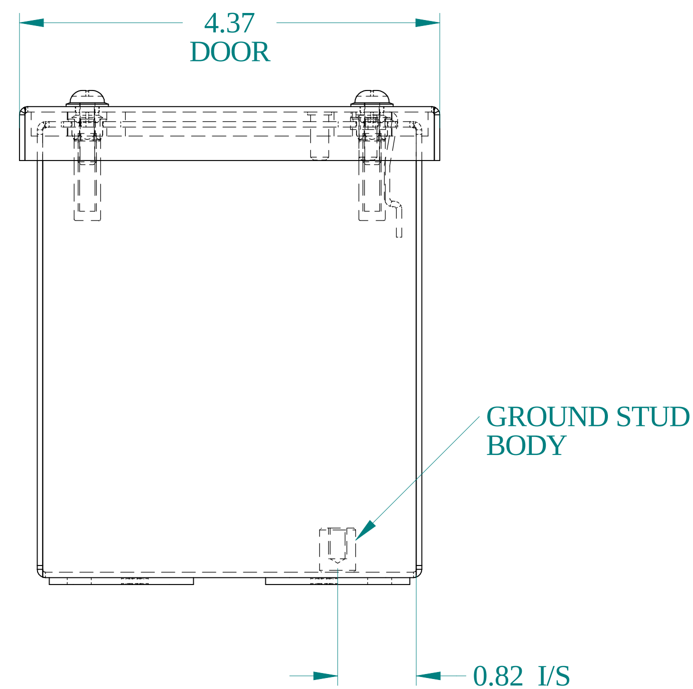
BOTTOM VIEW
