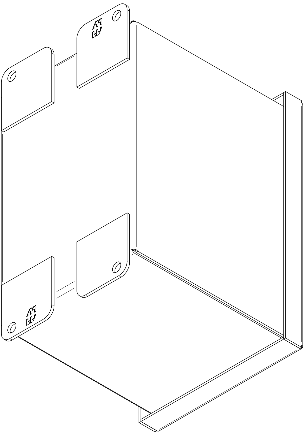
ISOMETRIC VIEWS
