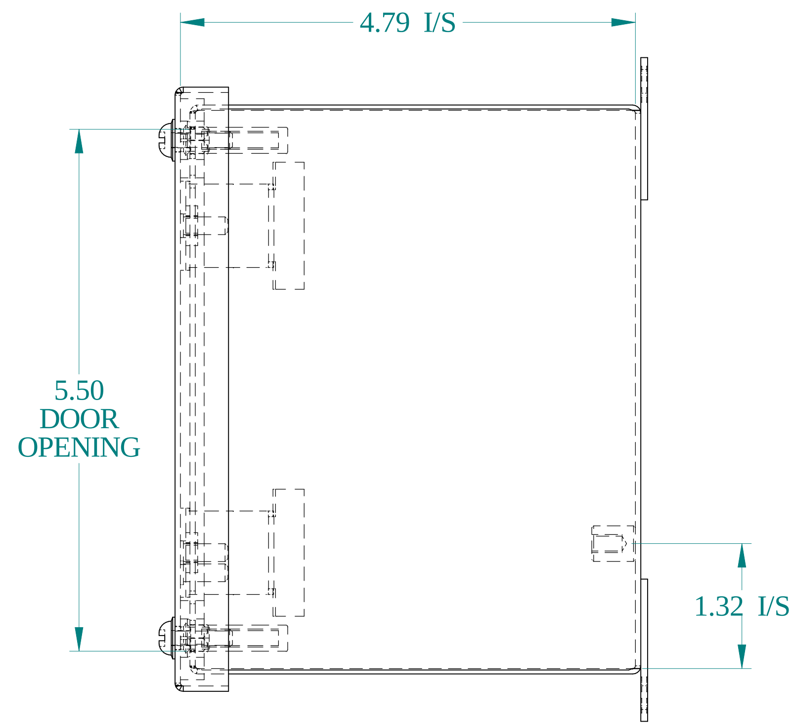
SIDE VIEW
