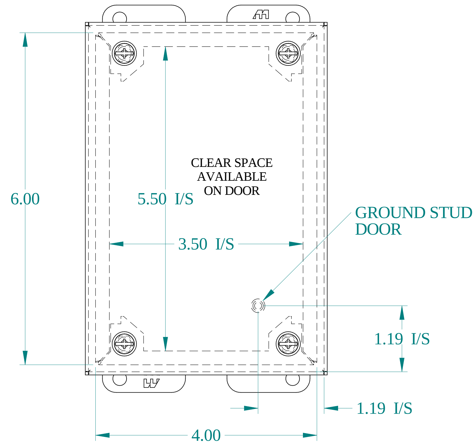
FRONT VIEW
