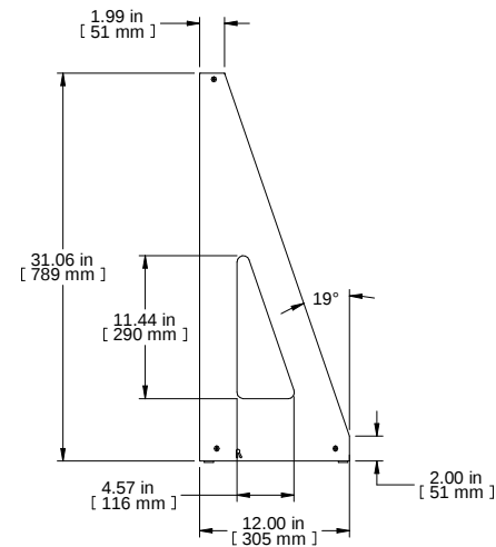
R.S. VIEW
