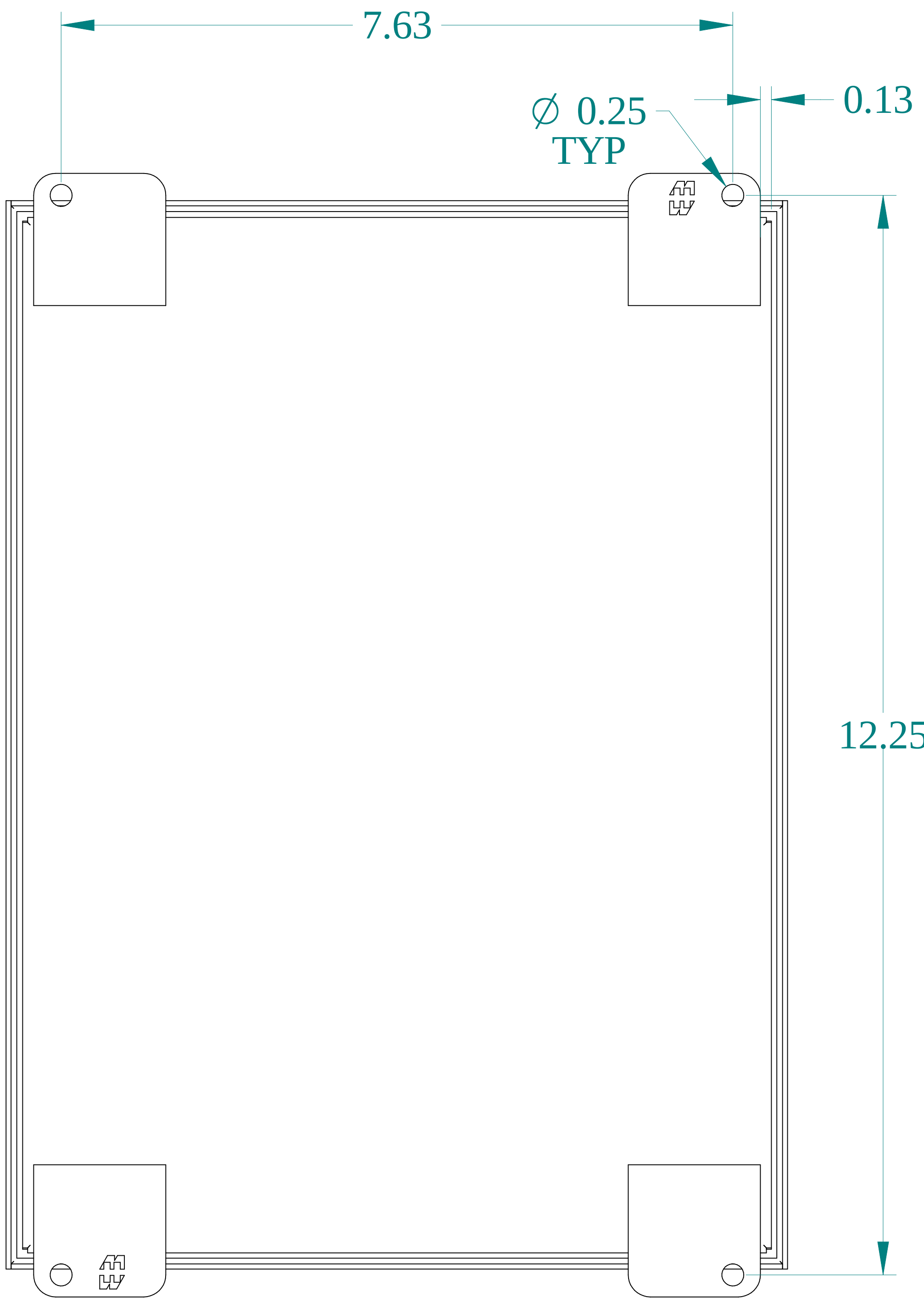
BACK VIEW
