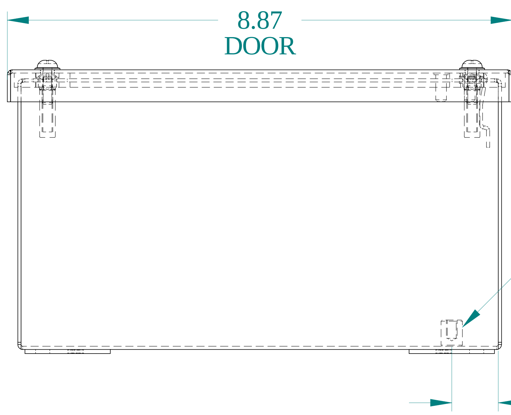
BOTTOM VIEW
