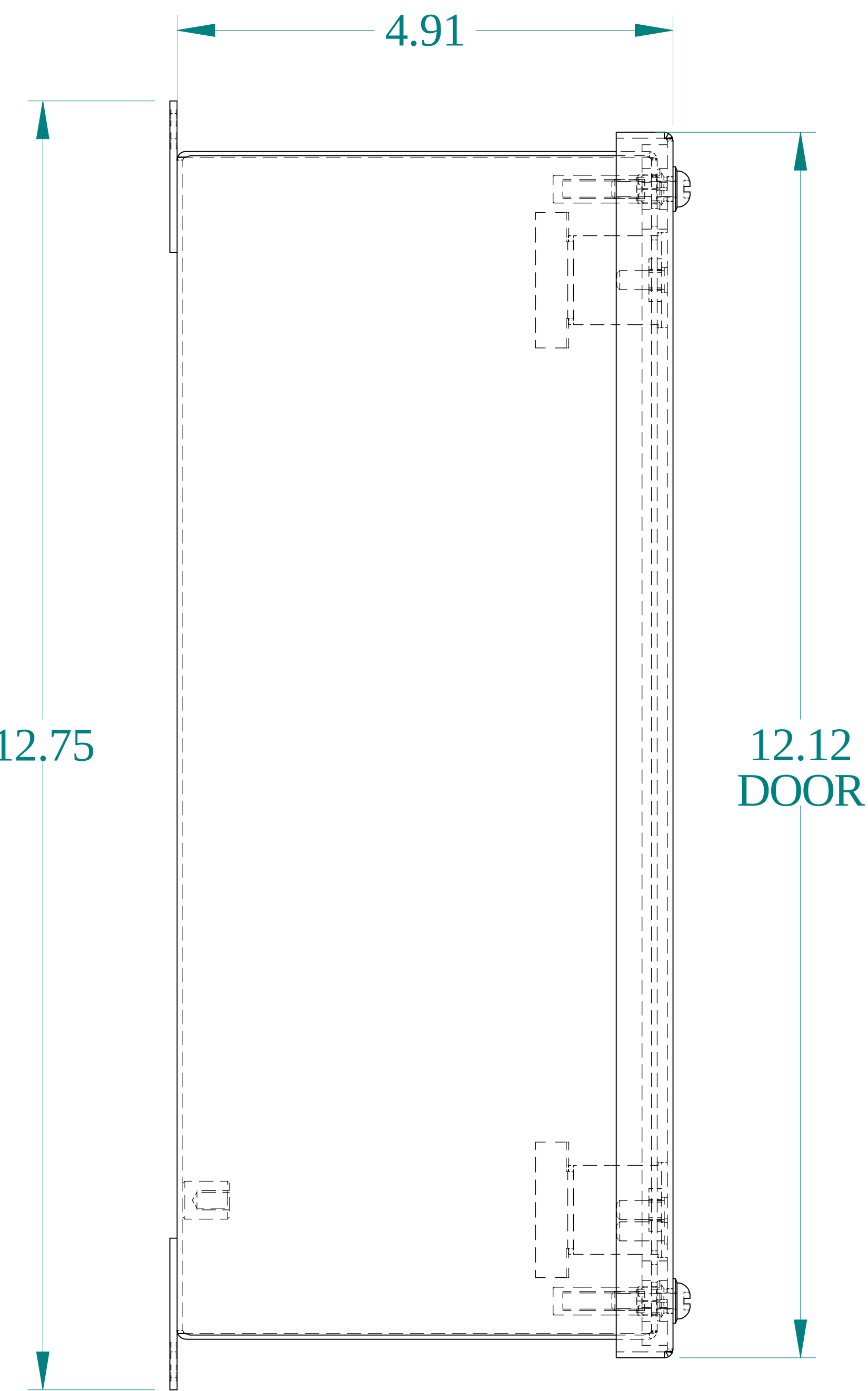
SIDE VIEW
