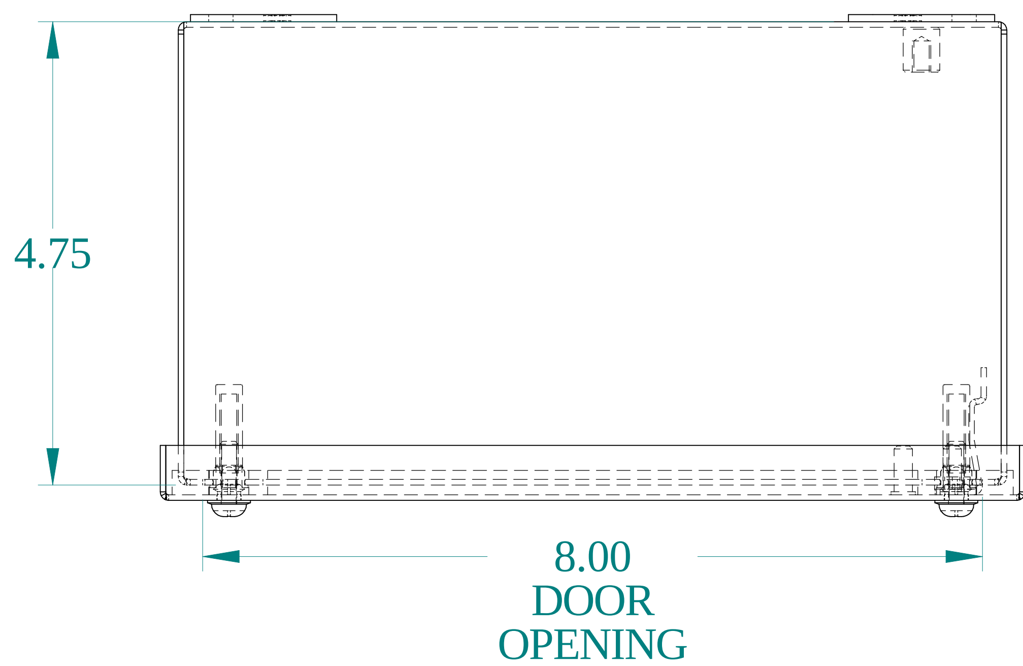
TOP VIEW
