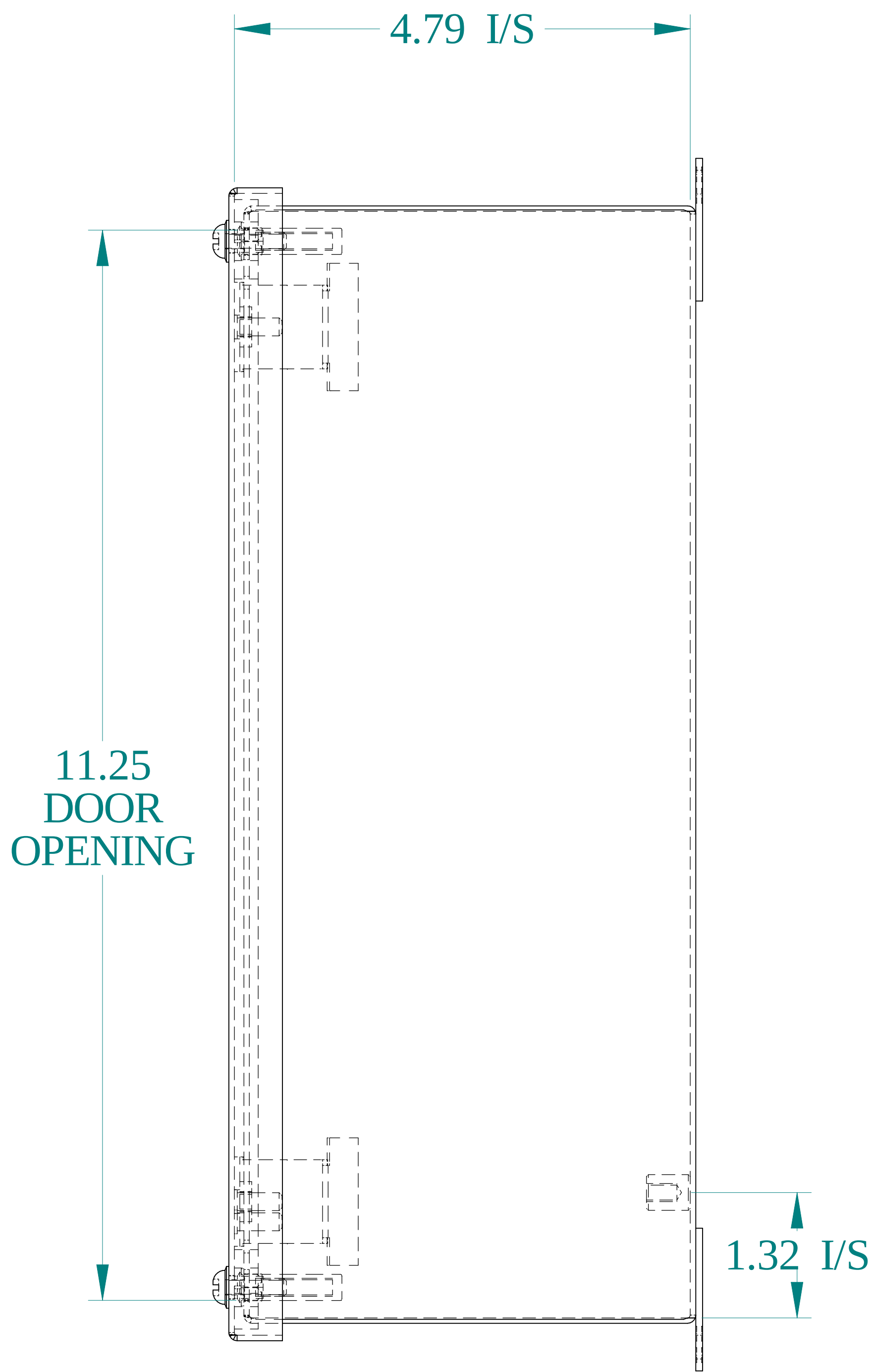
SIDE VIEW
