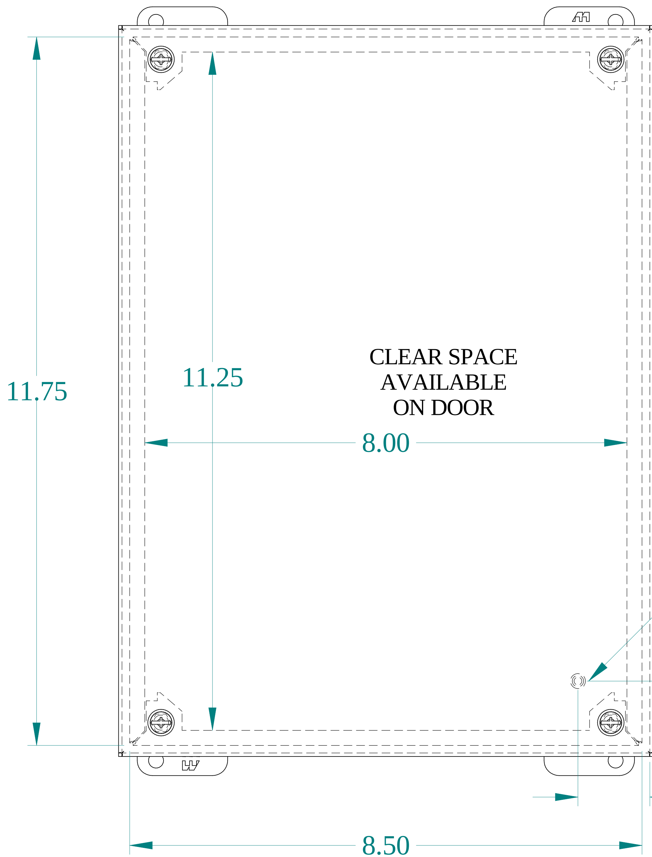
FRONT VIEW
