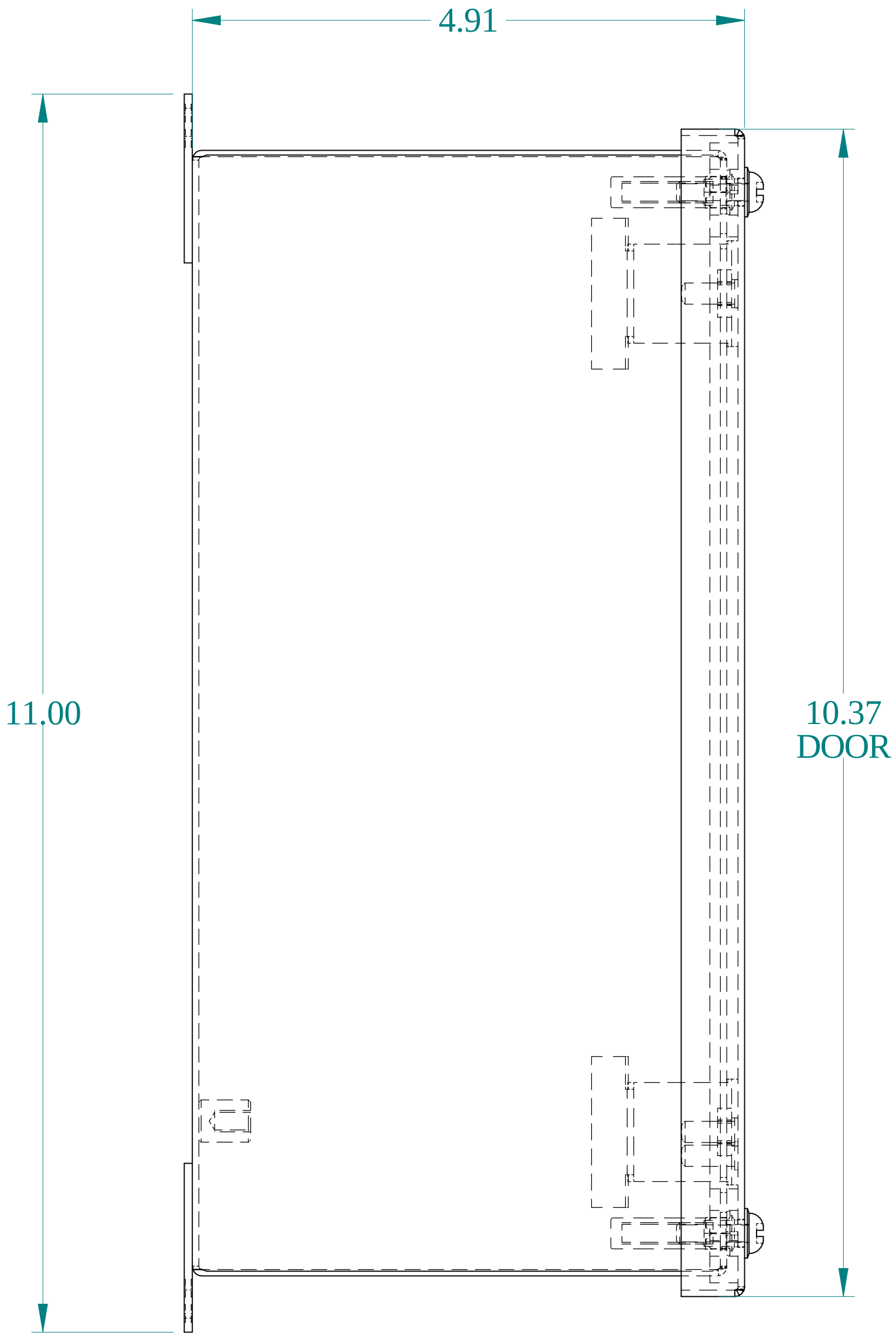
SIDE VIEW
