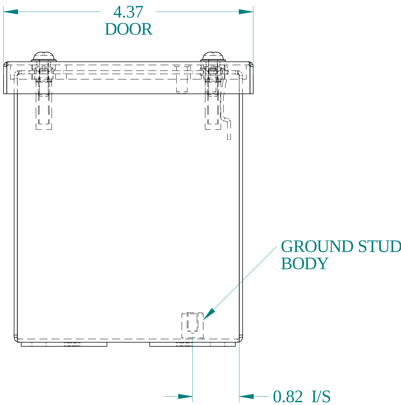
BOTTOM VIEW
