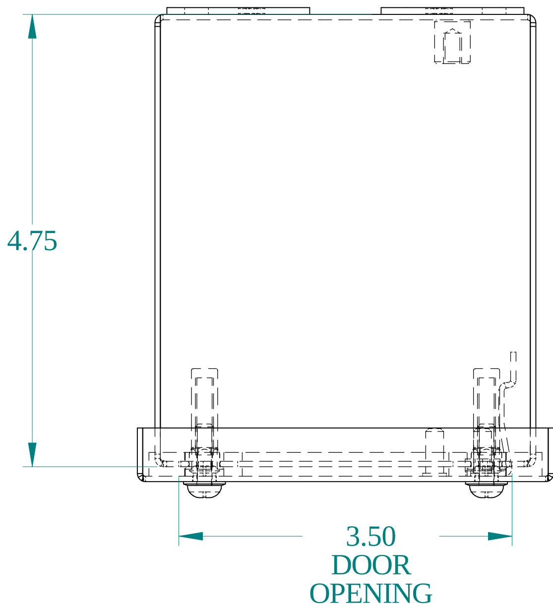
TOP VIEW
