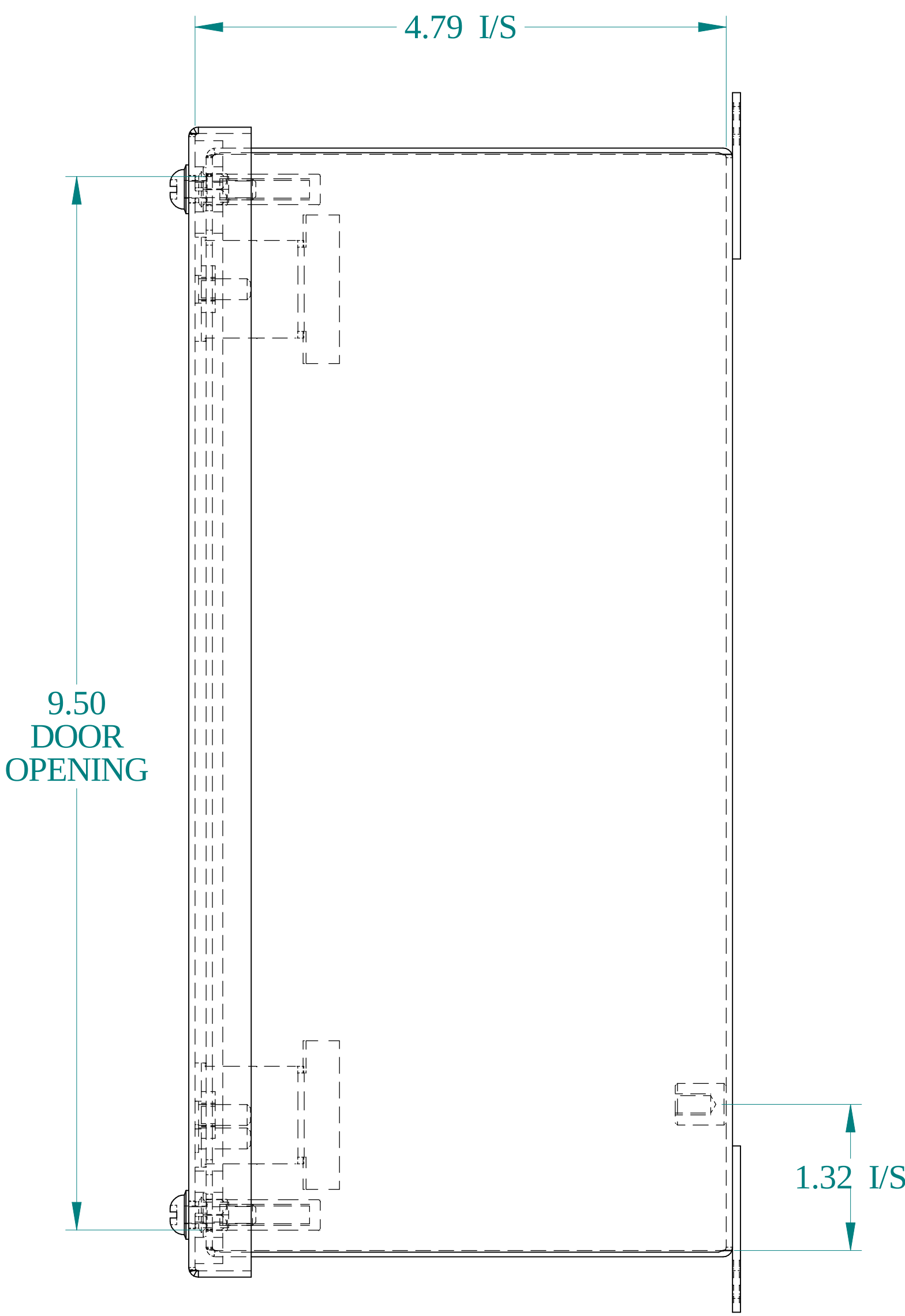
SIDE VIEW
