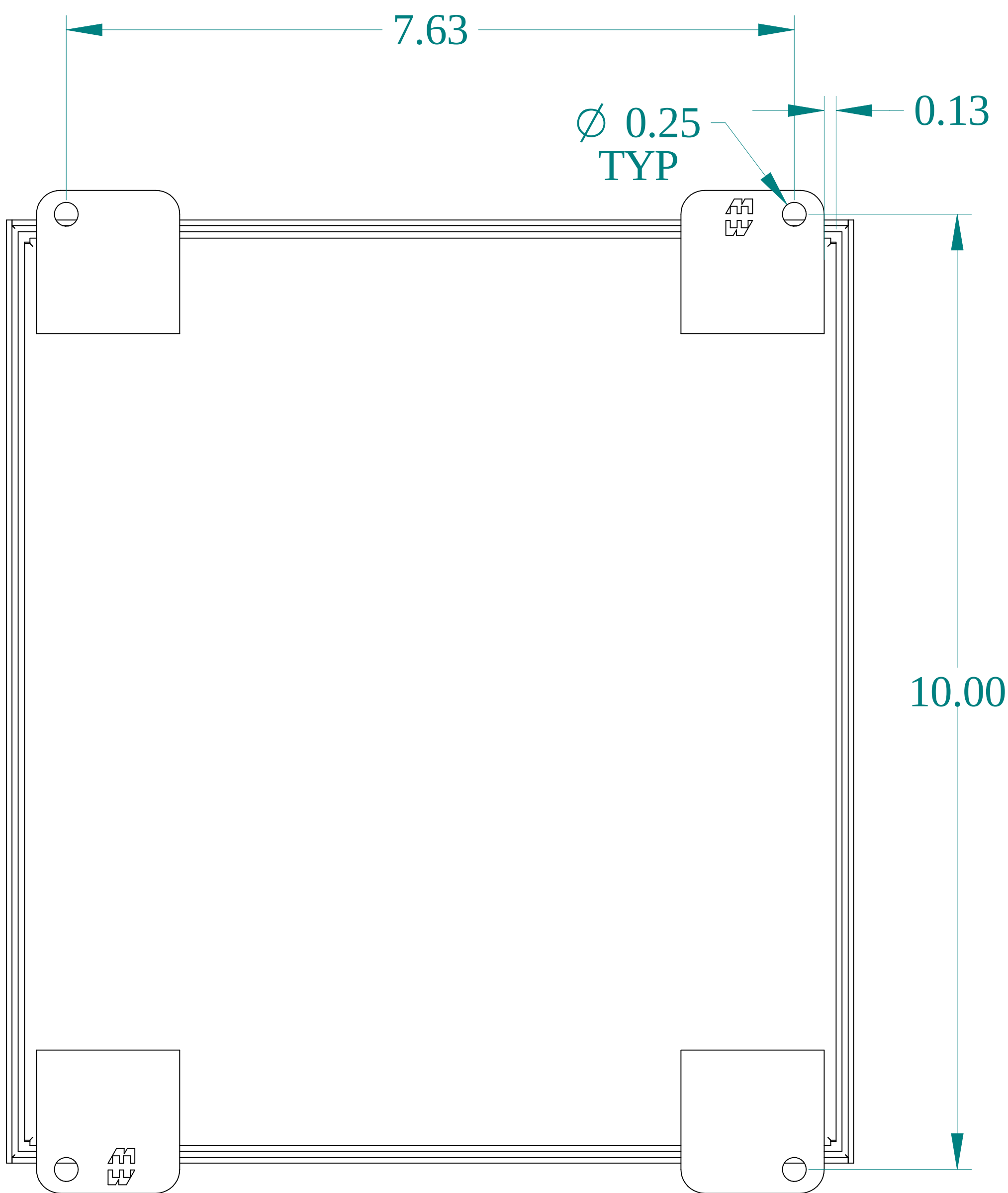
BACK VIEW
