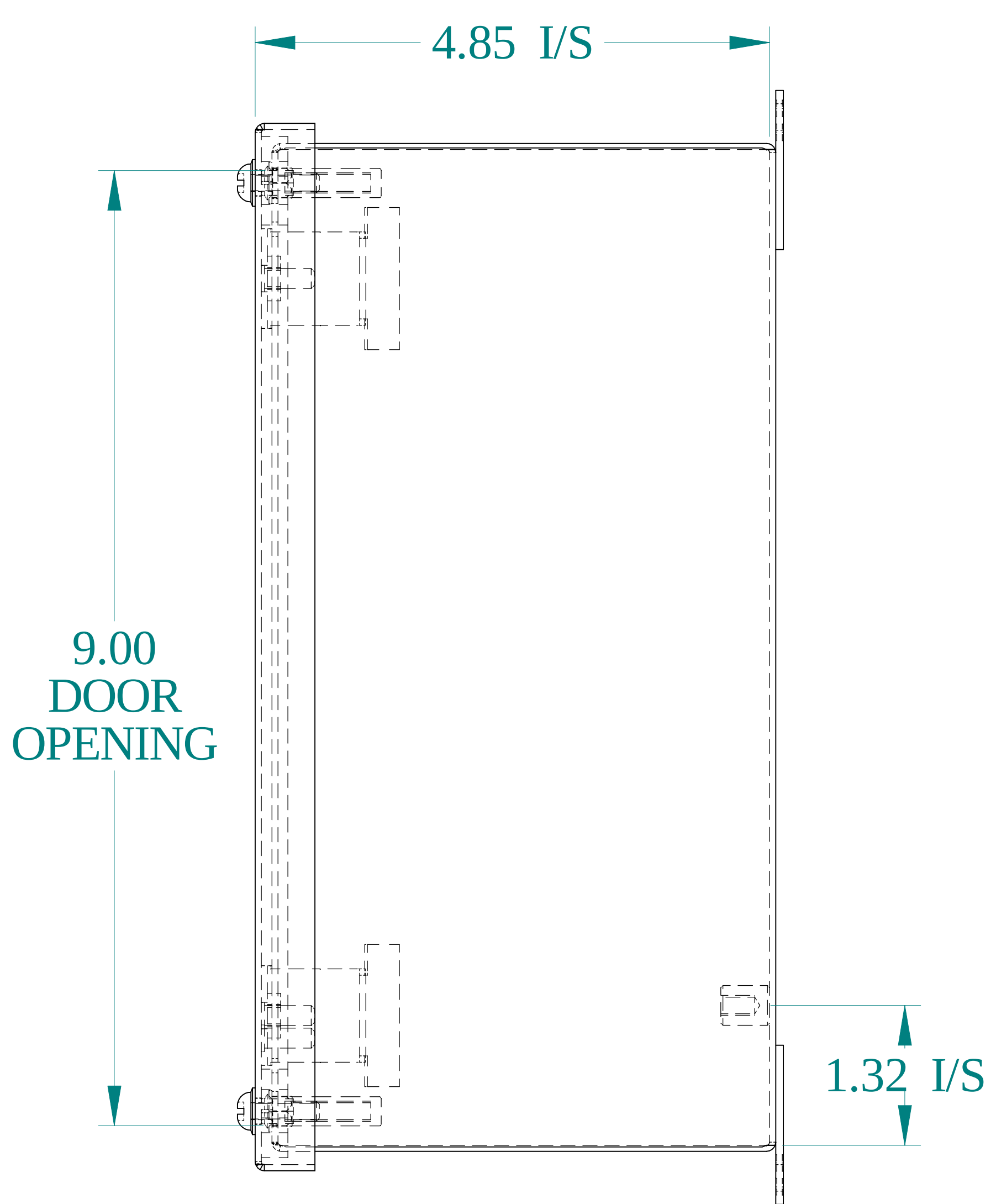
SIDE VIEW
