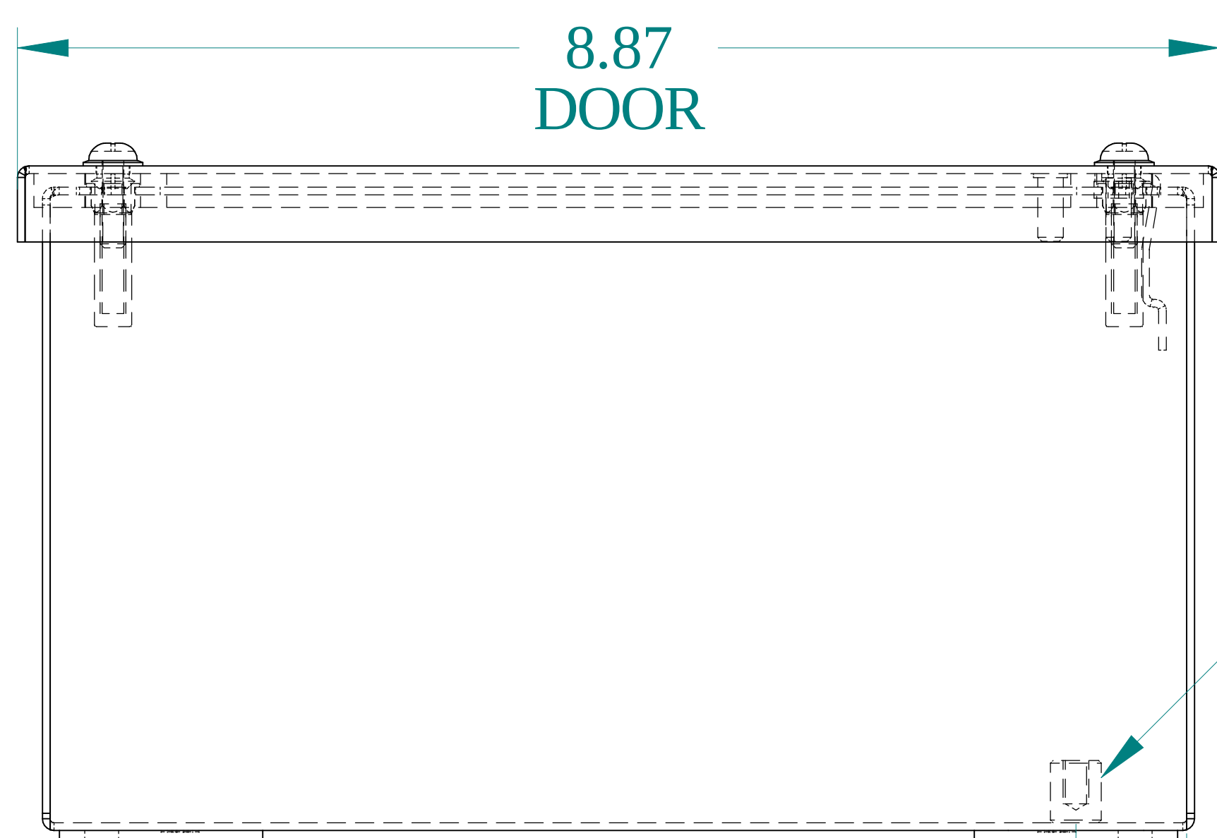
BOTTOM VIEW
