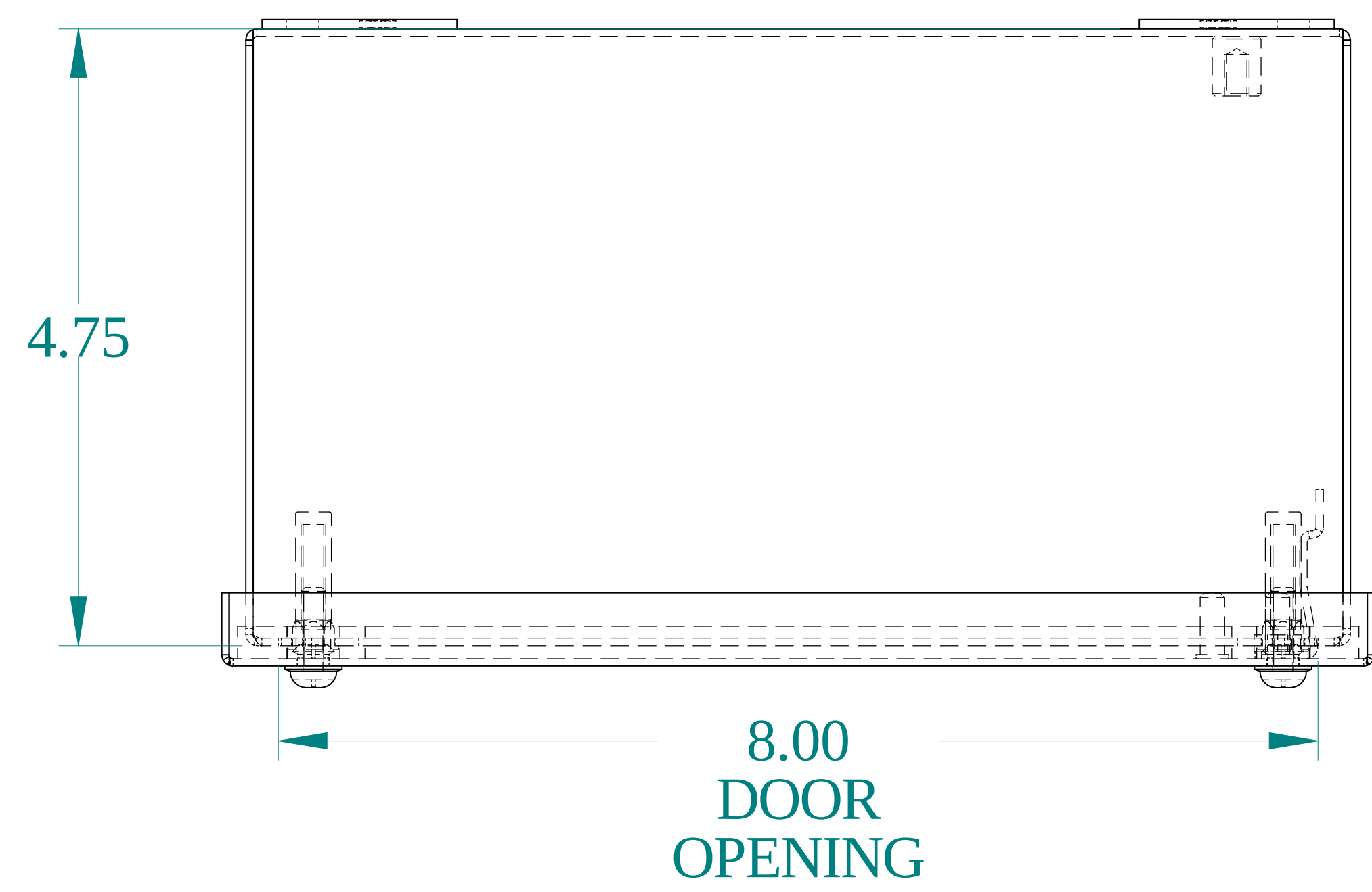
TOP VIEW
