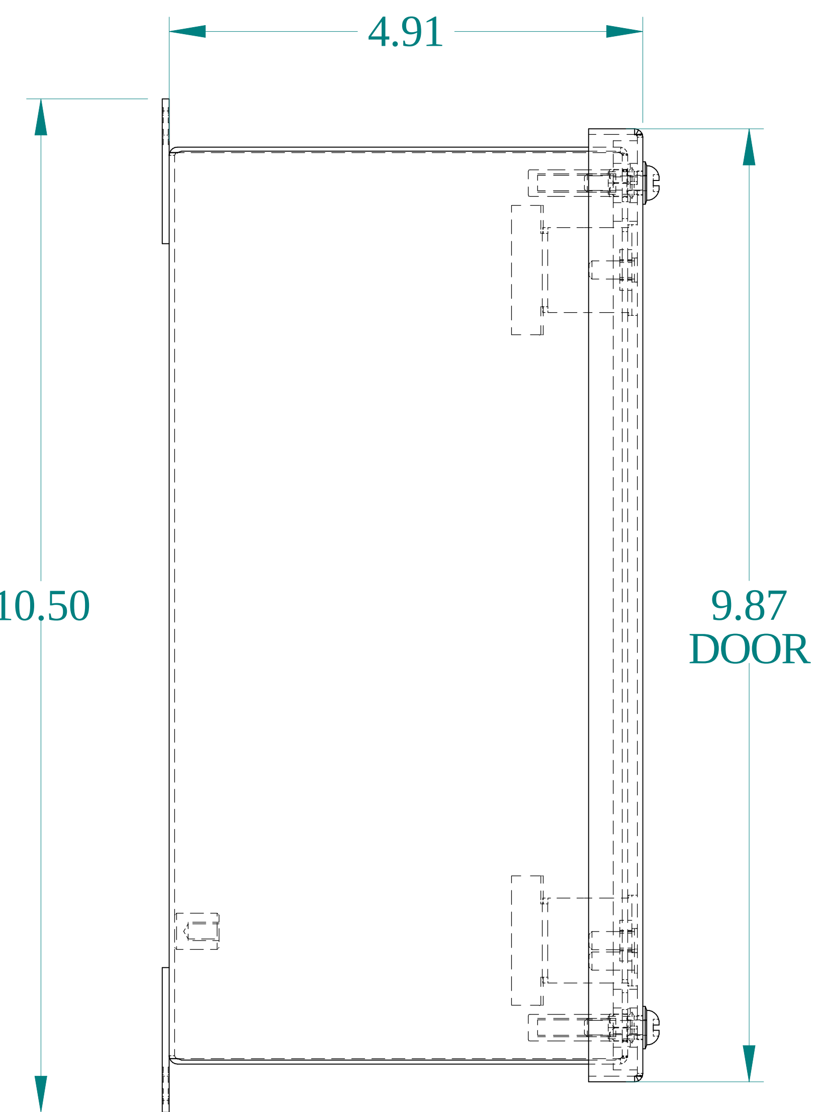
SIDE VIEW
