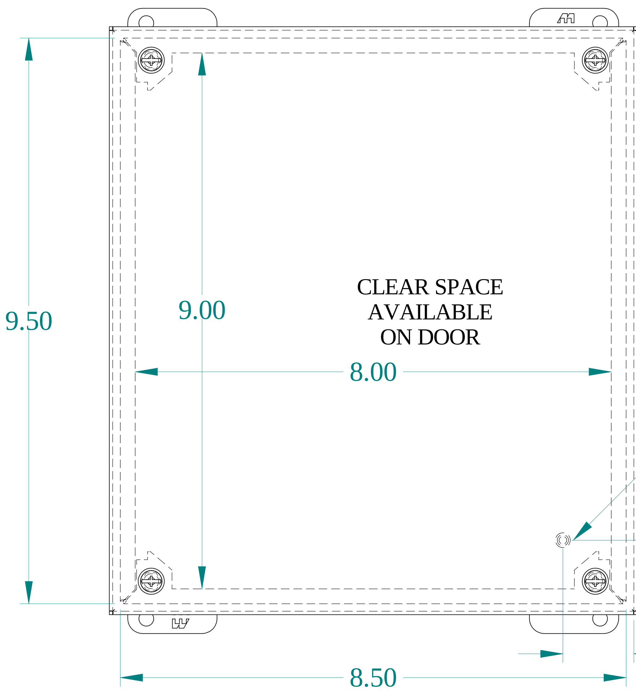
FRONT VIEW
