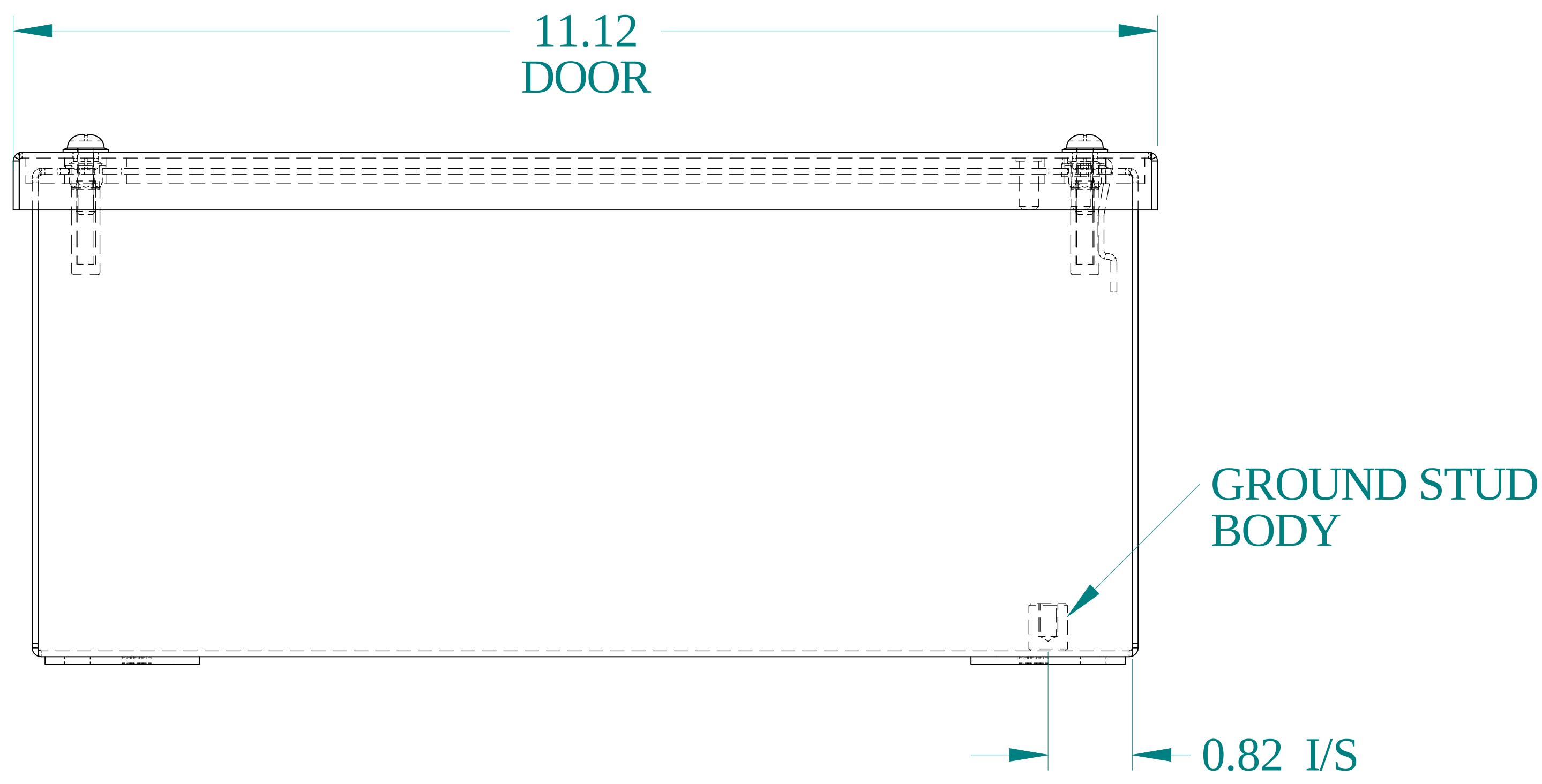
BOTTOM VIEW
