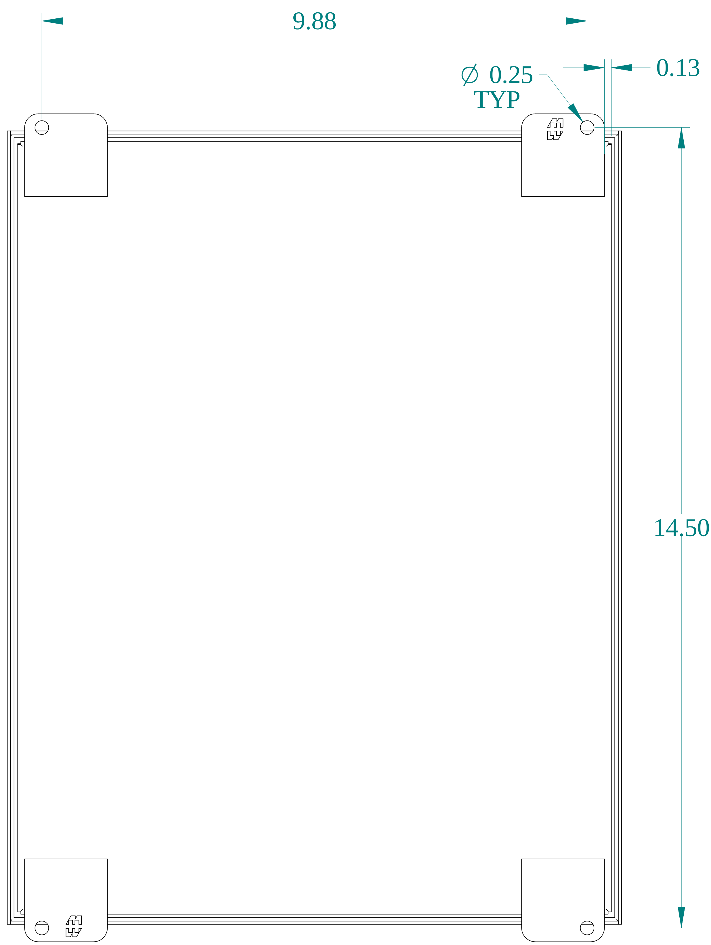
BACK VIEW
