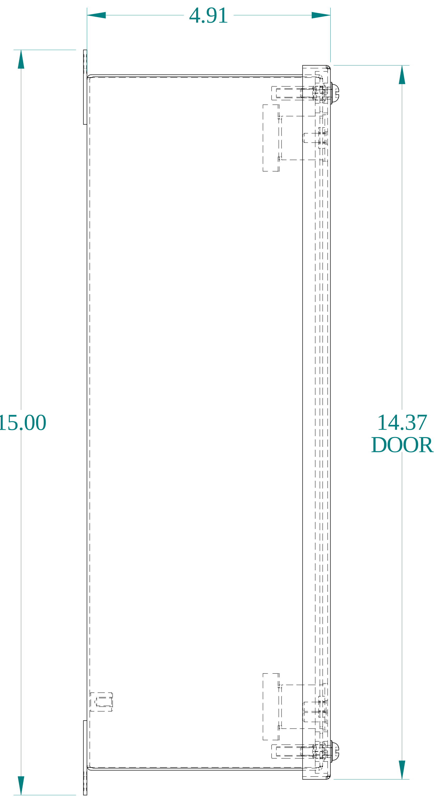
SIDE VIEW
