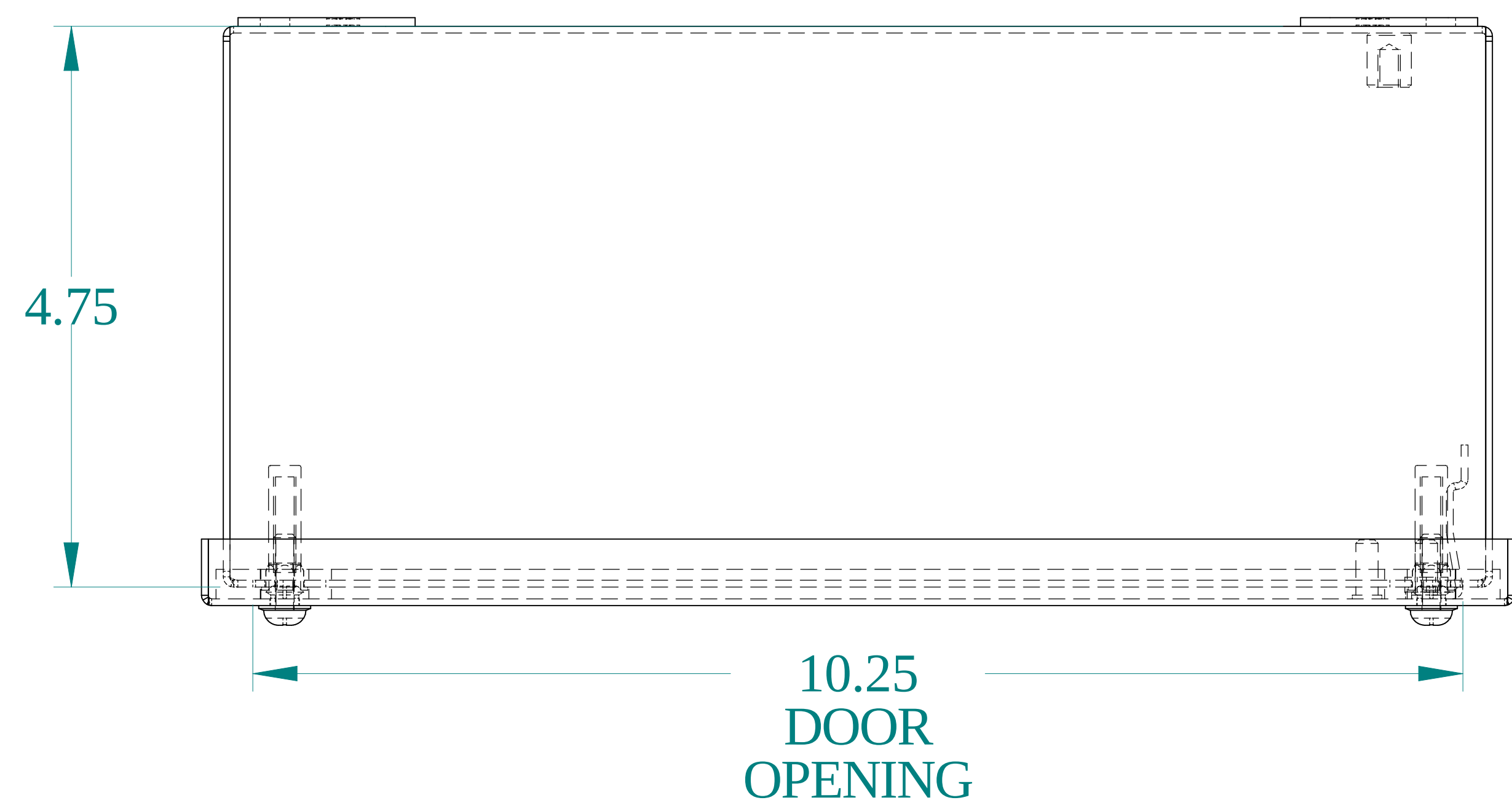
TOP VIEW
