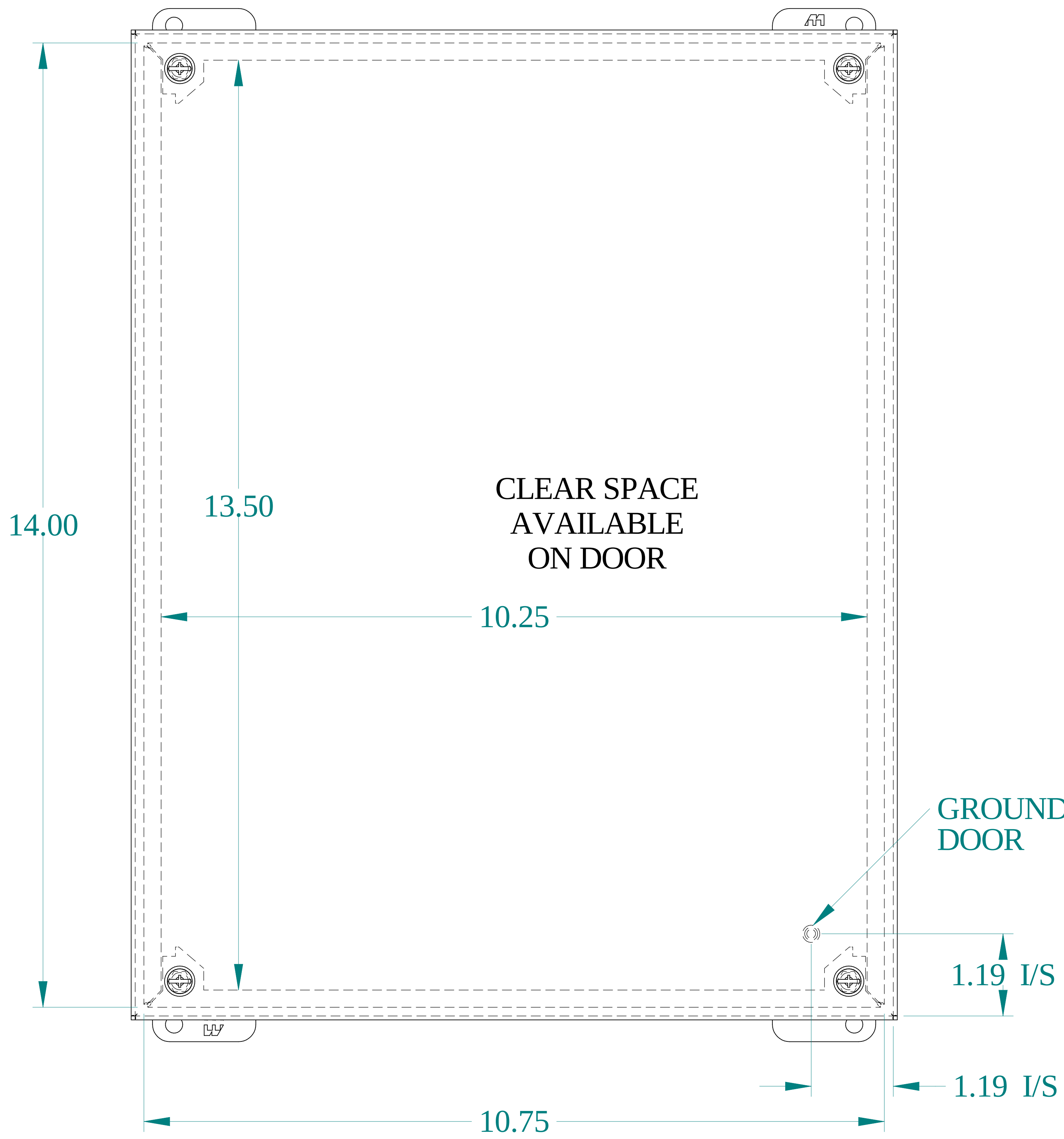
FRONT VIEW
