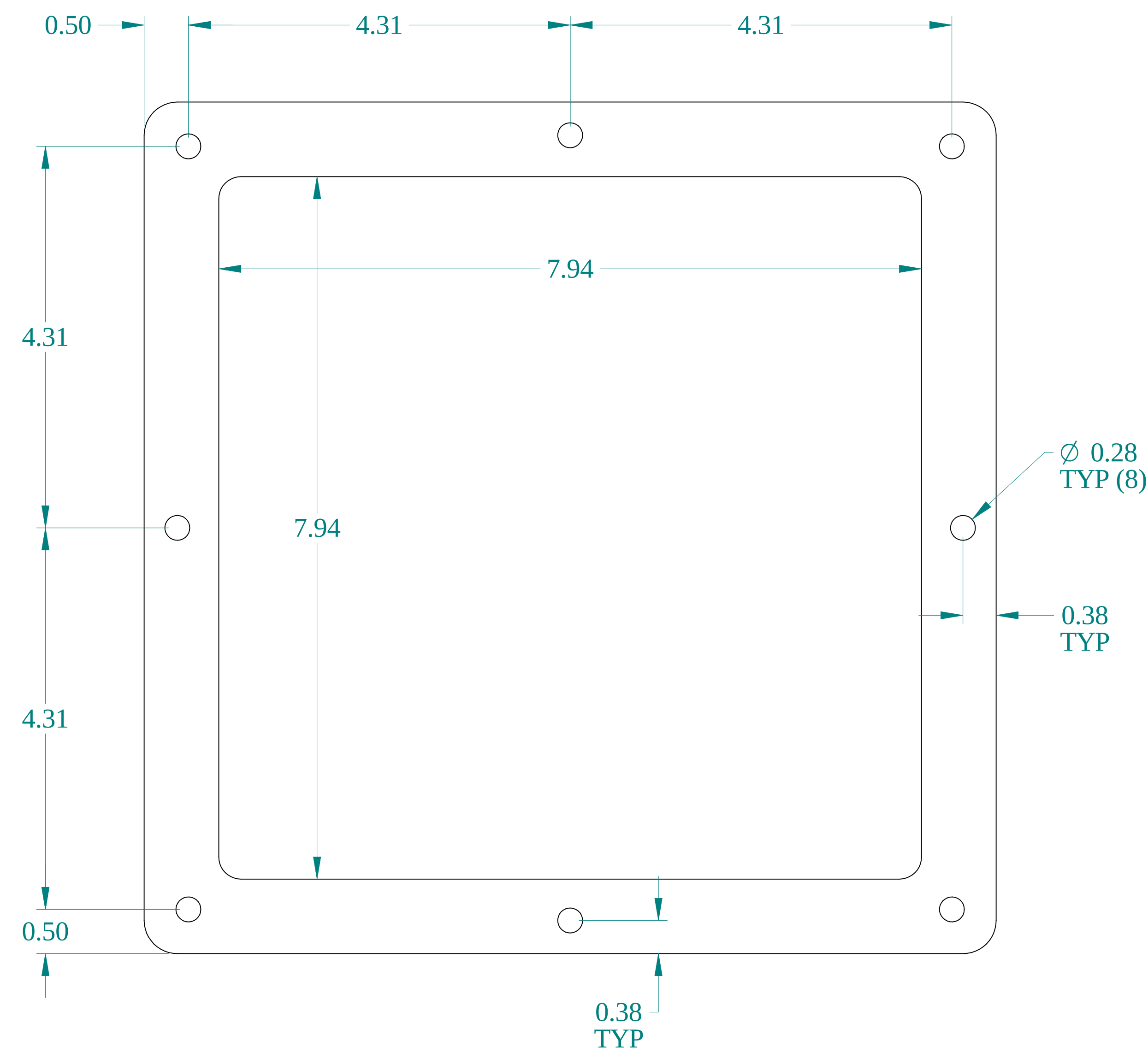
FRONT VIEW
