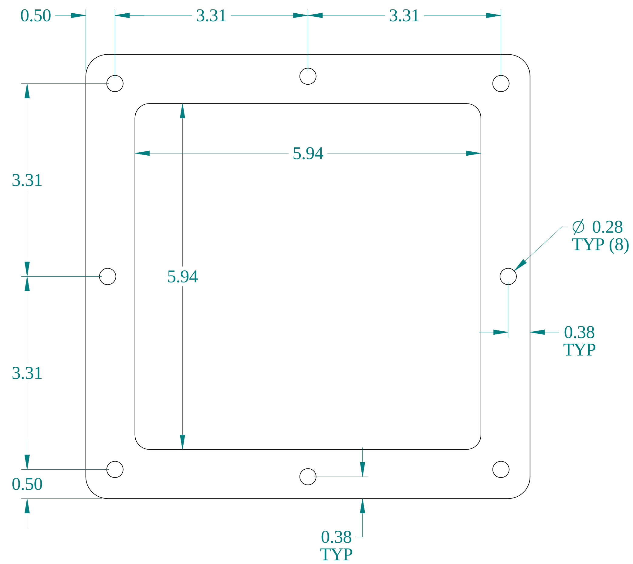
FRONT VIEW
