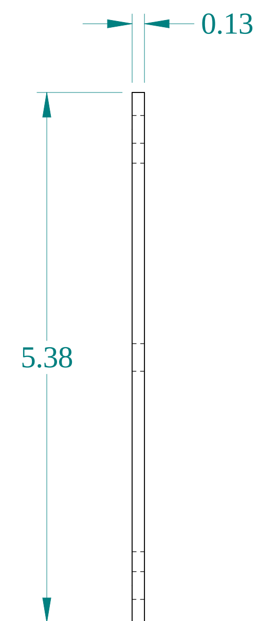
SIDE VIEW
