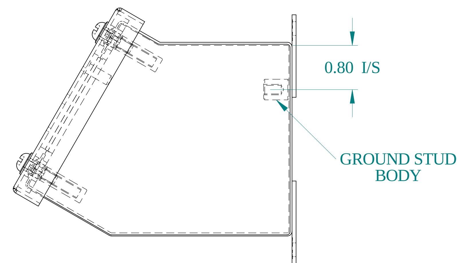
SIDE VIEW
