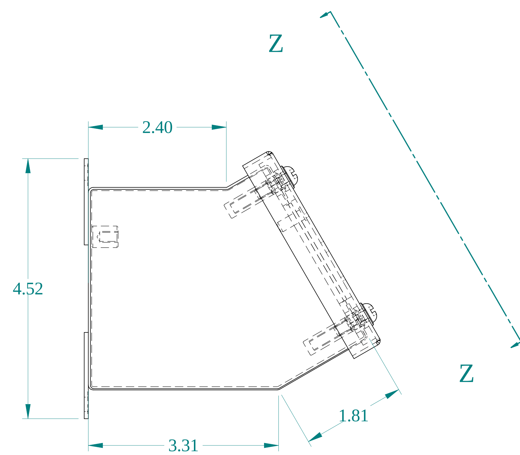
SIDE VIEW
