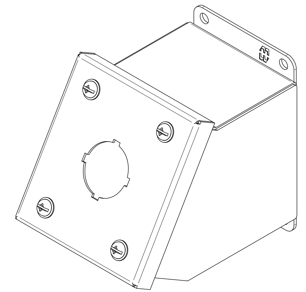
ISOMETRIC VIEWS
