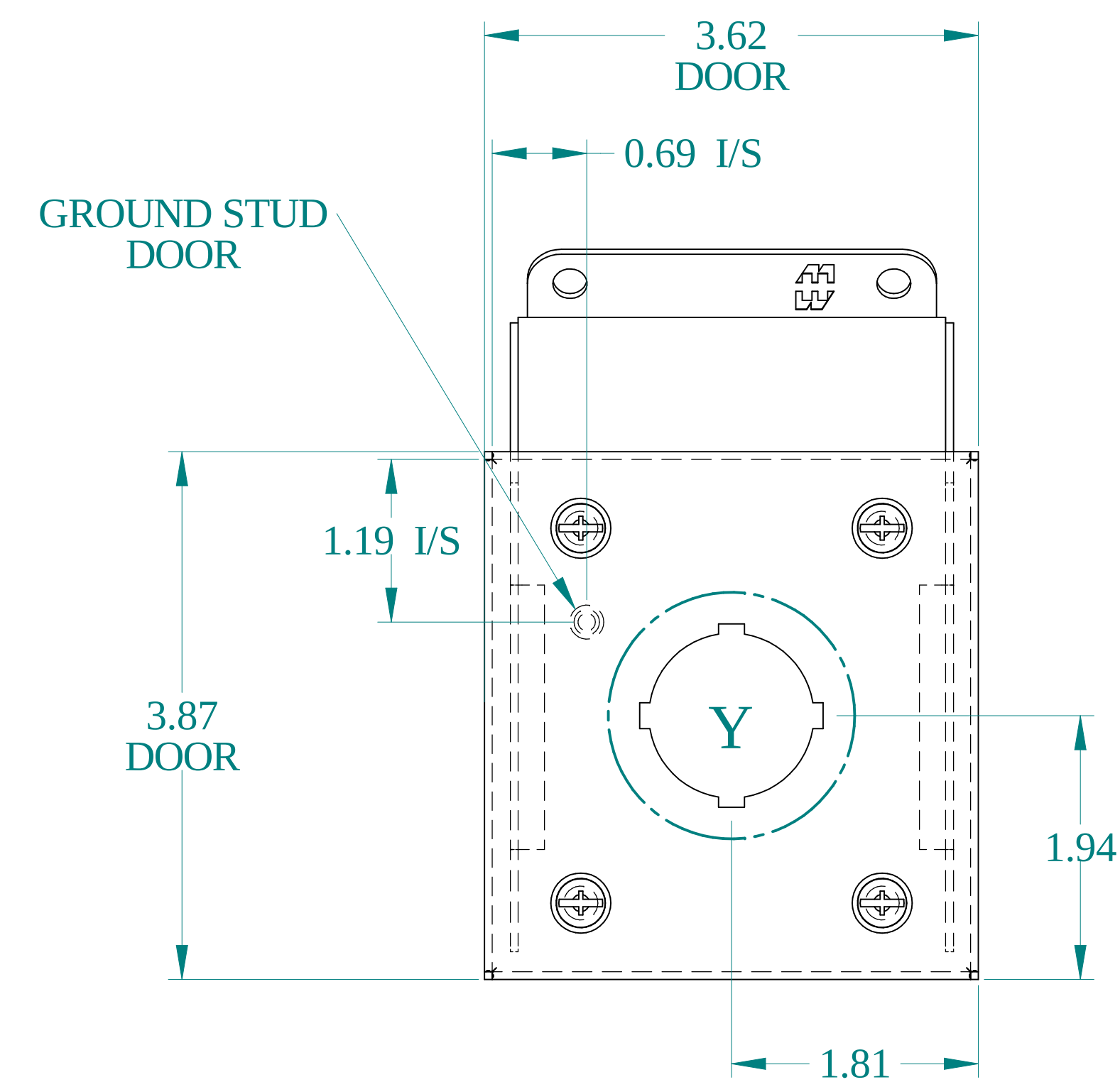
VIEW Z-Z
