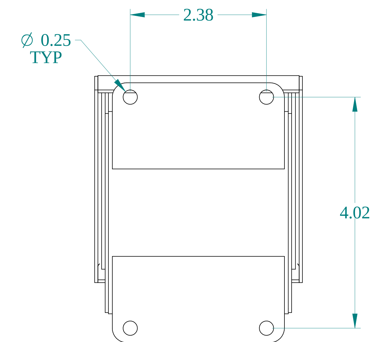
BACK VIEW
