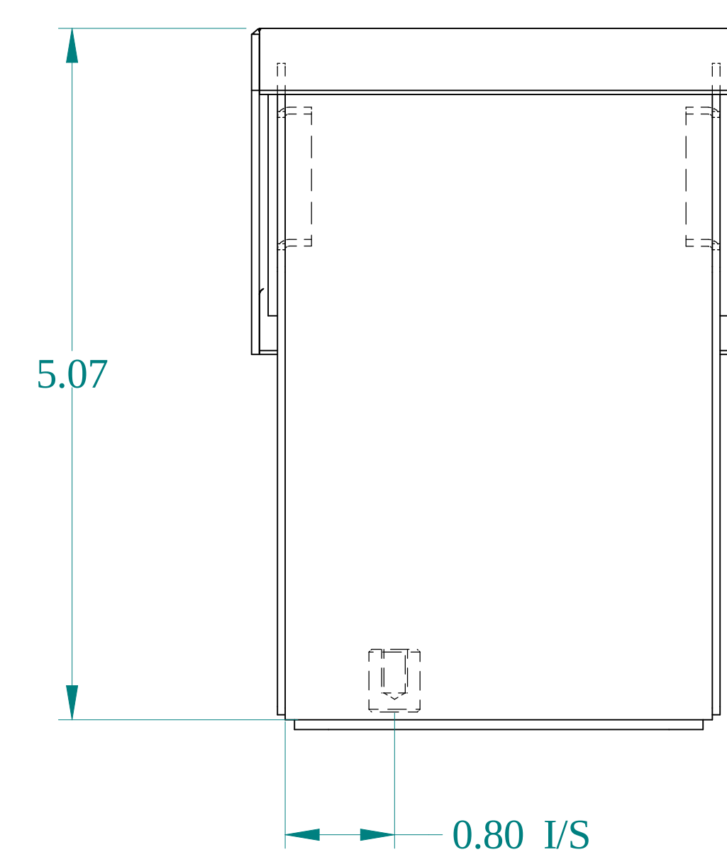
BOTTOM VIEW
