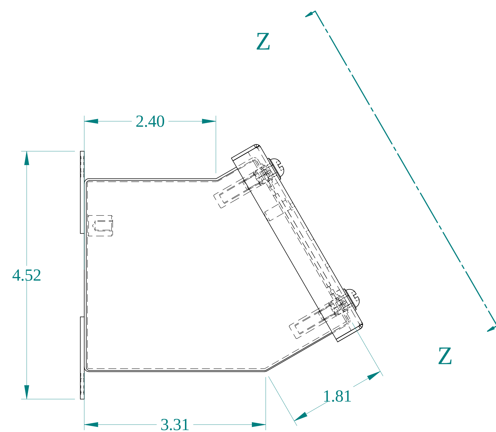
SIDE VIEW
