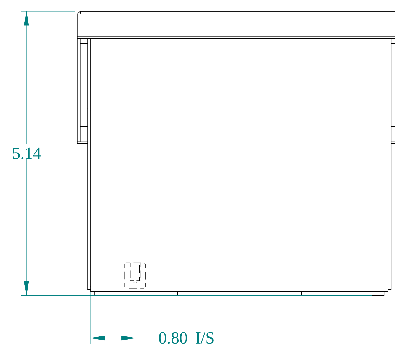
BOTTOM VIEW
