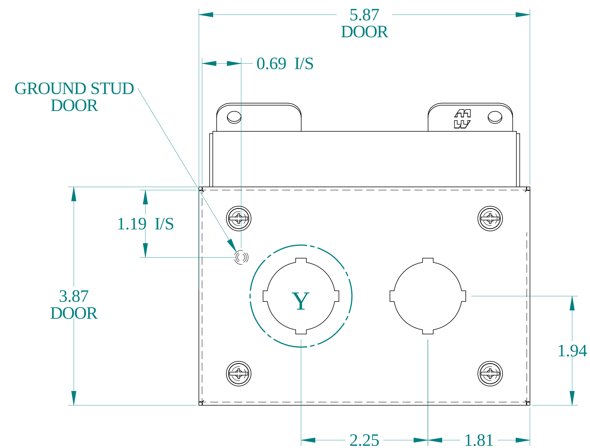
VIEW Z-Z
