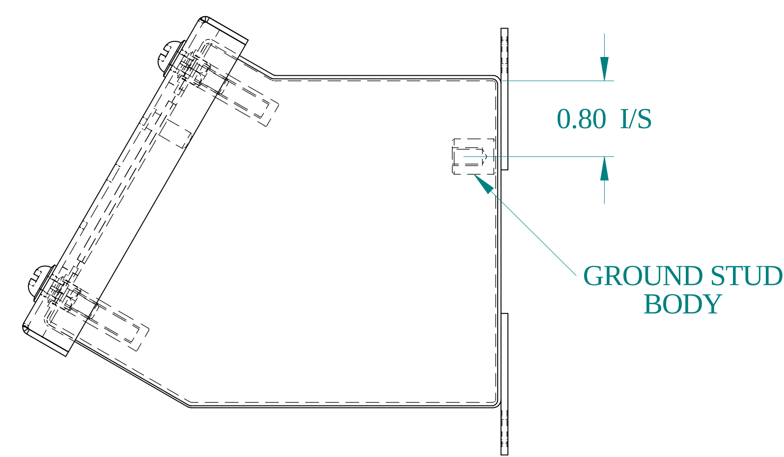
SIDE VIEW
