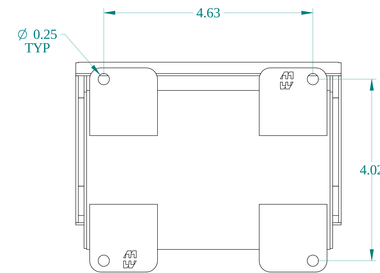
BACK VIEW
