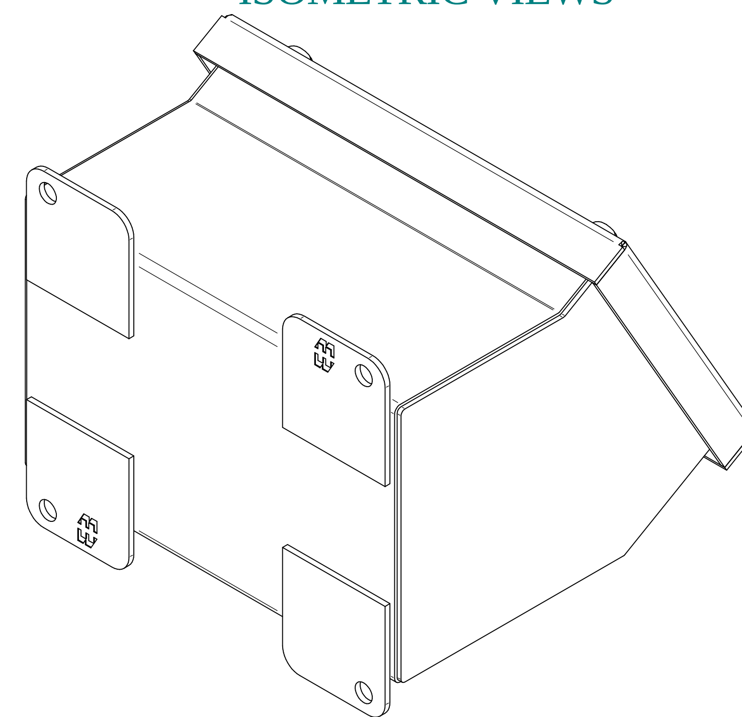
ISOMETRIC VIEWS
