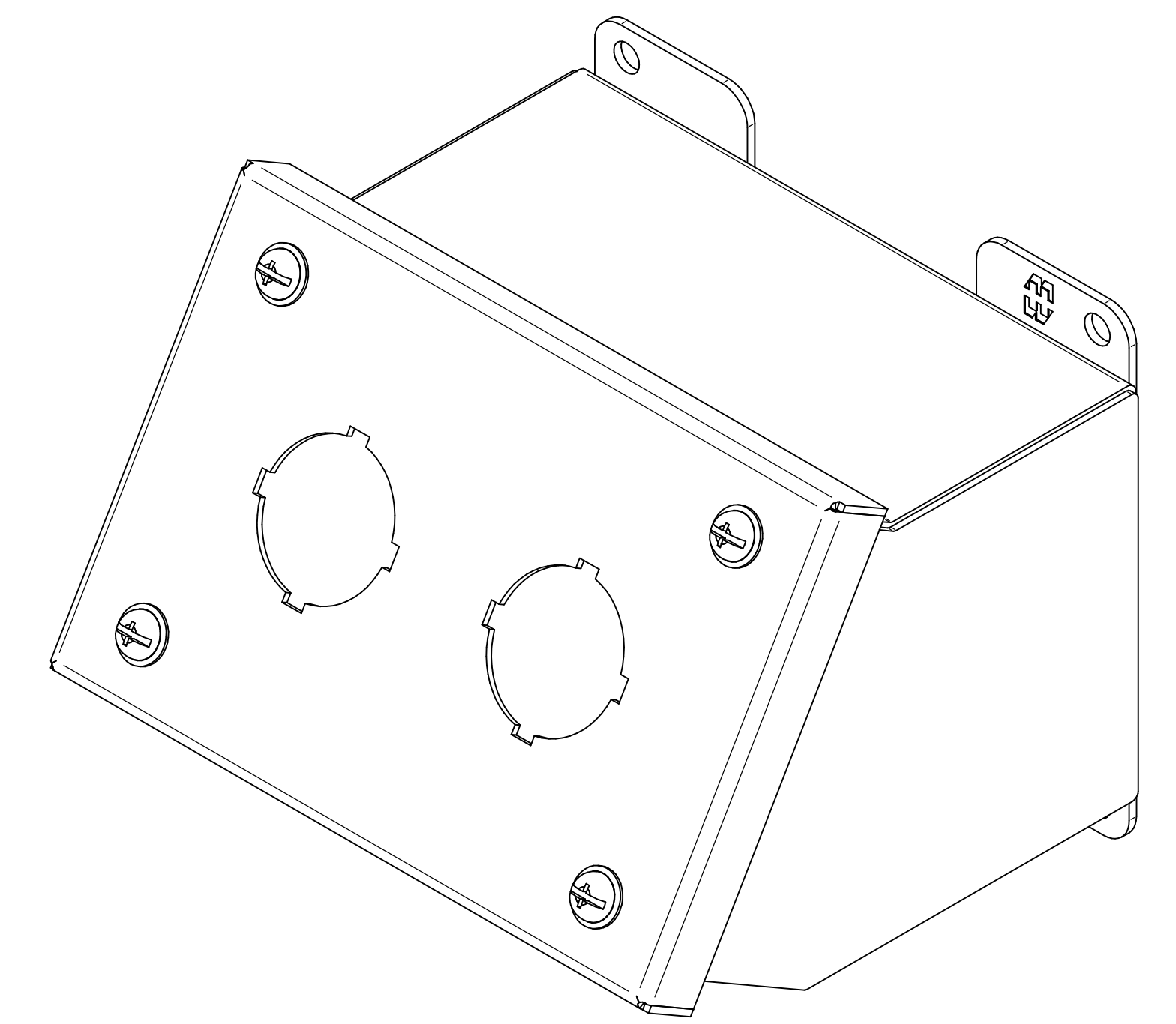
ISOMETRIC VIEWS
