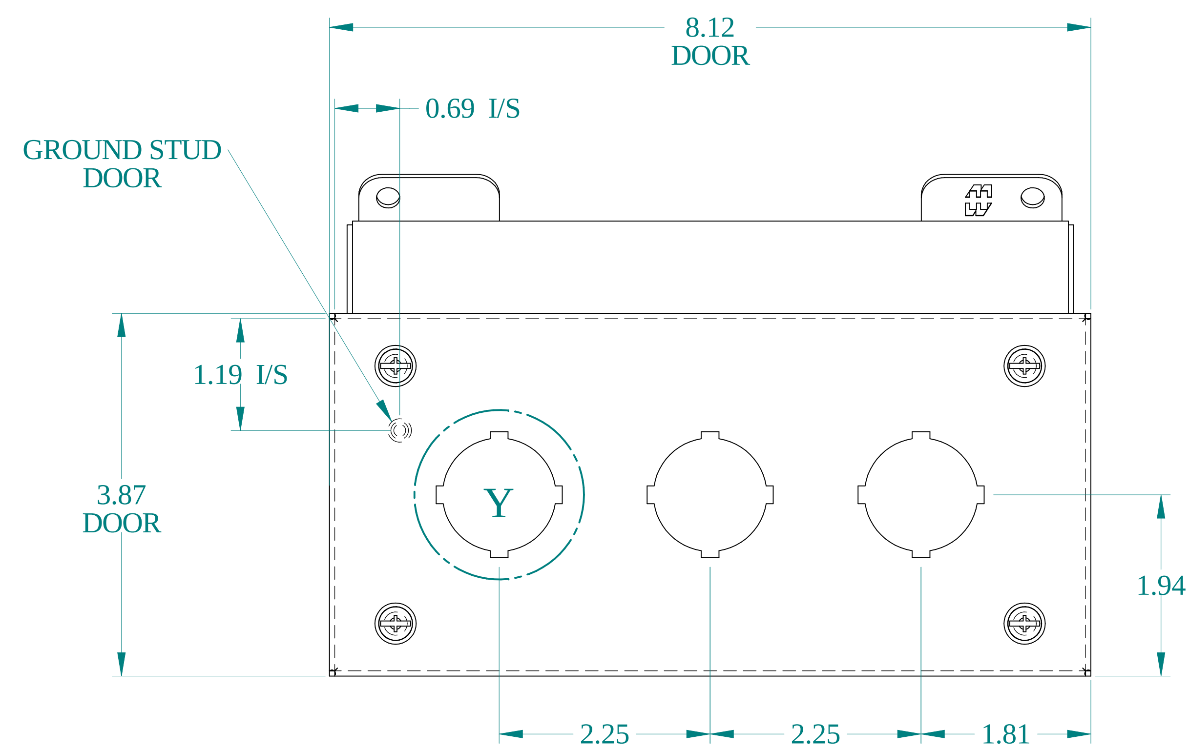
VIEW Z-Z
