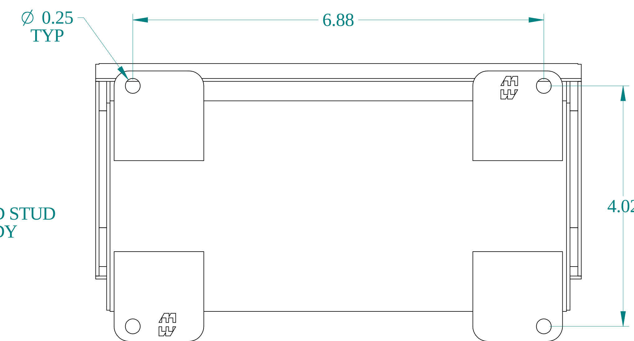
BACK VIEW
