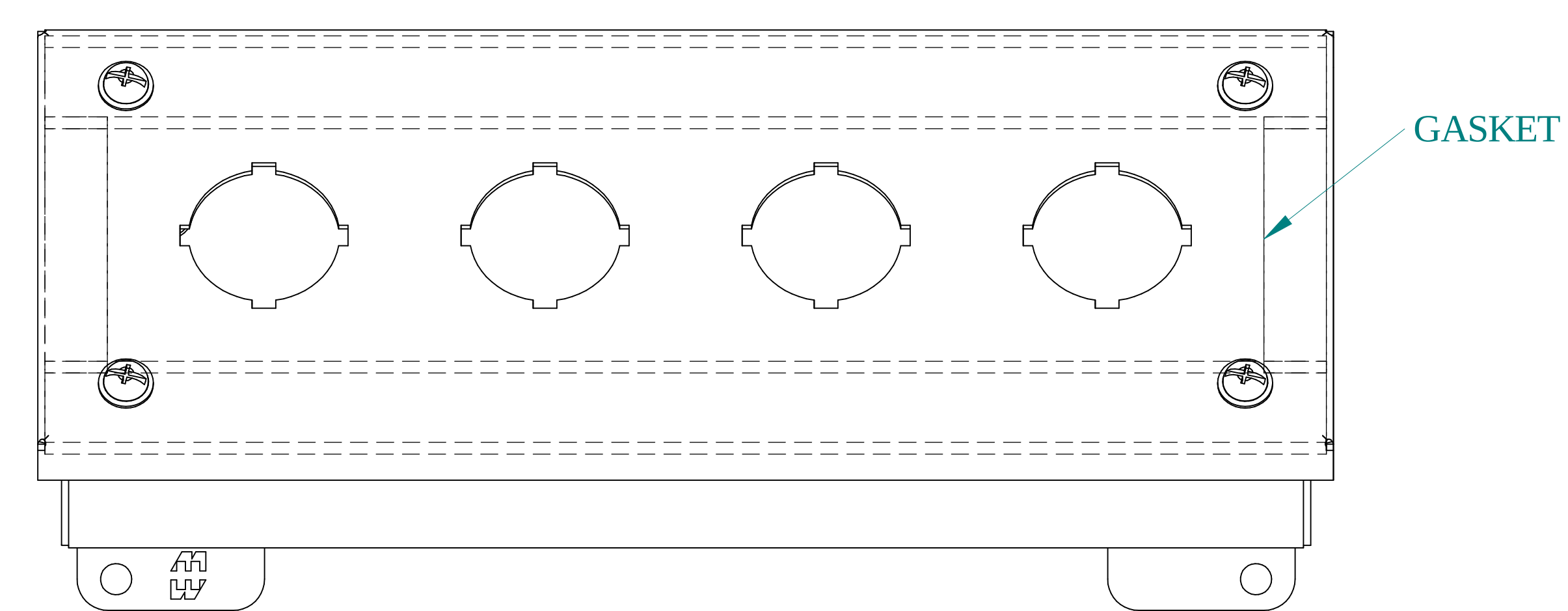
FRONT VIEW
