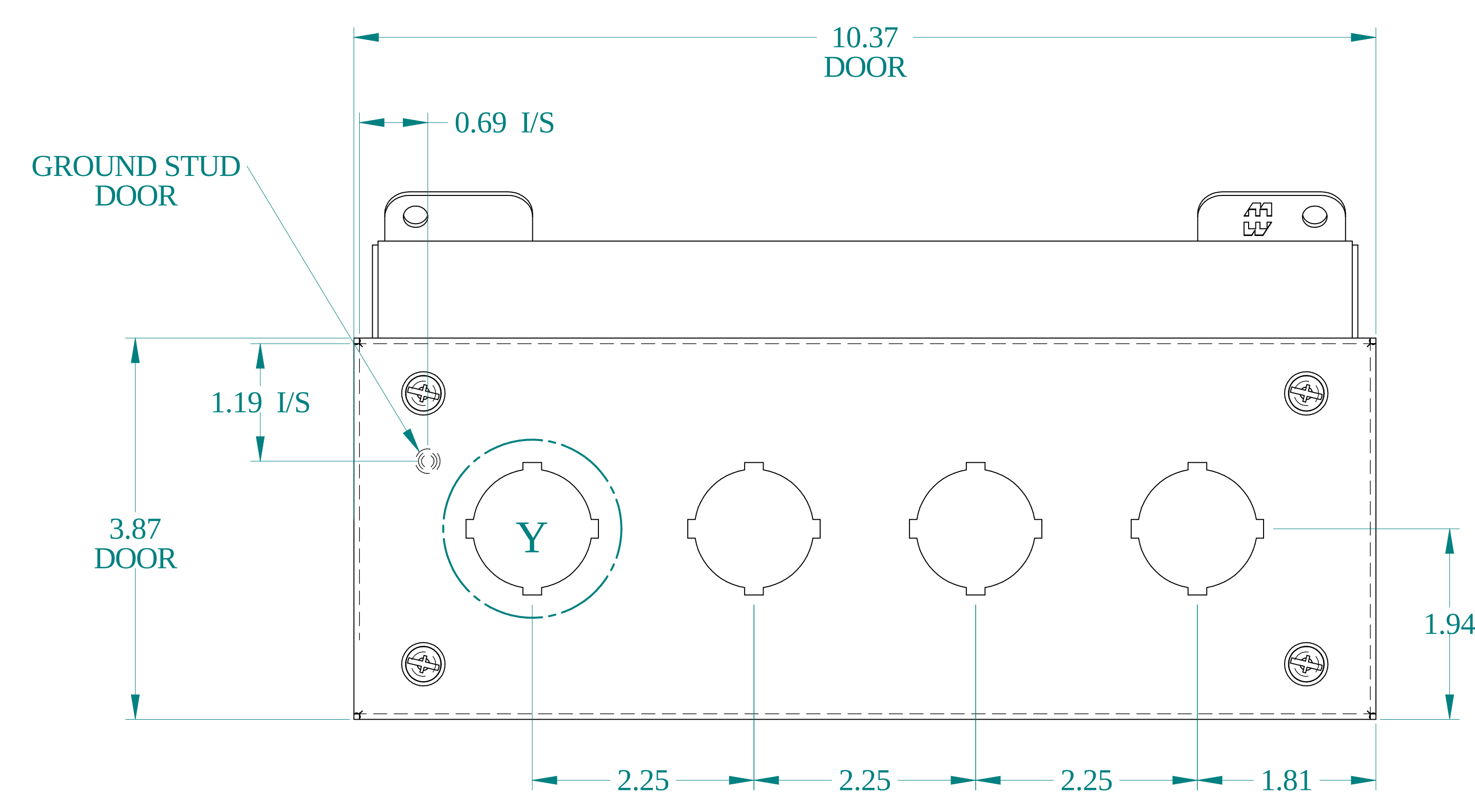
VIEW Z-Z
