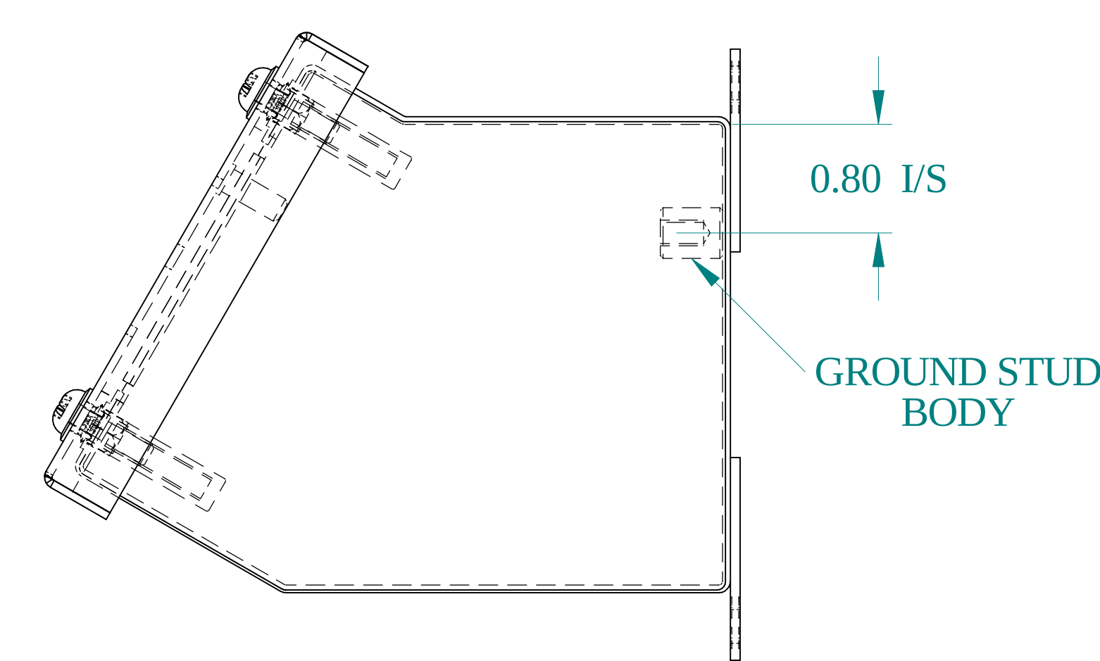
SIDE VIEW
