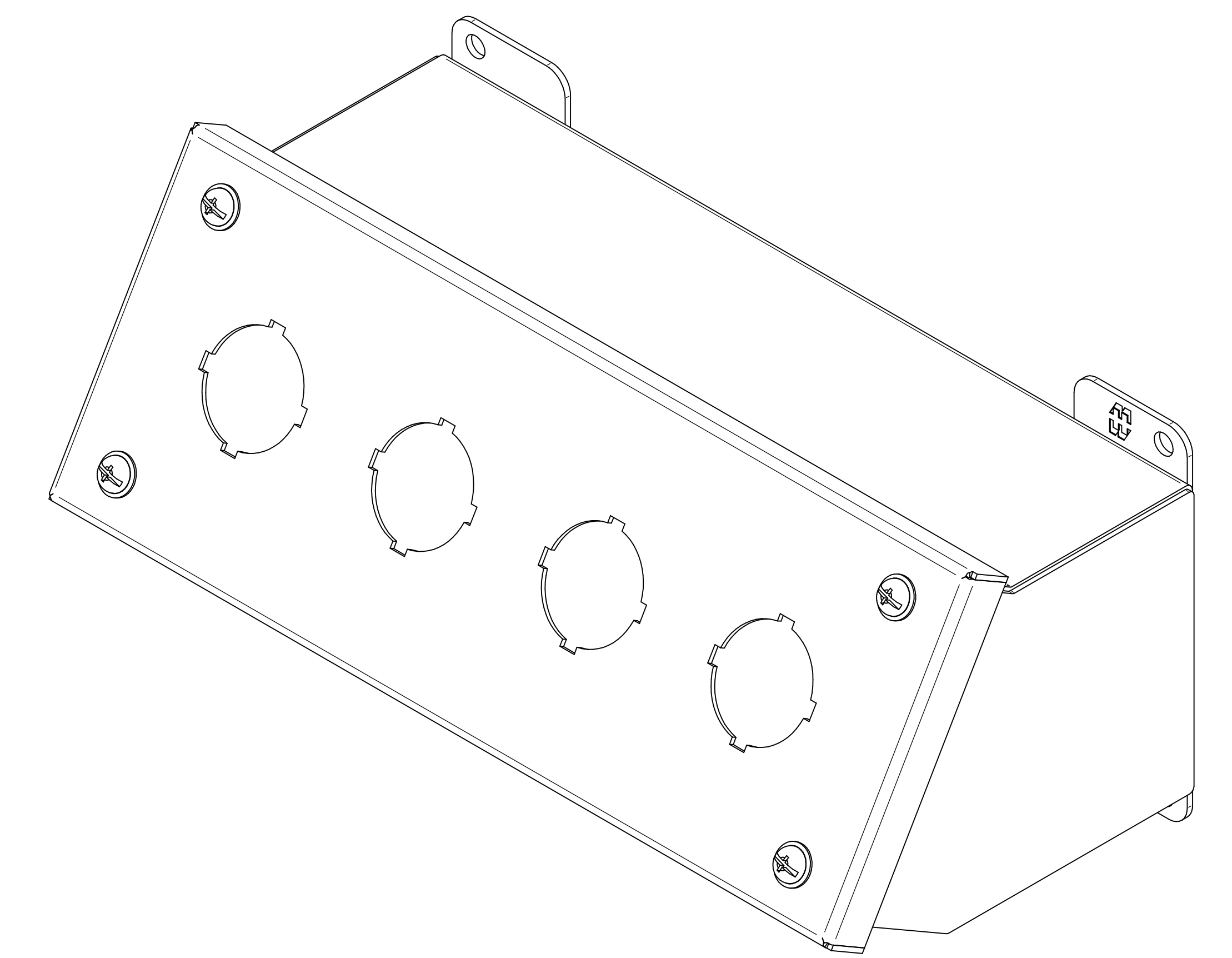
ISOMETRIC VIEWS
