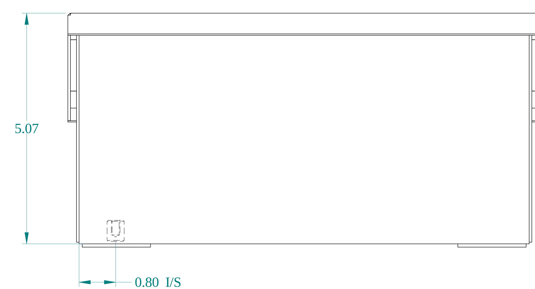
BOTTOM VIEW
