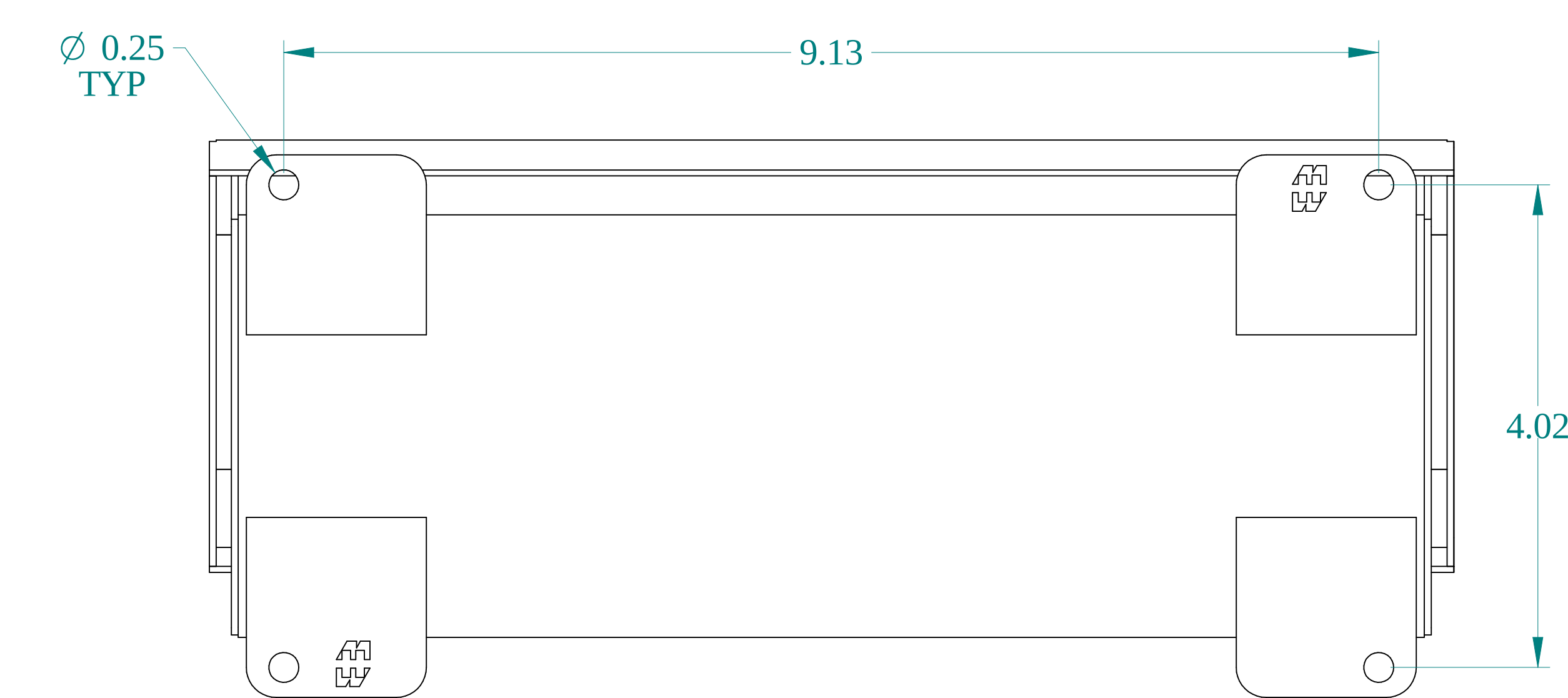
BACK VIEW
