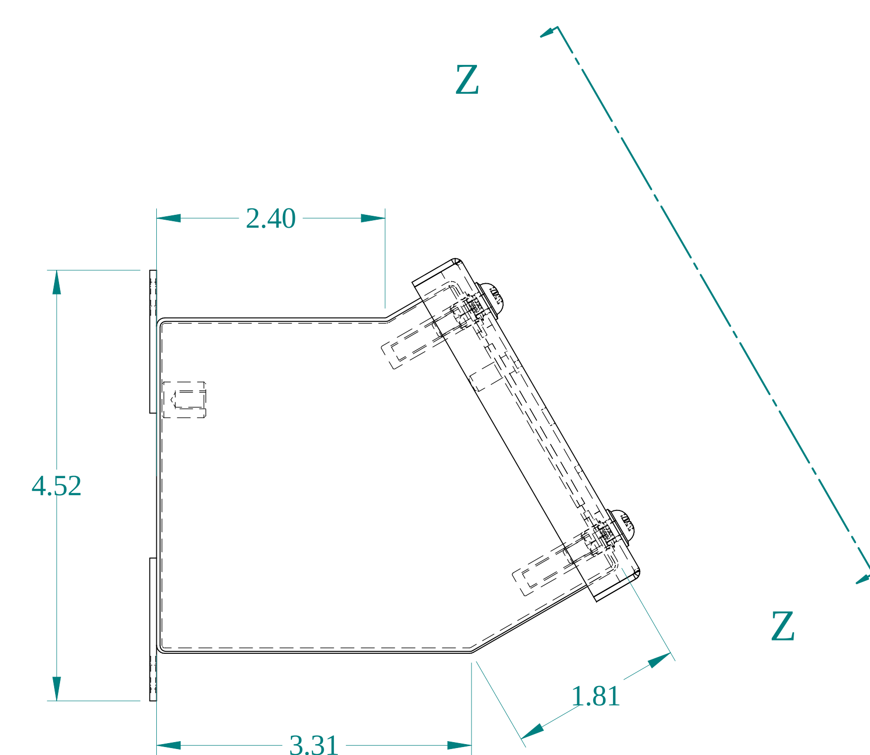
SIDE VIEW
