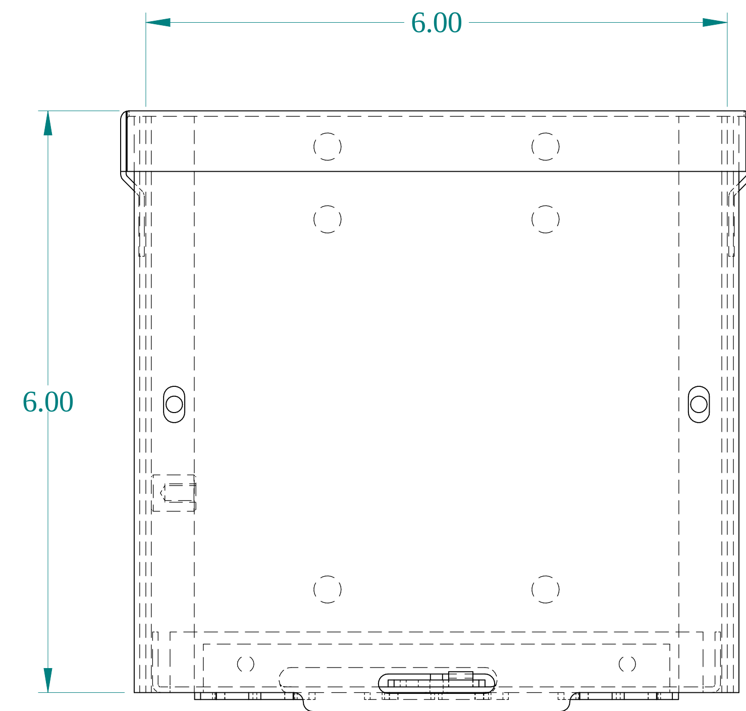
FRONT VIEW
