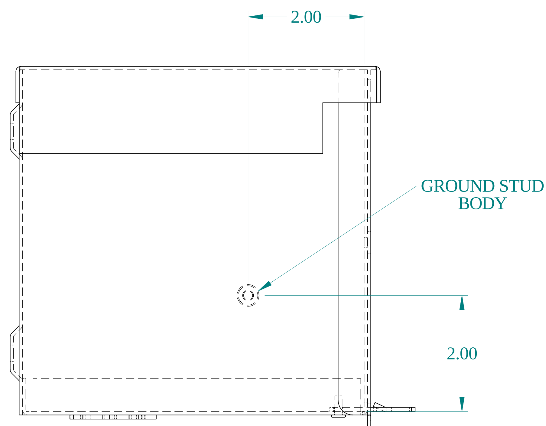
SIDE VIEW
