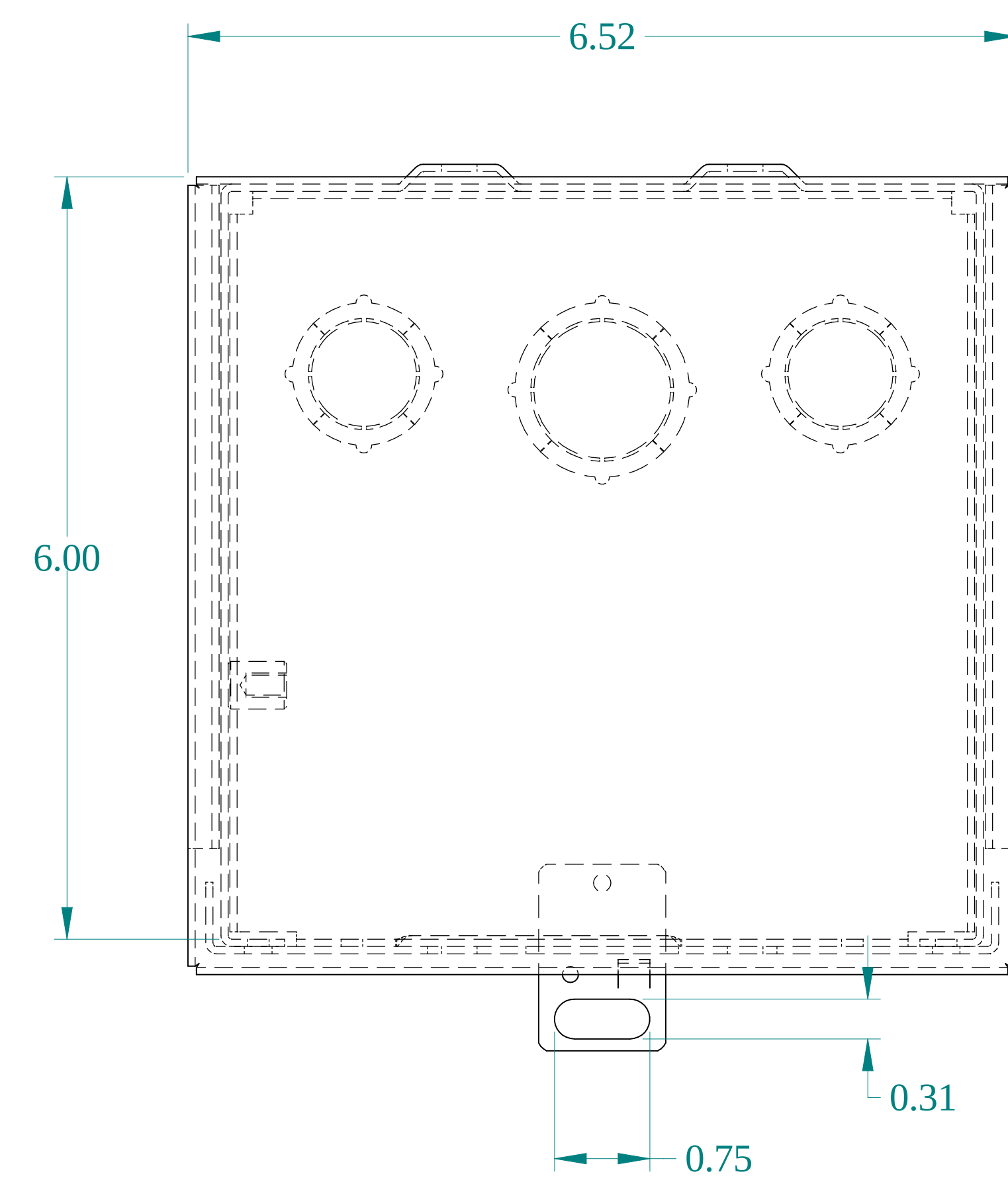
TOP VIEW
