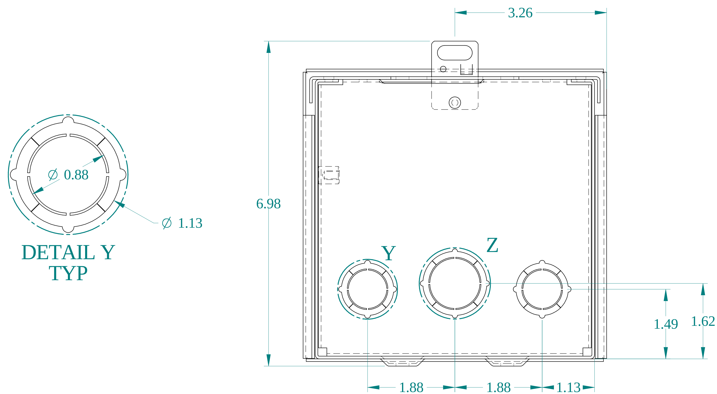
BOTTOM VIEW
