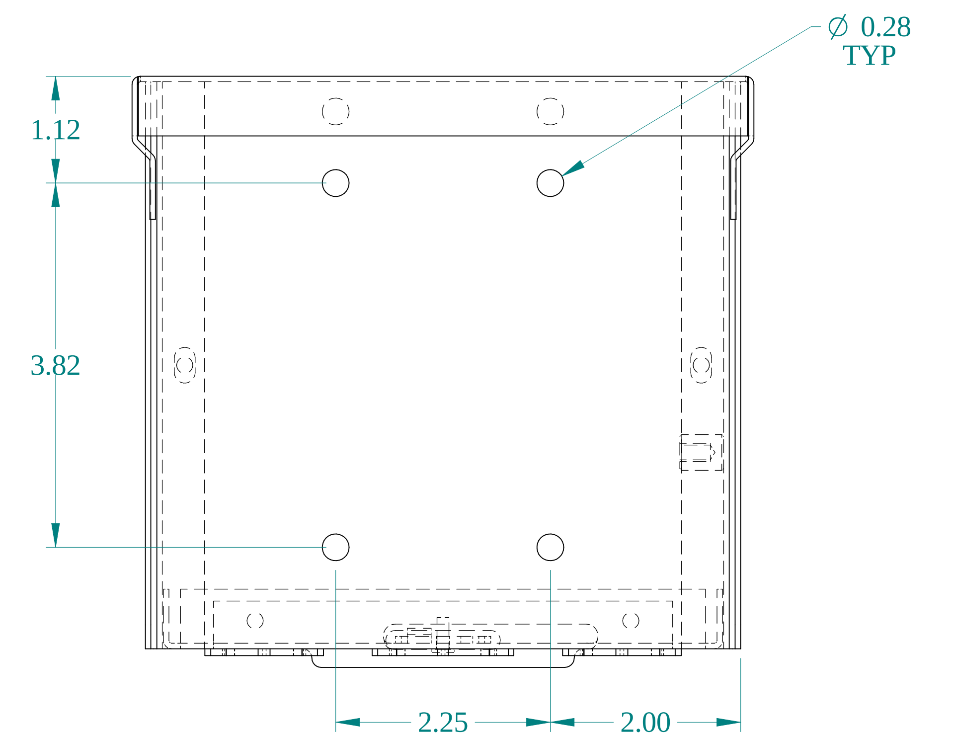
BACK VIEW
