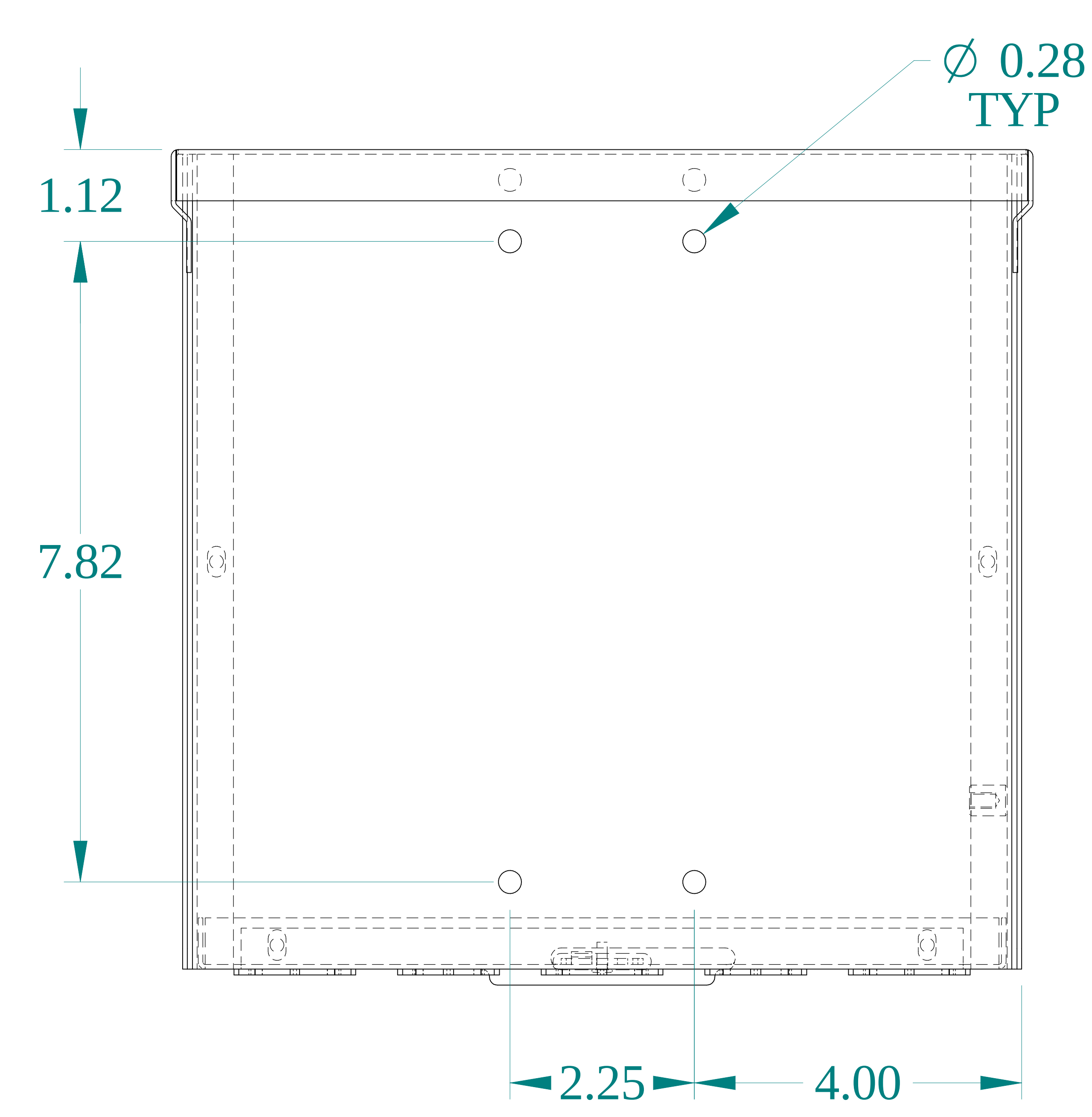
BACK VIEW
