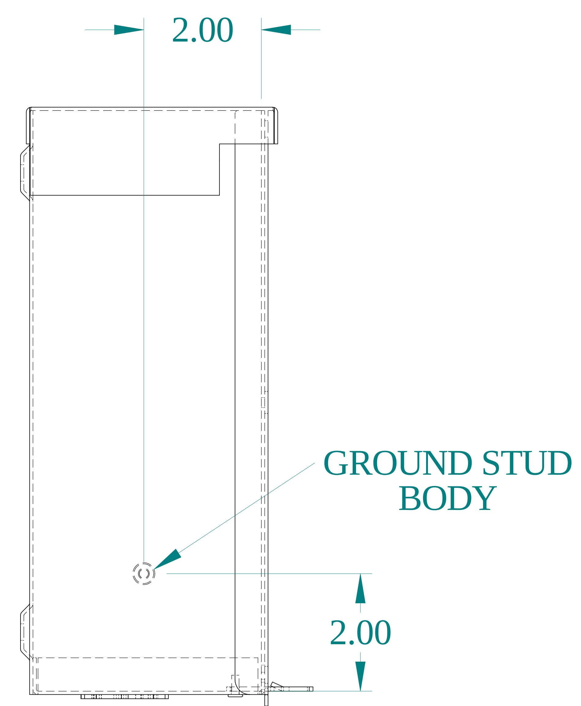
SIDE VIEW
