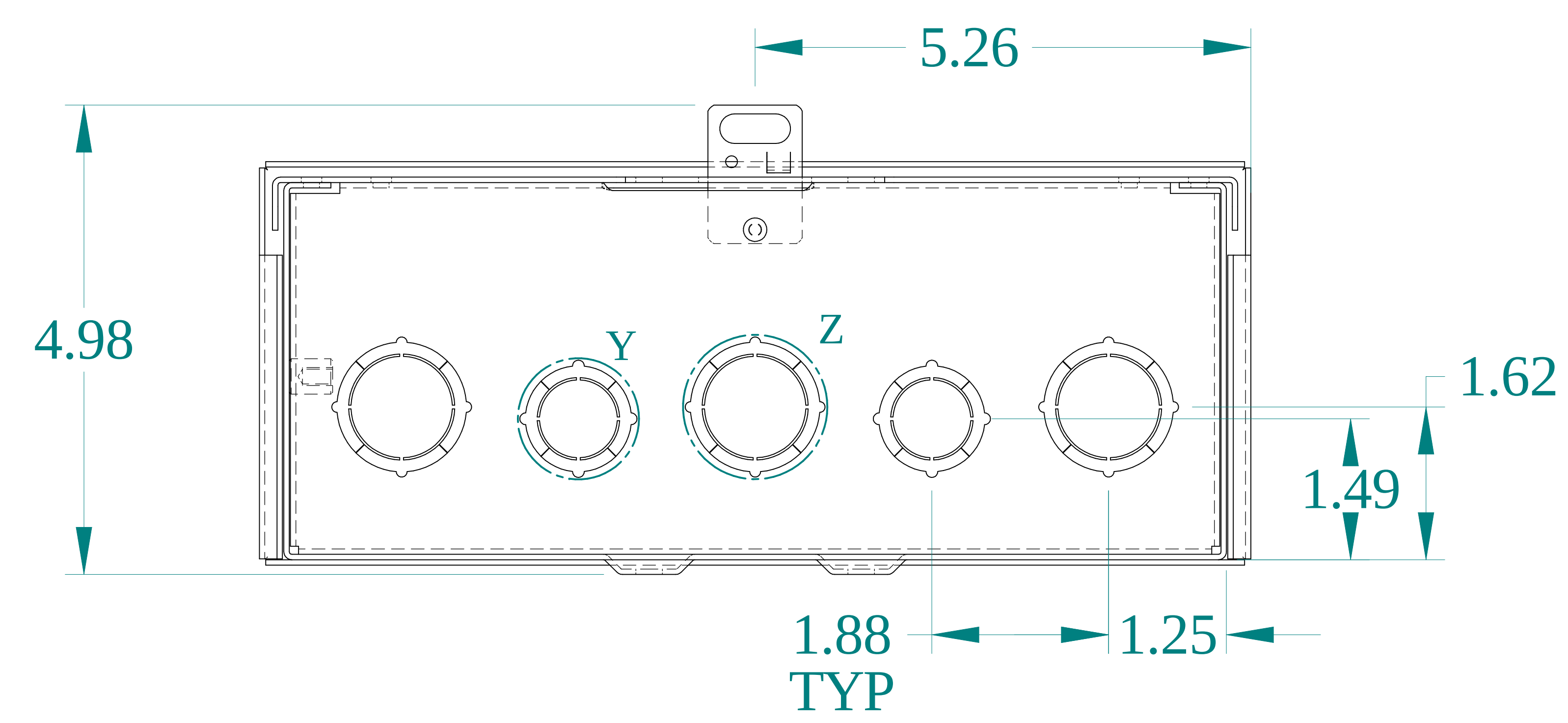
BOTTOM VIEW
