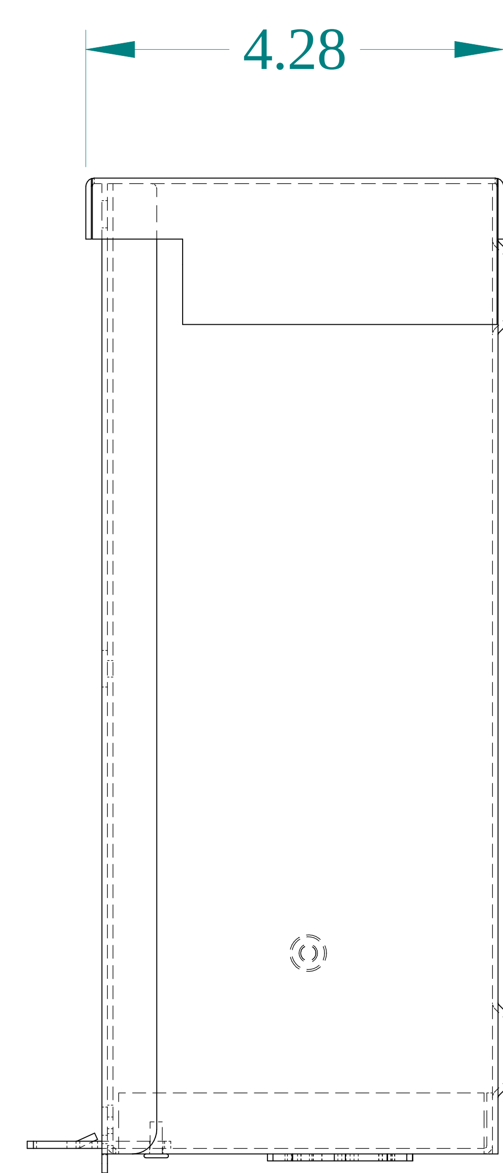
SIDE VIEW
