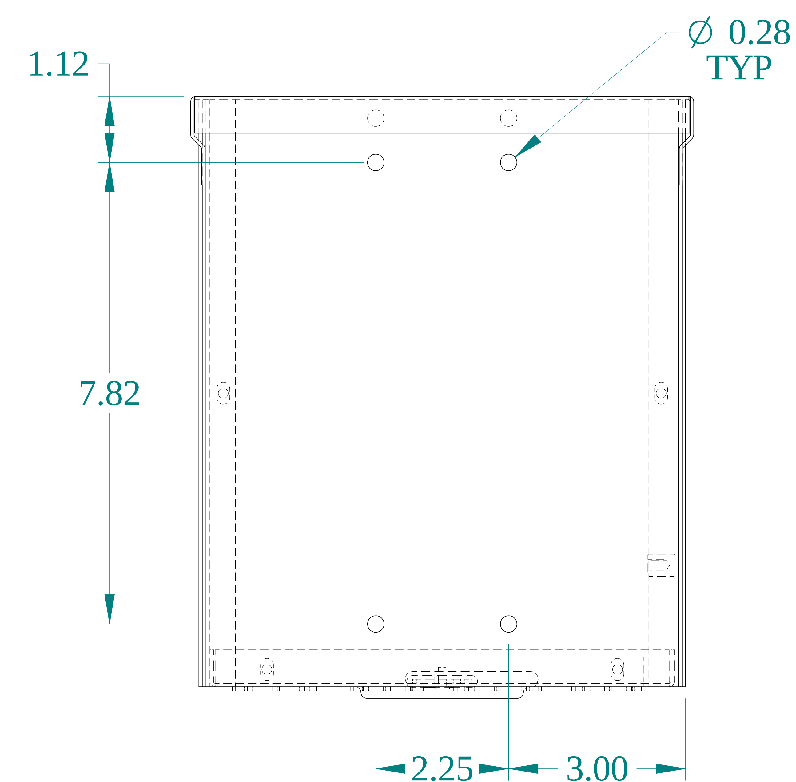
BACK VIEW
