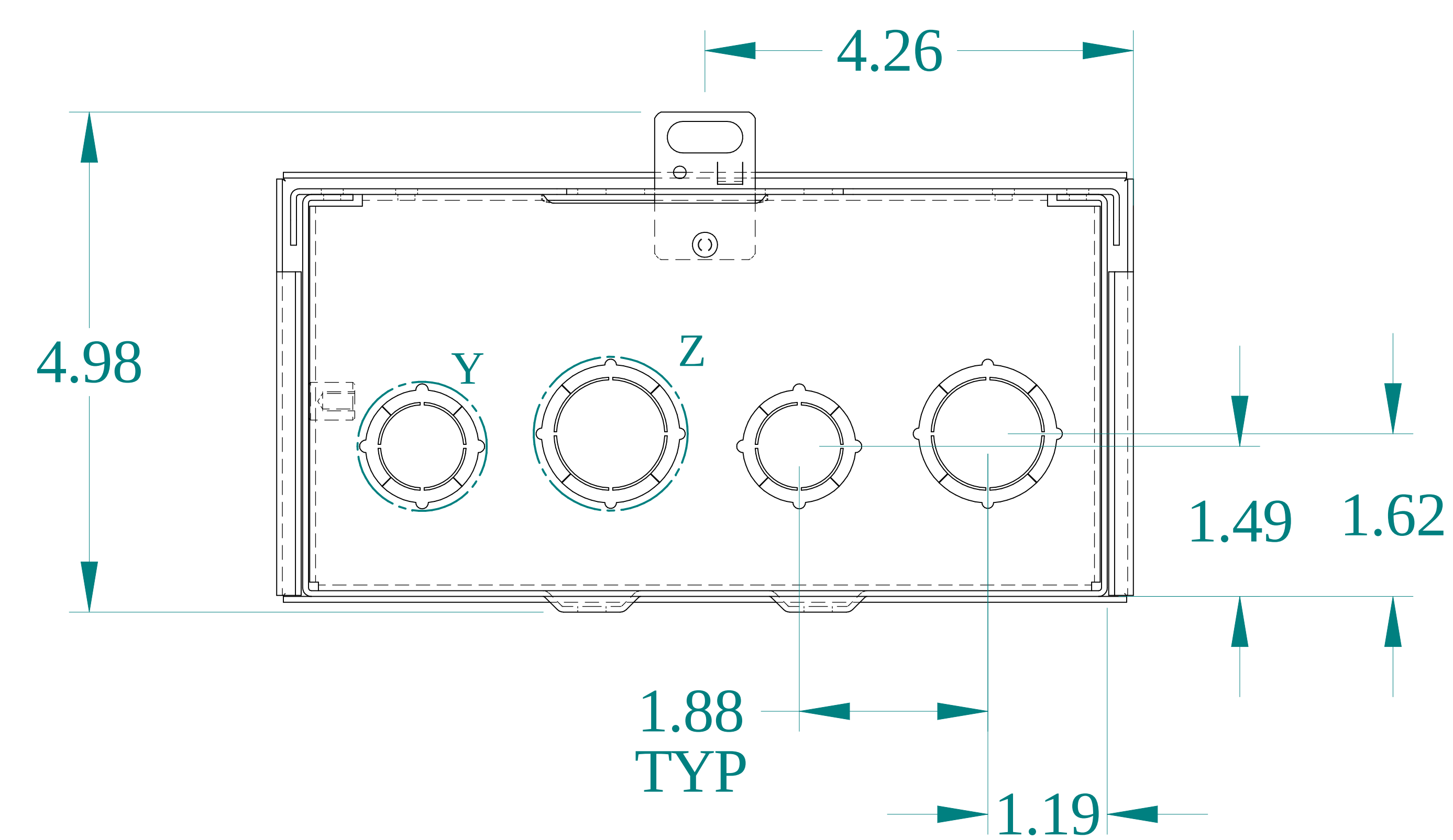
BOTTOM VIEW
