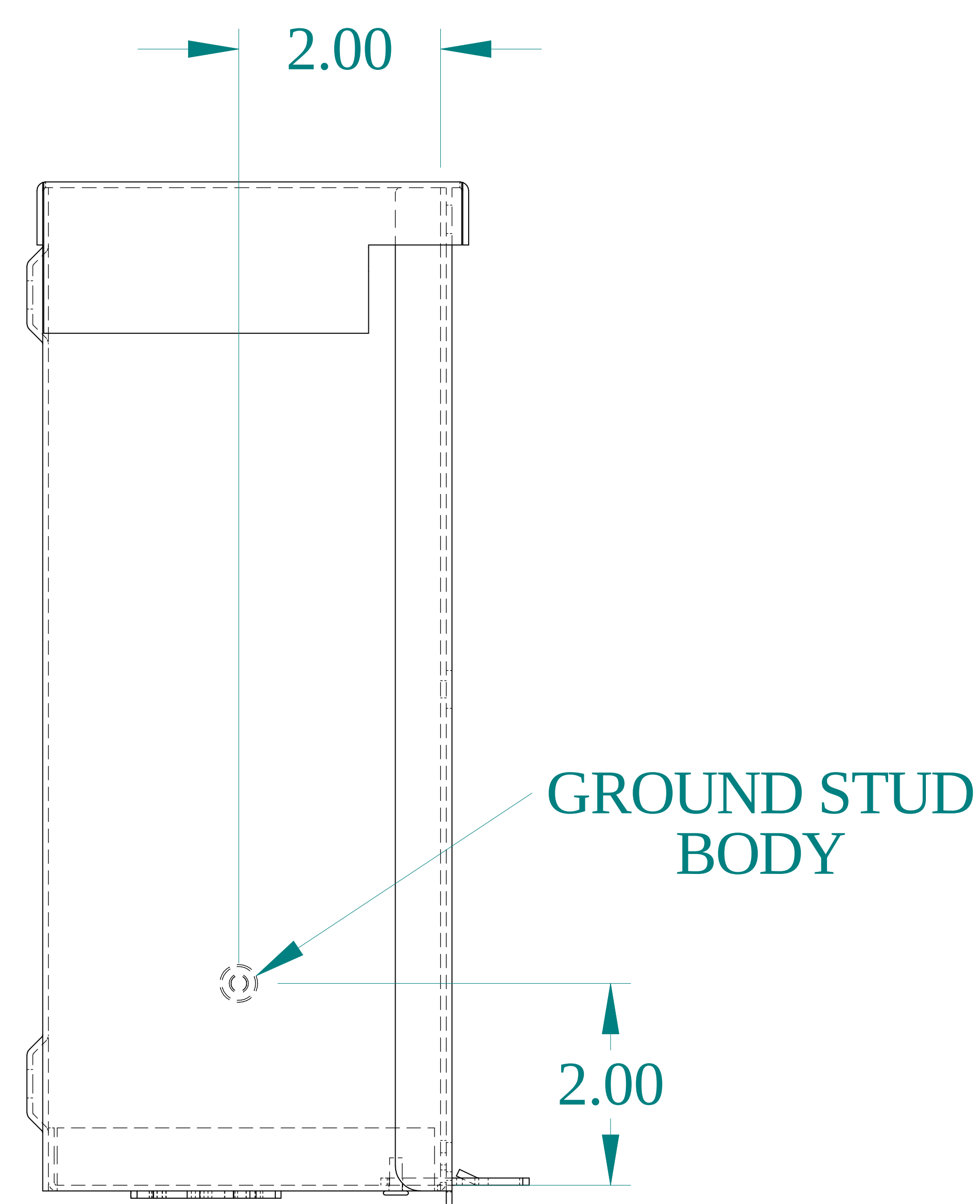
SIDE VIEW
