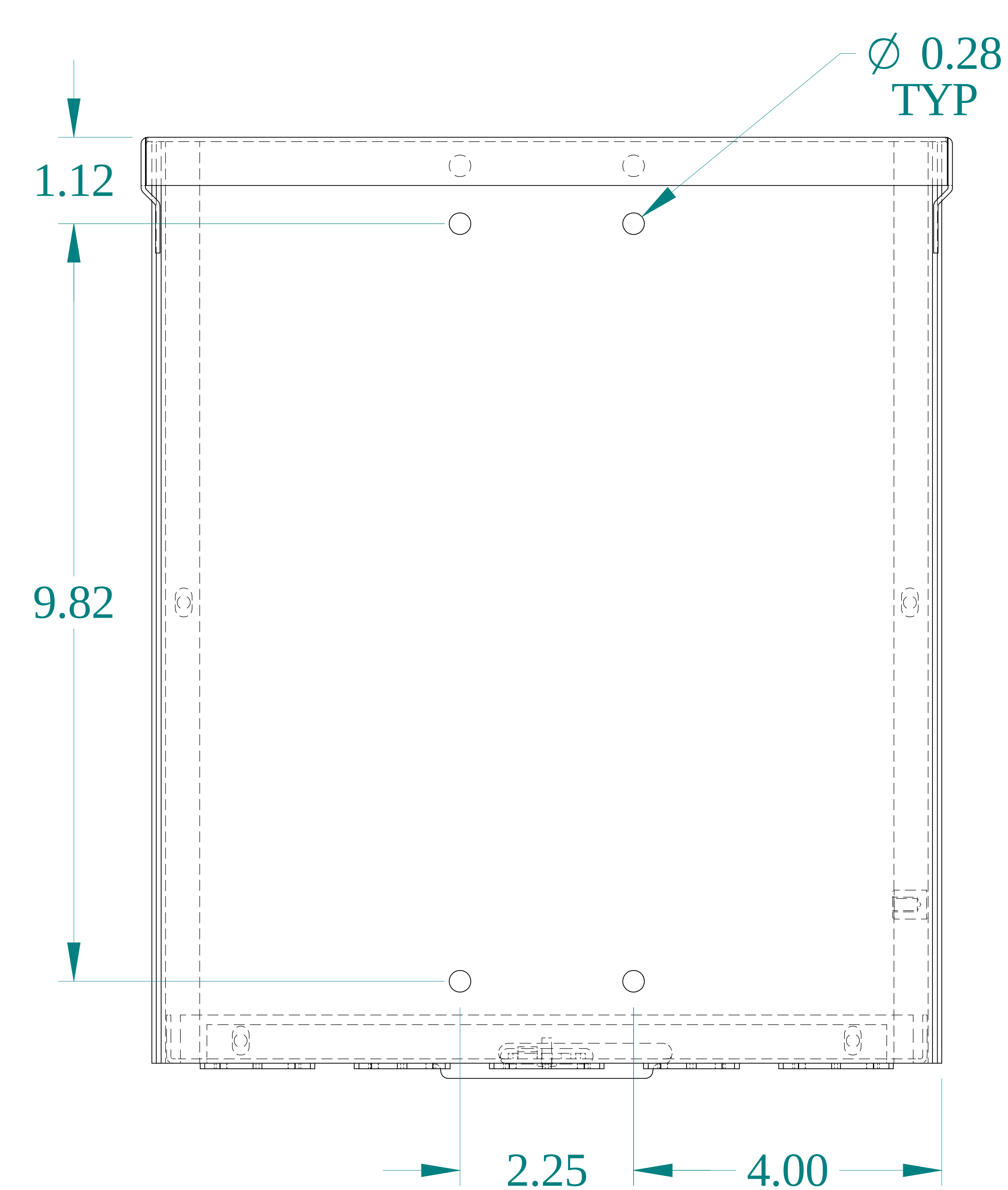
BACK VIEW
