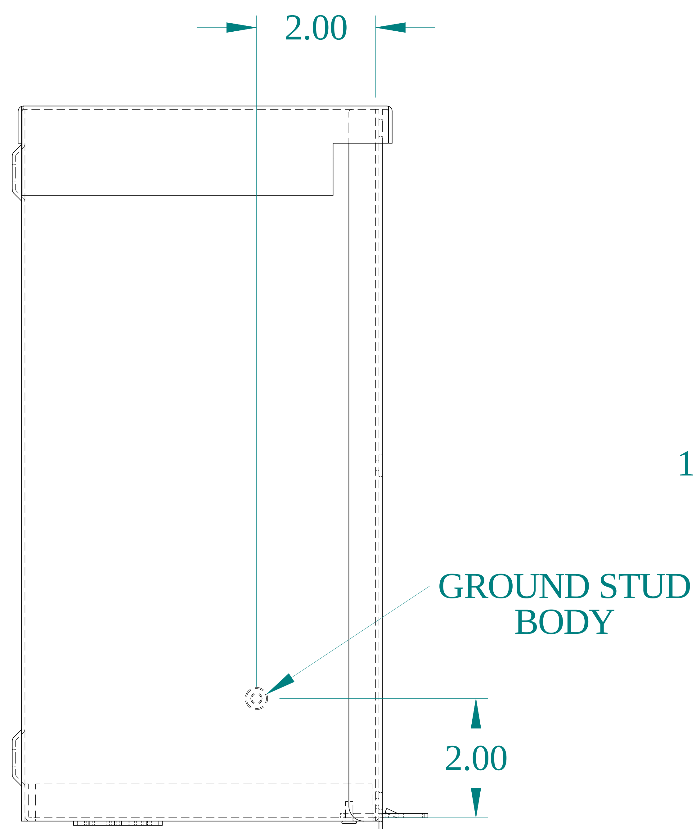
SIDE VIEW
