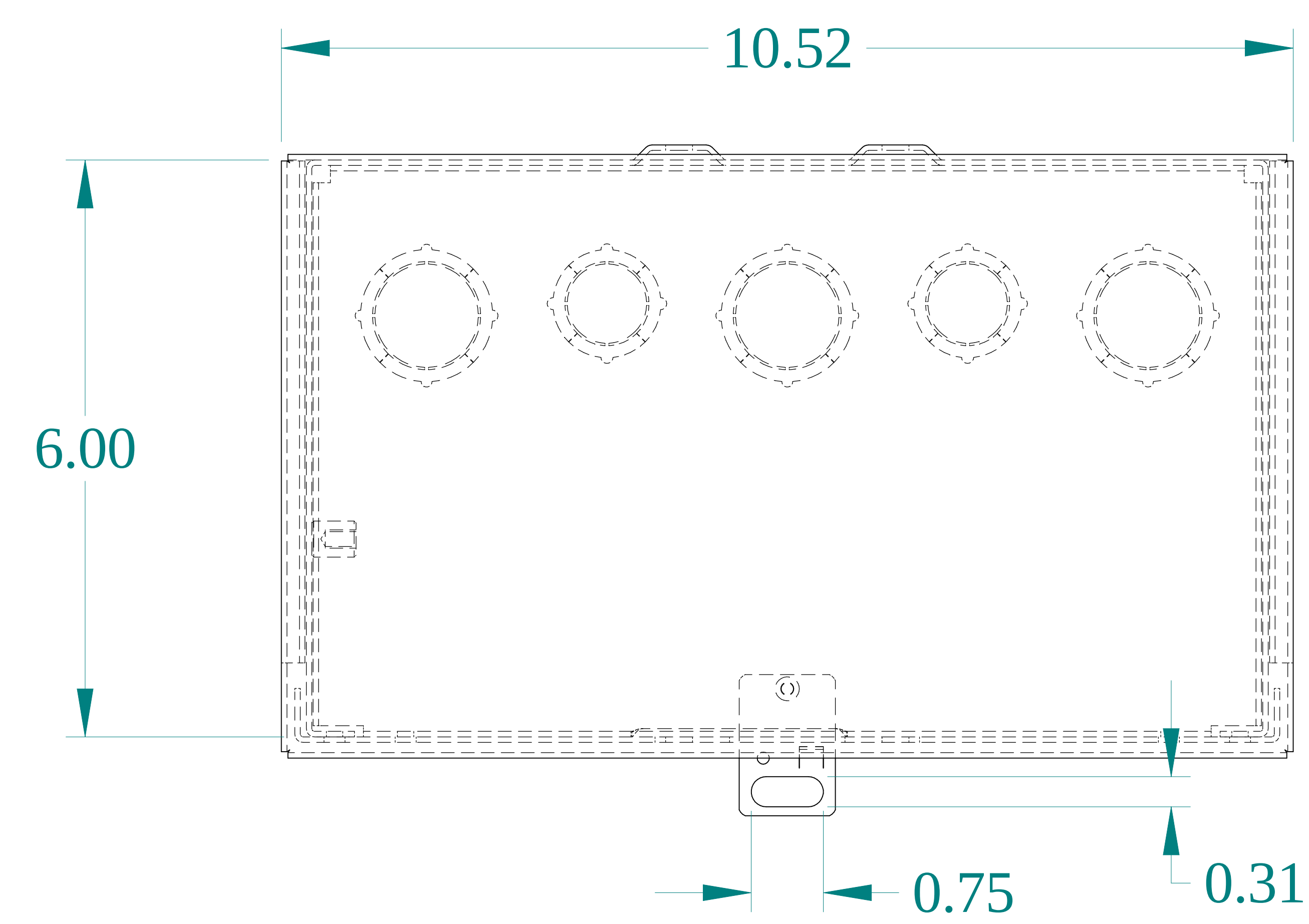
TOP VIEW
