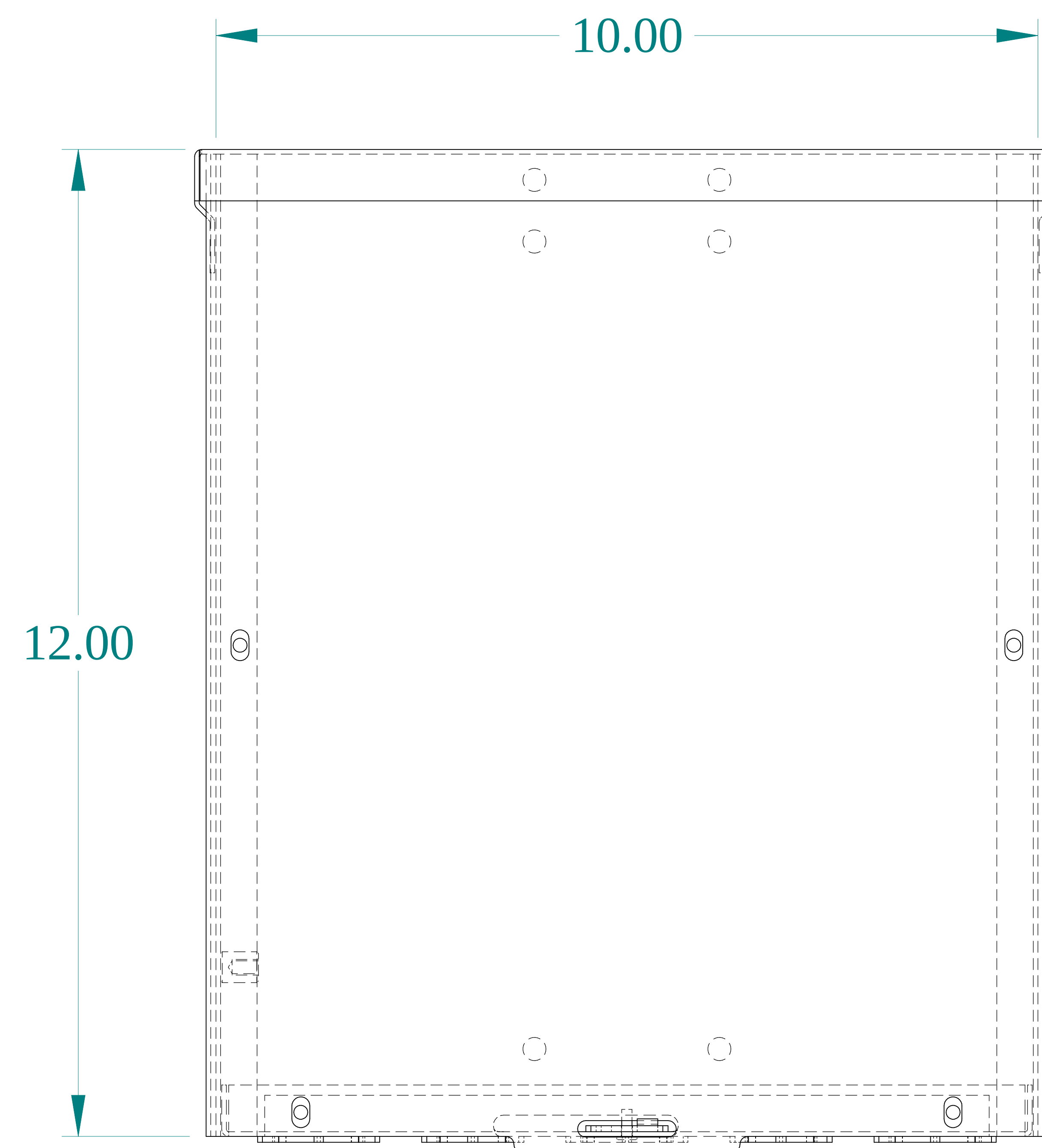
FRONT VIEW
