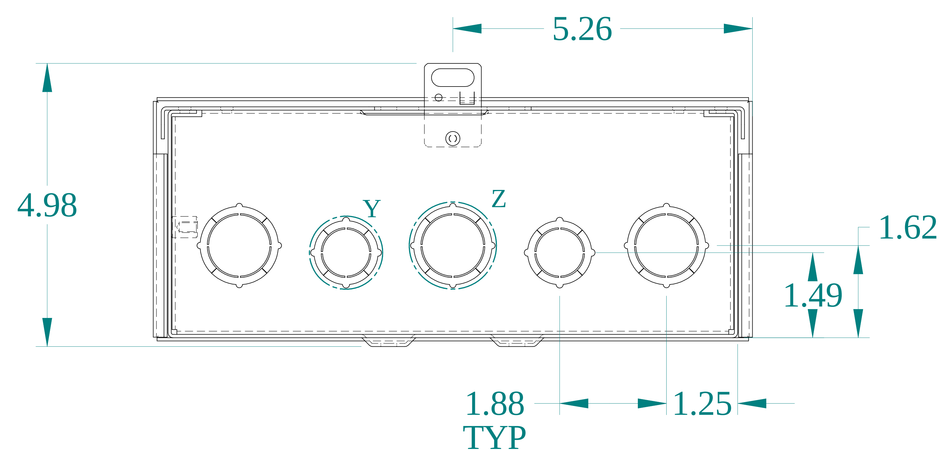
BOTTOM VIEW
