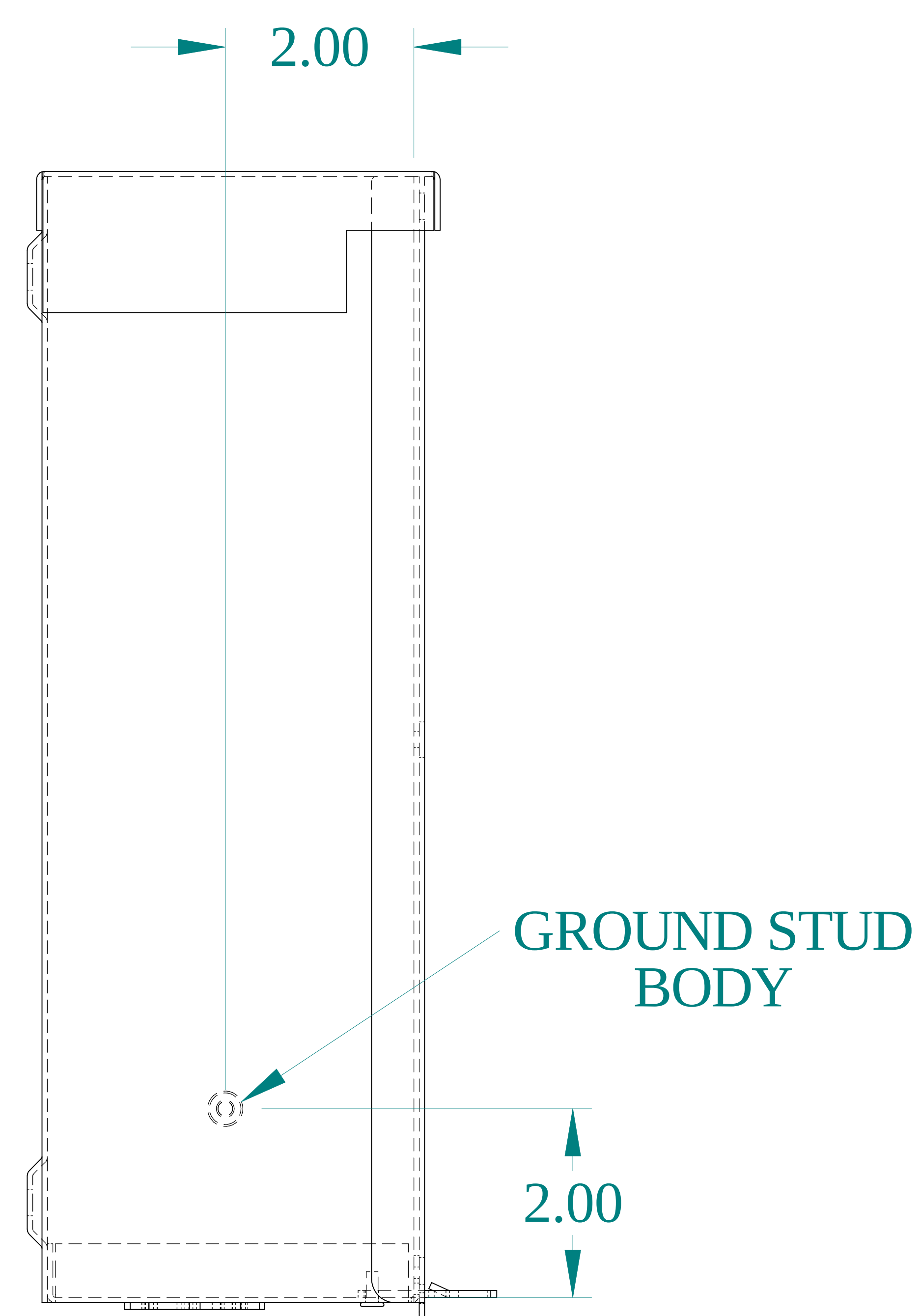
SIDE VIEW
