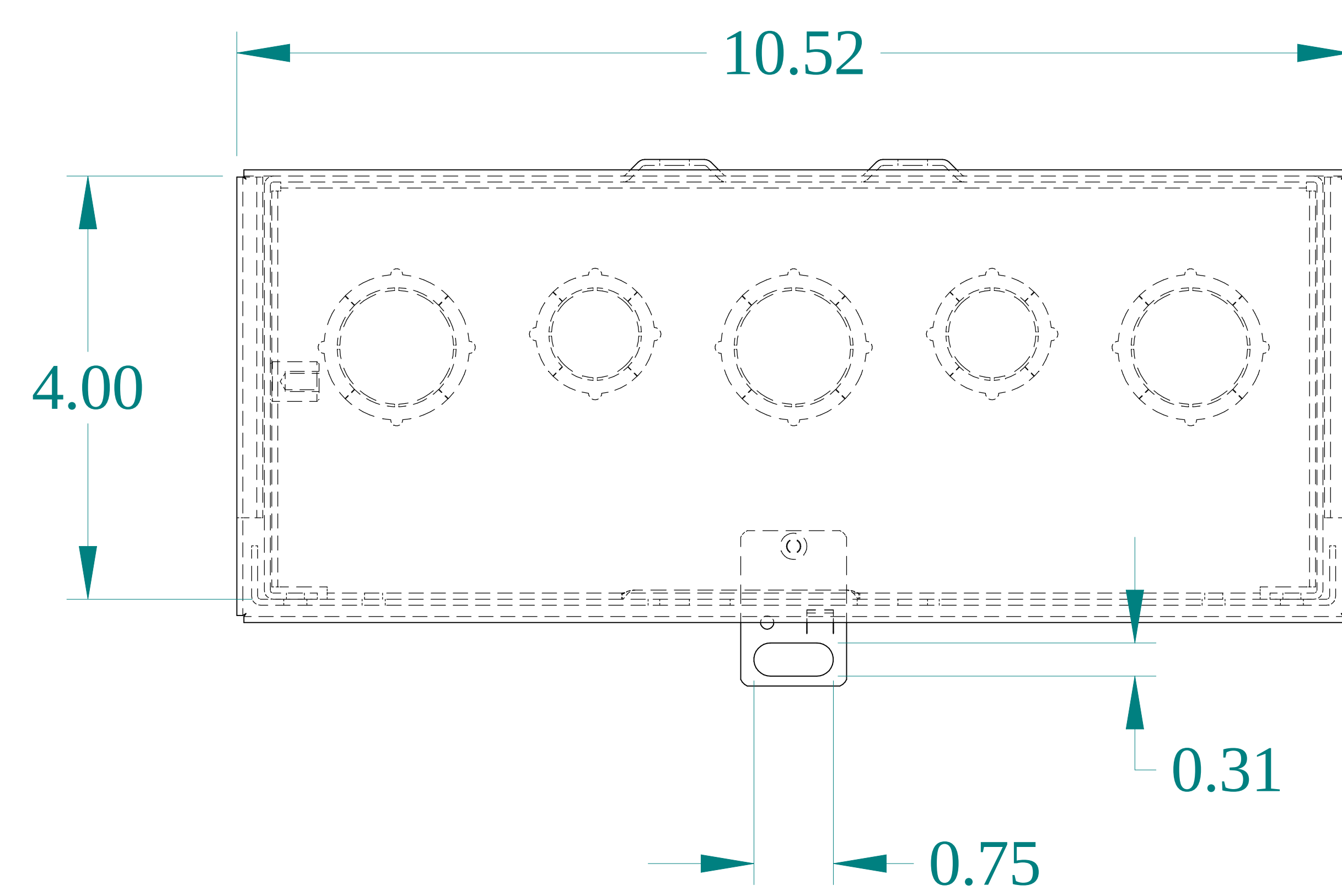
TOP VIEW
