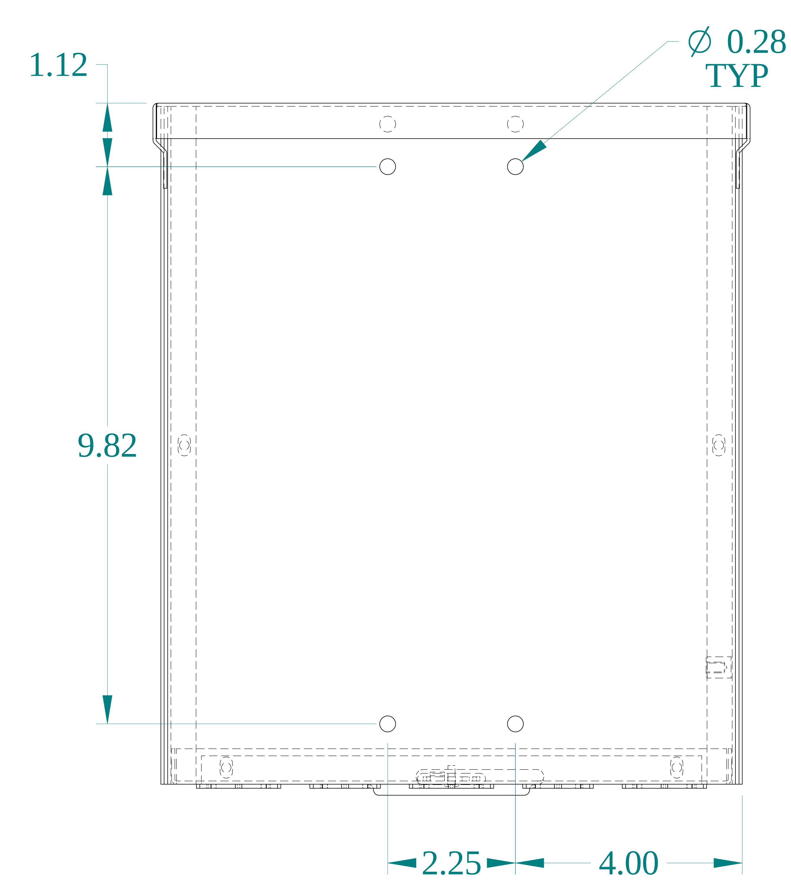
BACK VIEW
