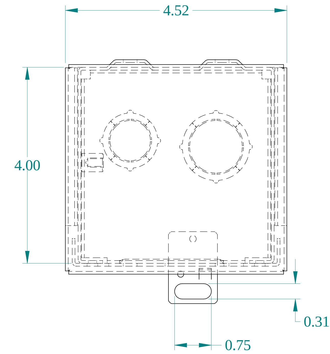
TOP VIEW
