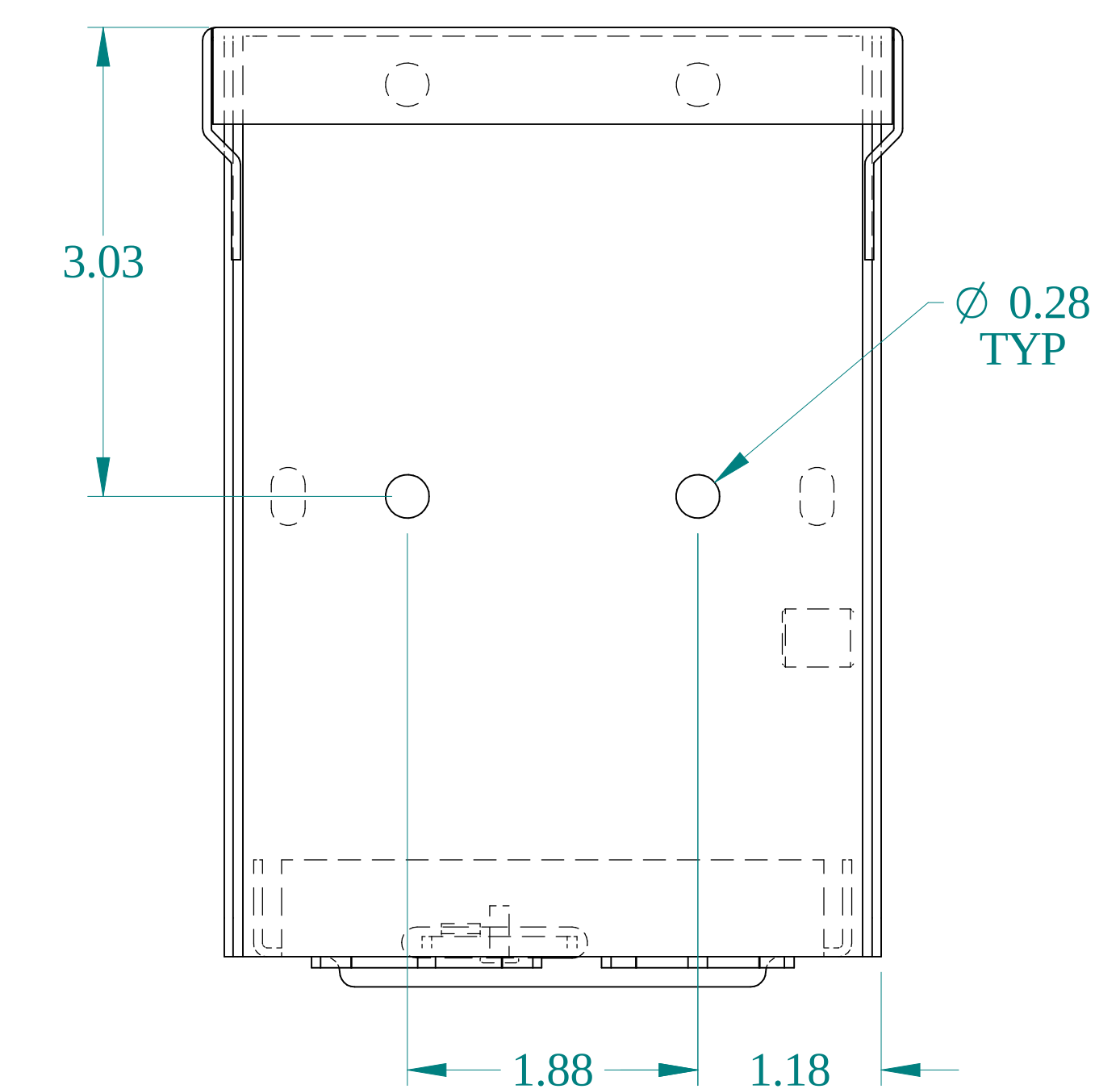
BACK VIEW
