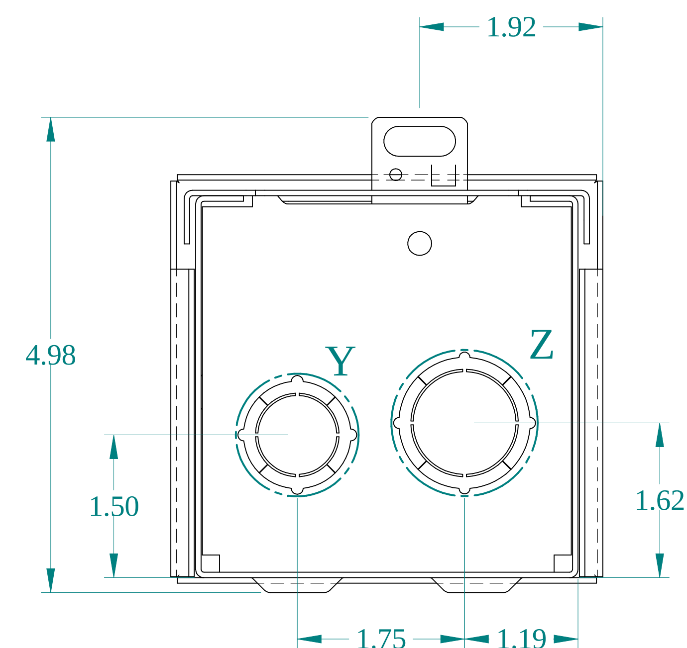
BOTTOM VIEW
