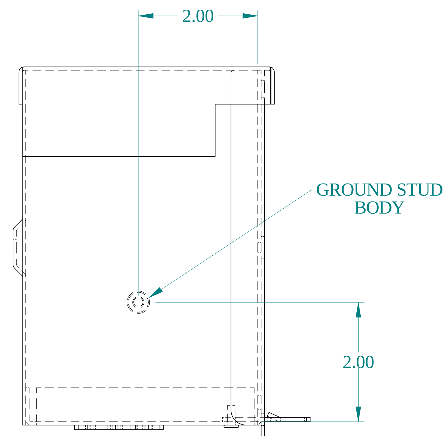
SIDE VIEW
