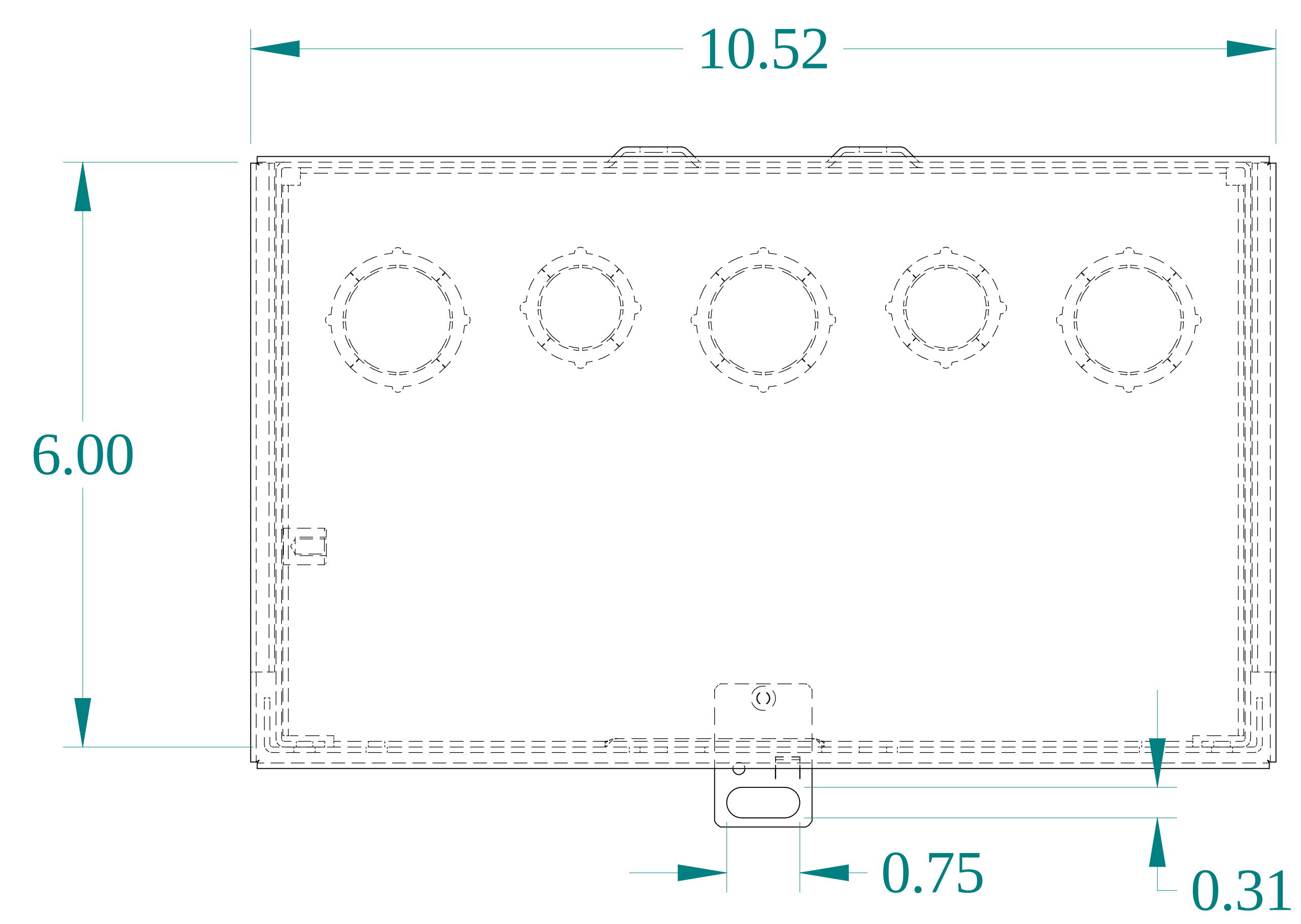
TOP VIEW
