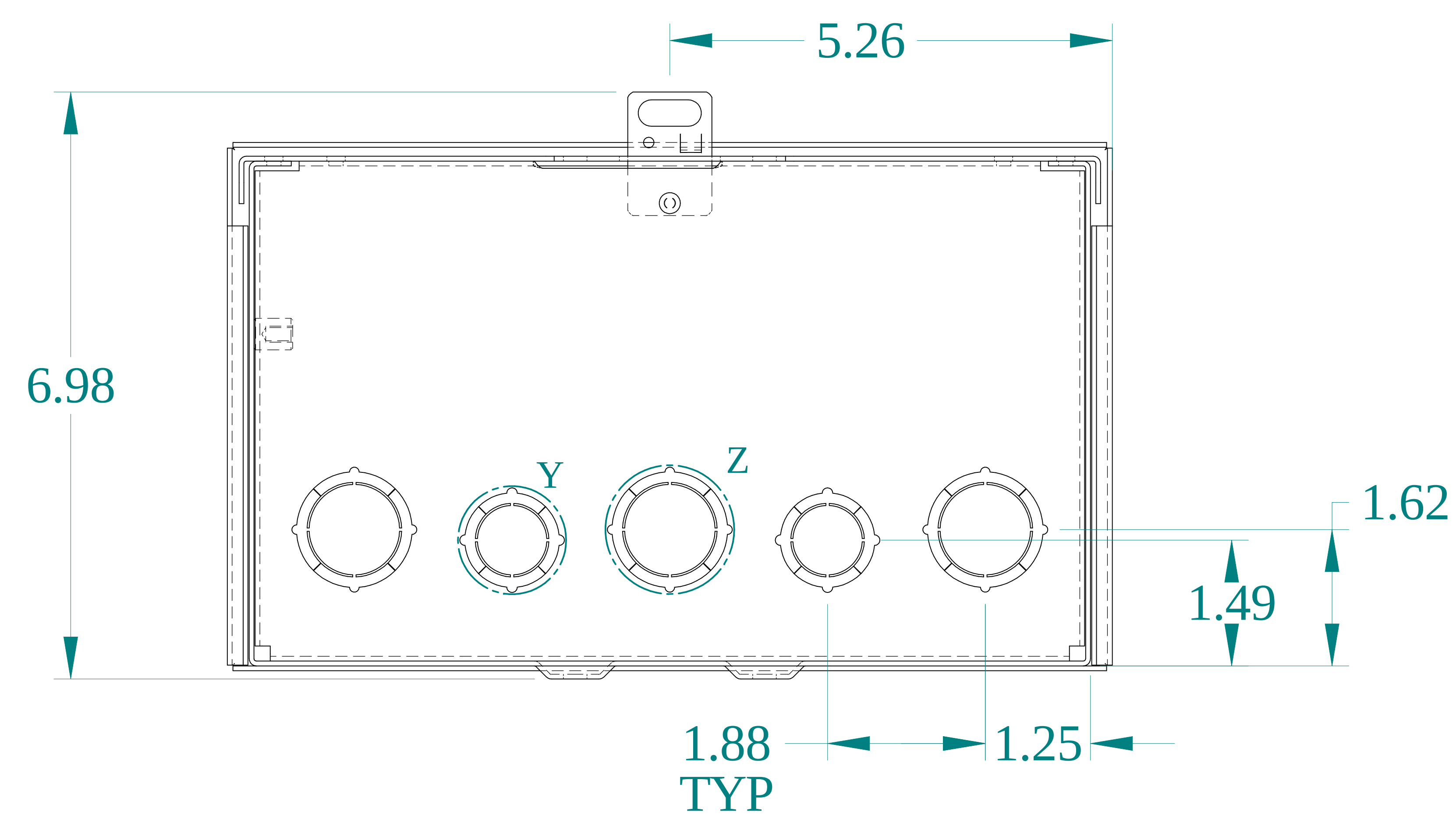
BOTTOM VIEW
