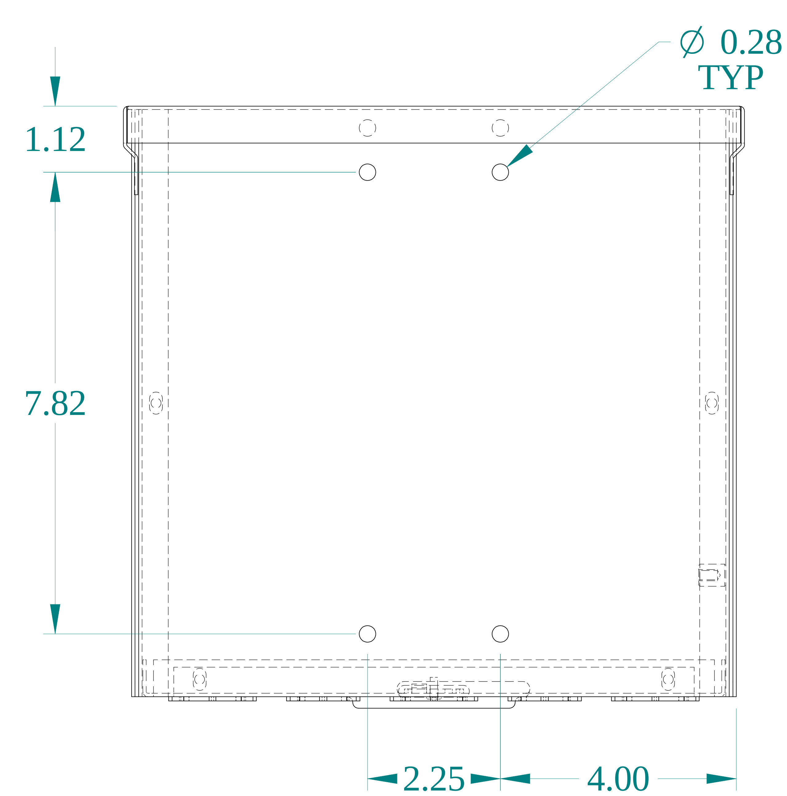
BACK VIEW
