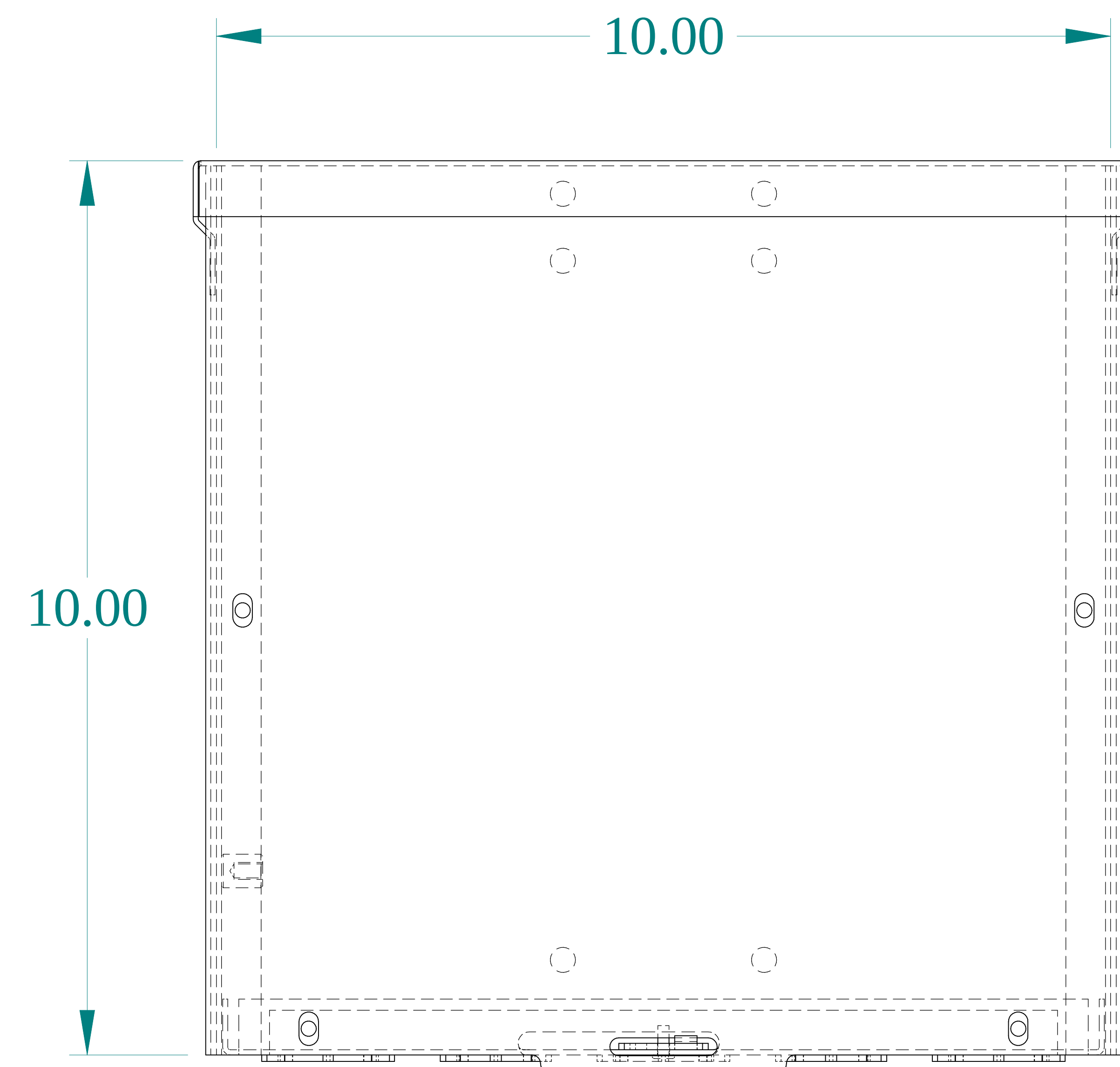
FRONT VIEW
