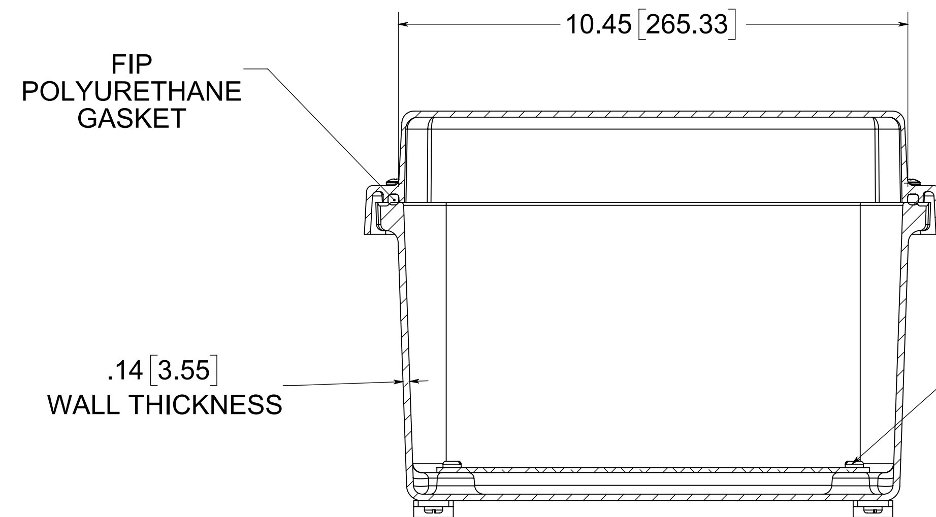
SECTION B-B
