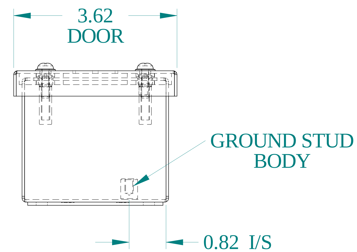
BOTTOM VIEW
