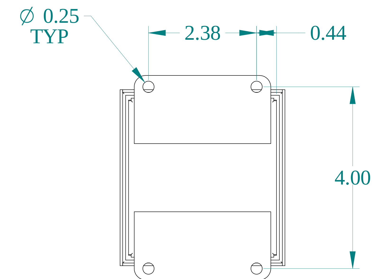
BACK VIEW
