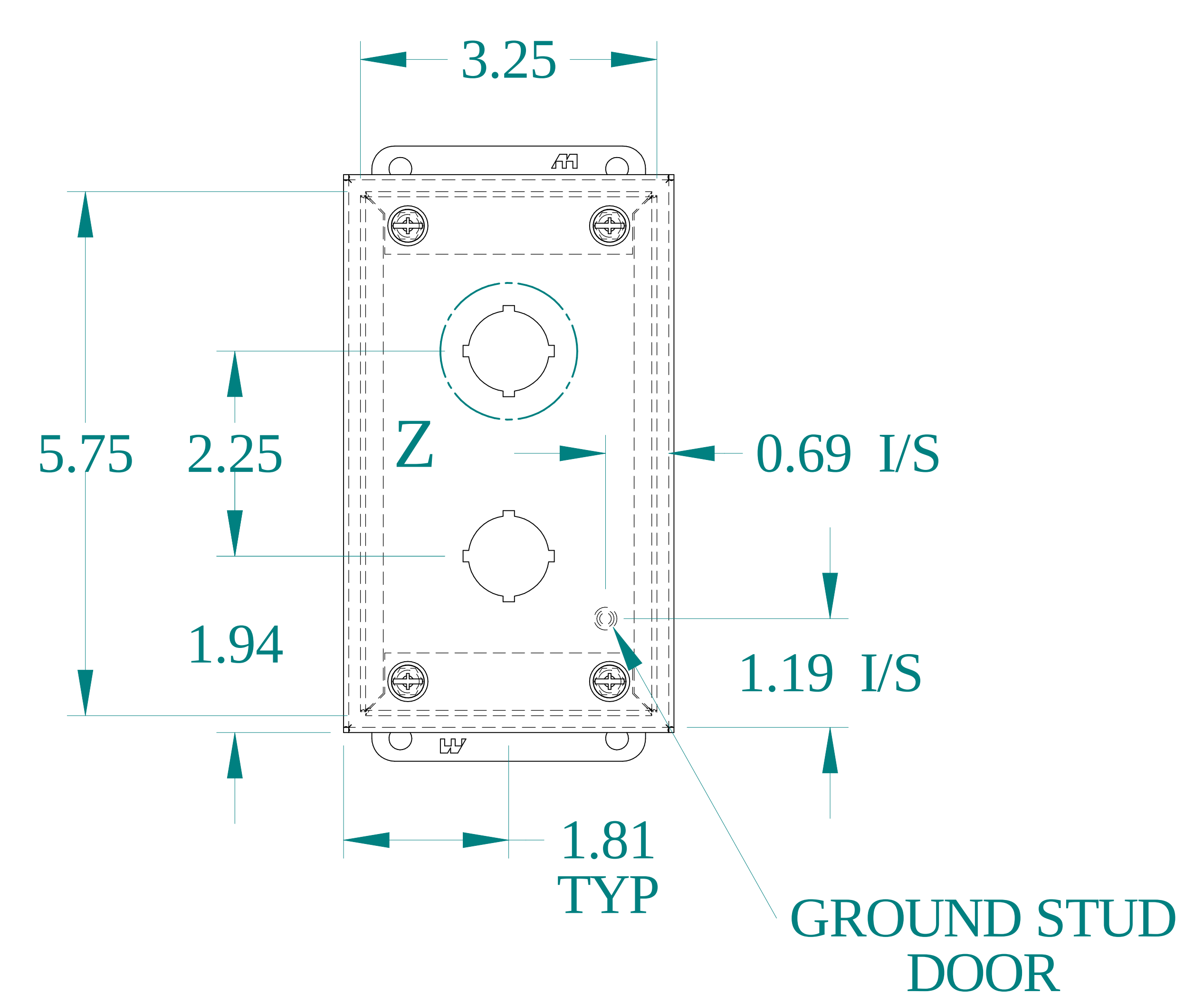
FRONT VIEW
