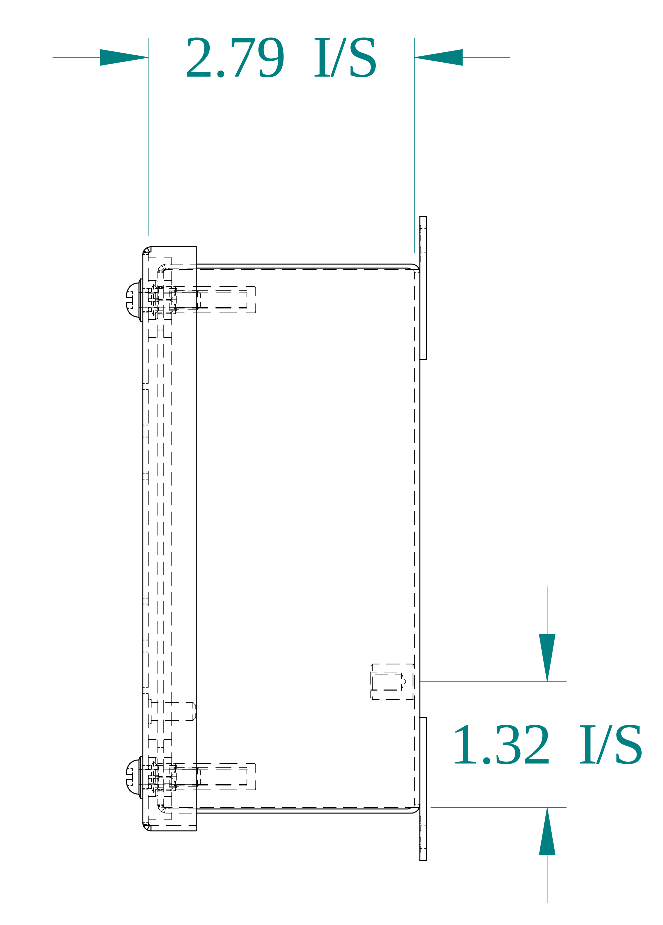
SIDE VIEW
