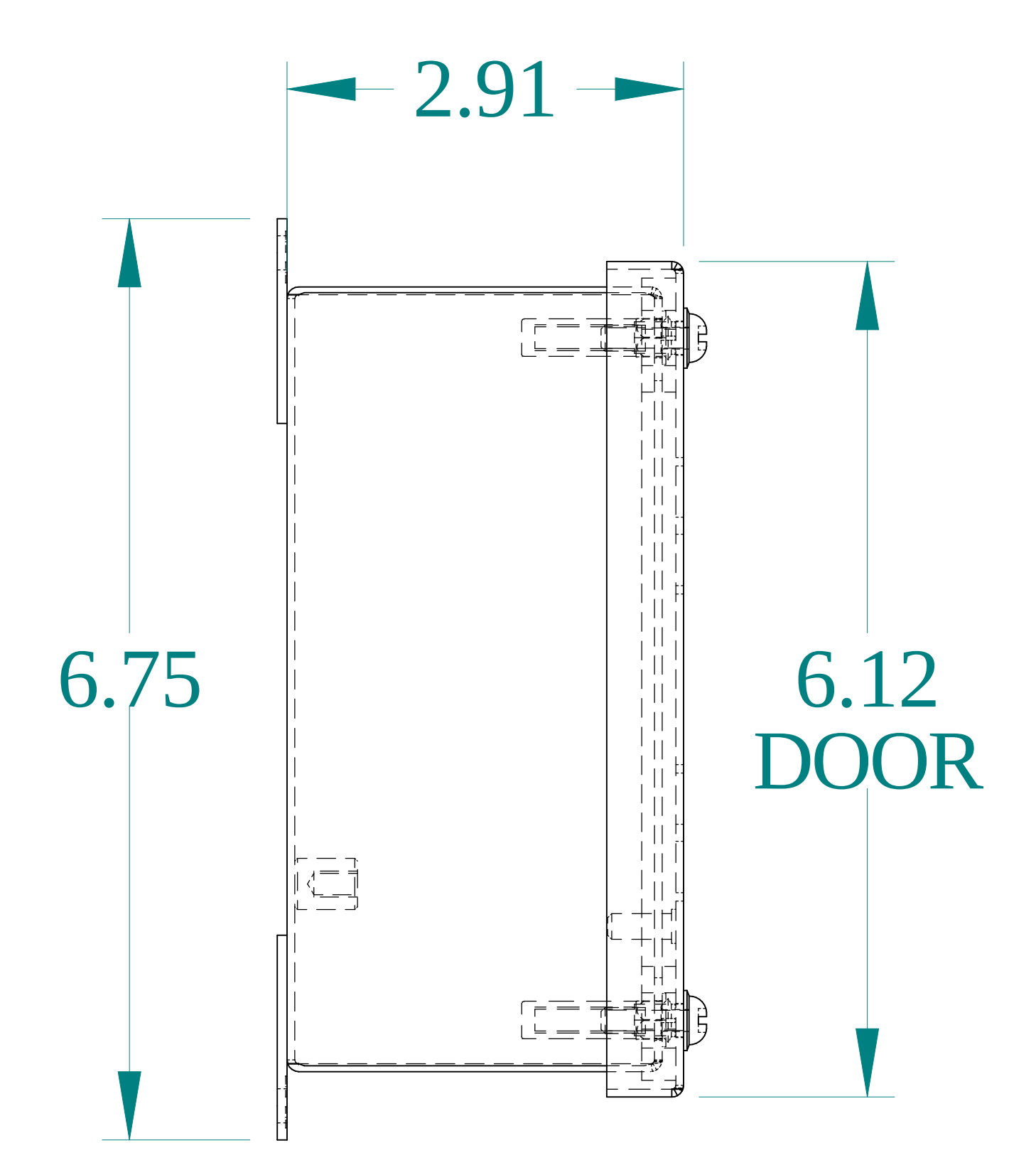
SIDE VIEW
