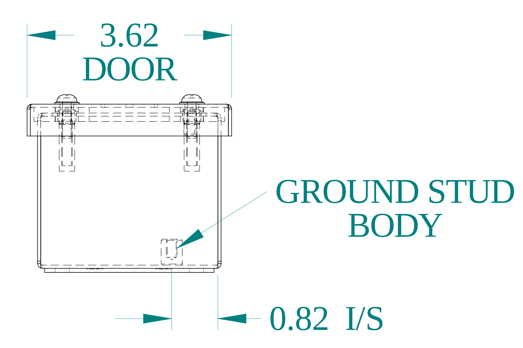
BOTTOM VIEW
