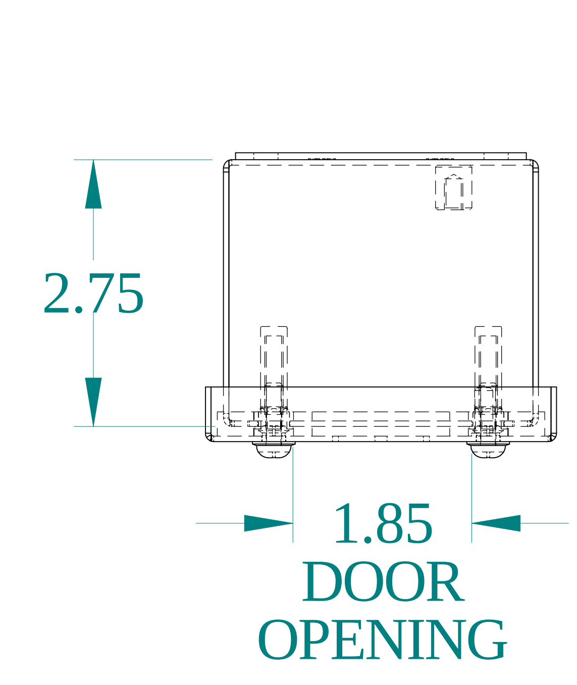
TOP VIEW
