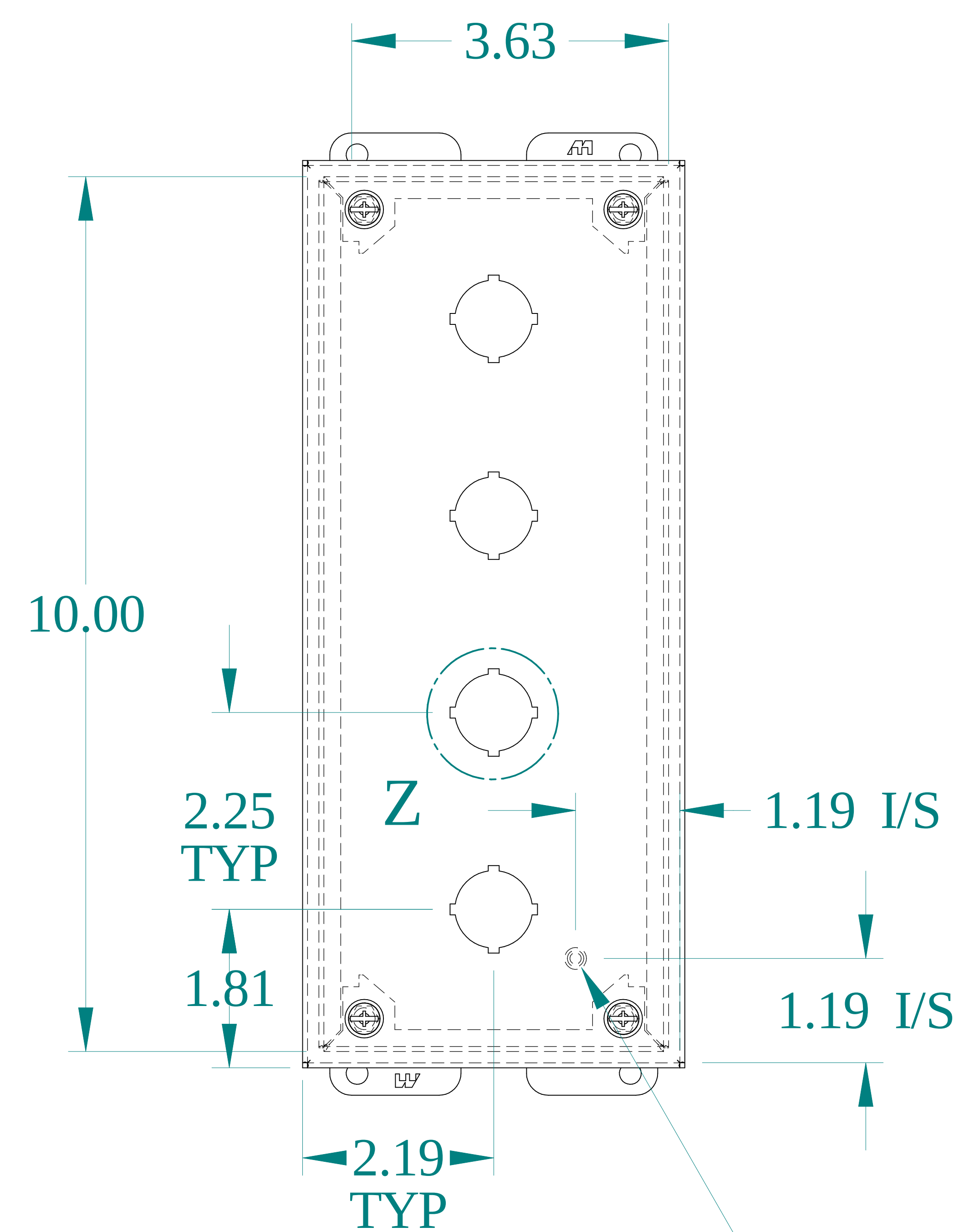
FRONT VIEW
