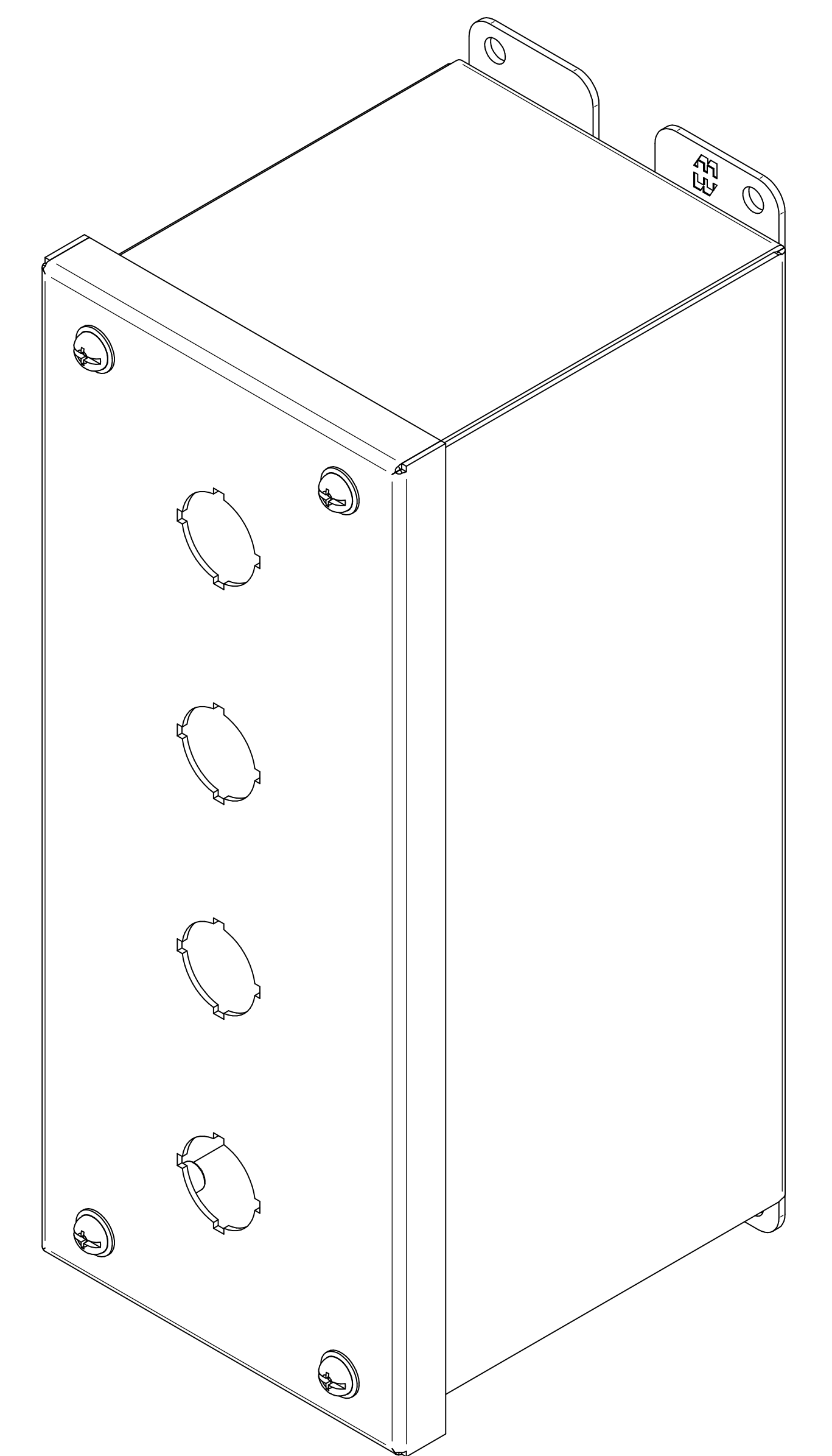
ISOMETRIC VIEWS
