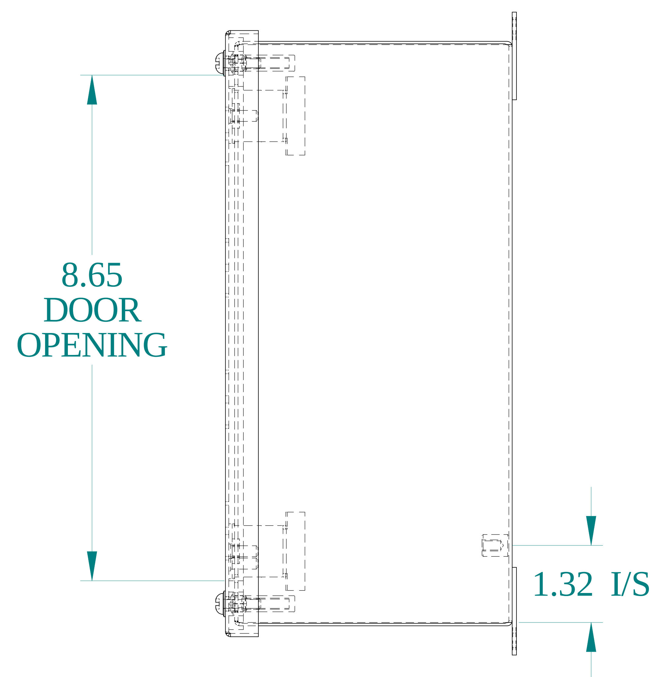
SIDE VIEW
