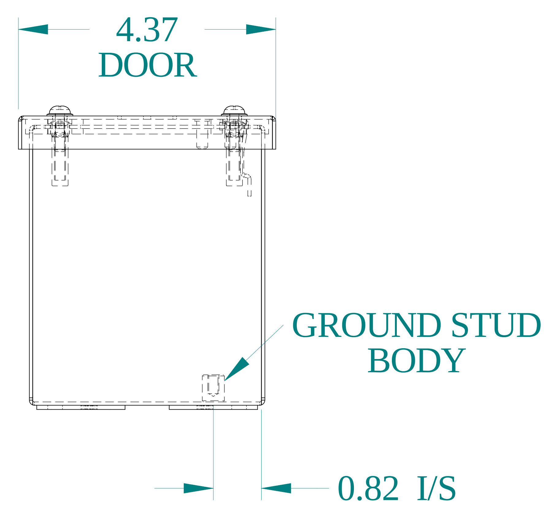
BOTTOM VIEW
