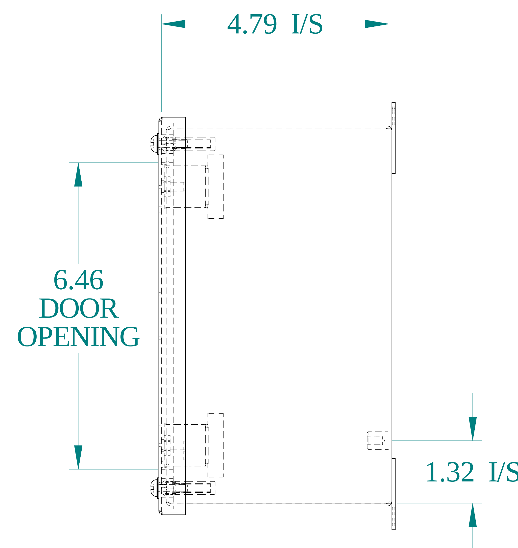
SIDE VIEW
