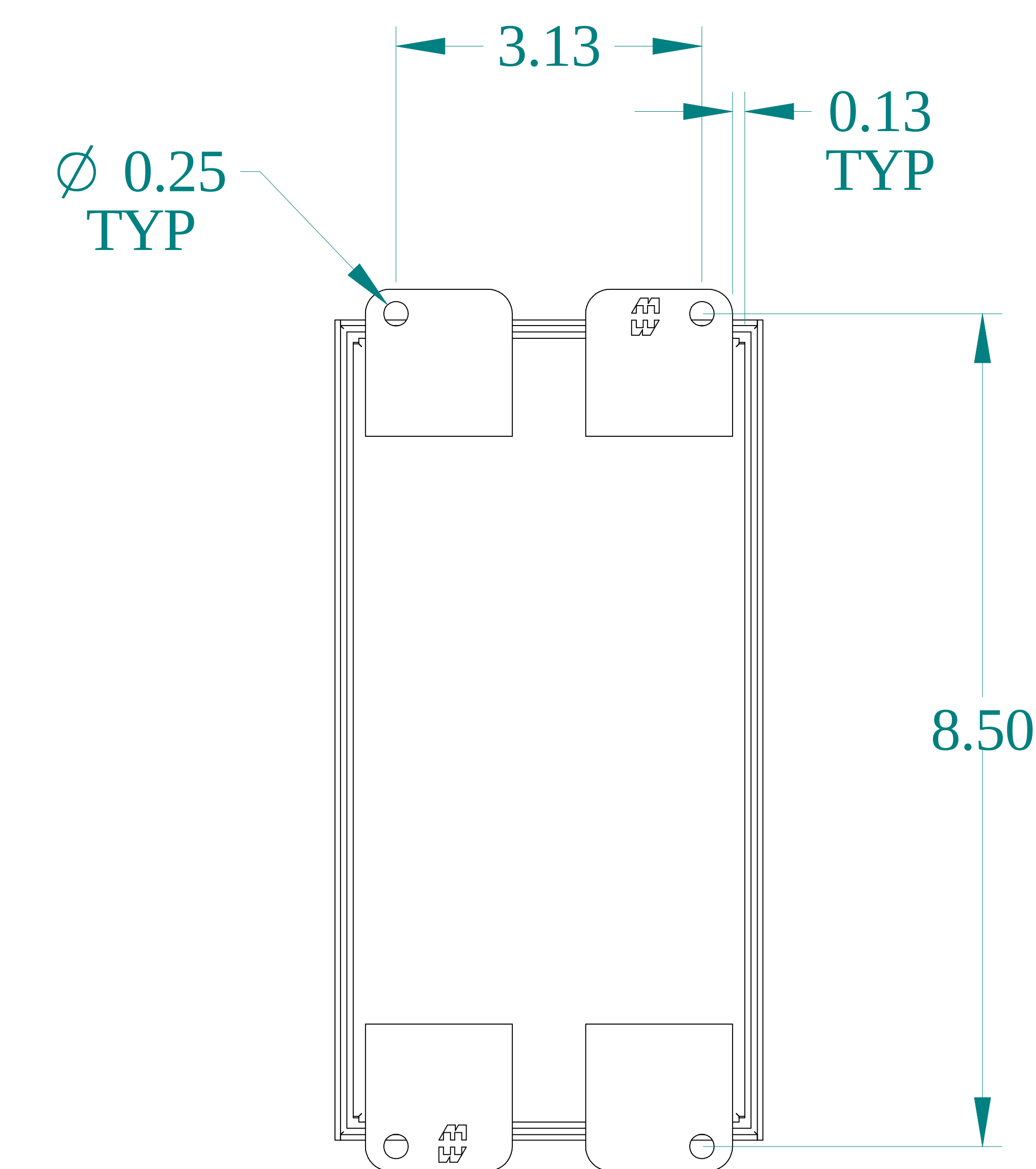
BACK VIEW
