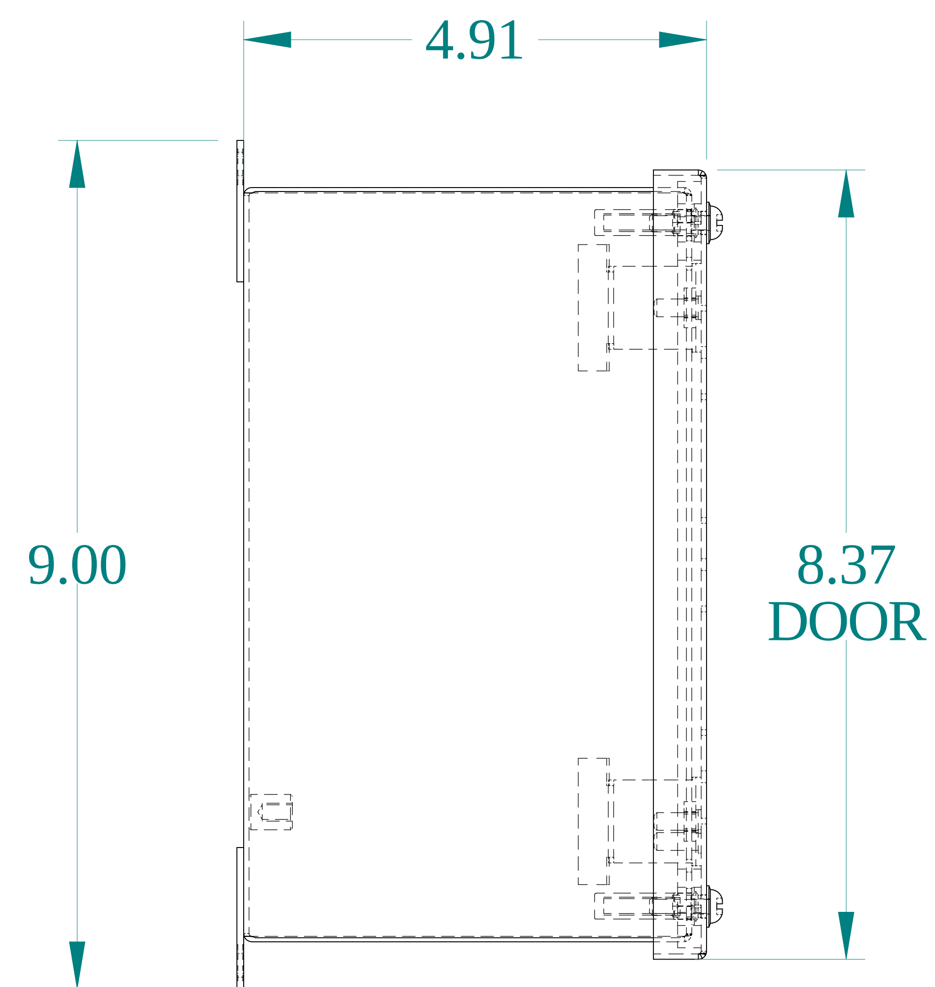
SIDE VIEW
