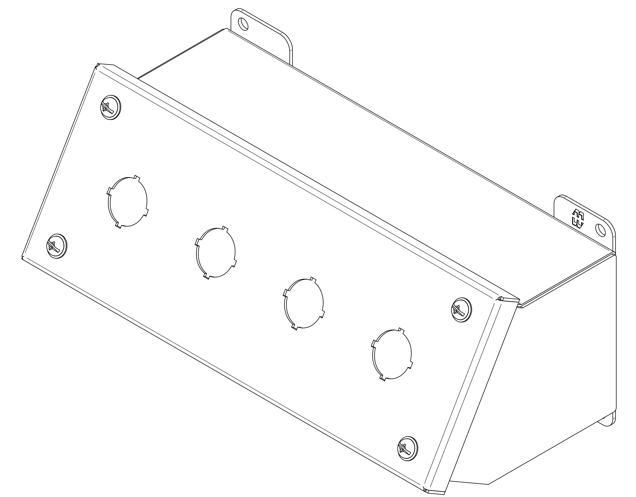
ISOMETRIC VIEWS
