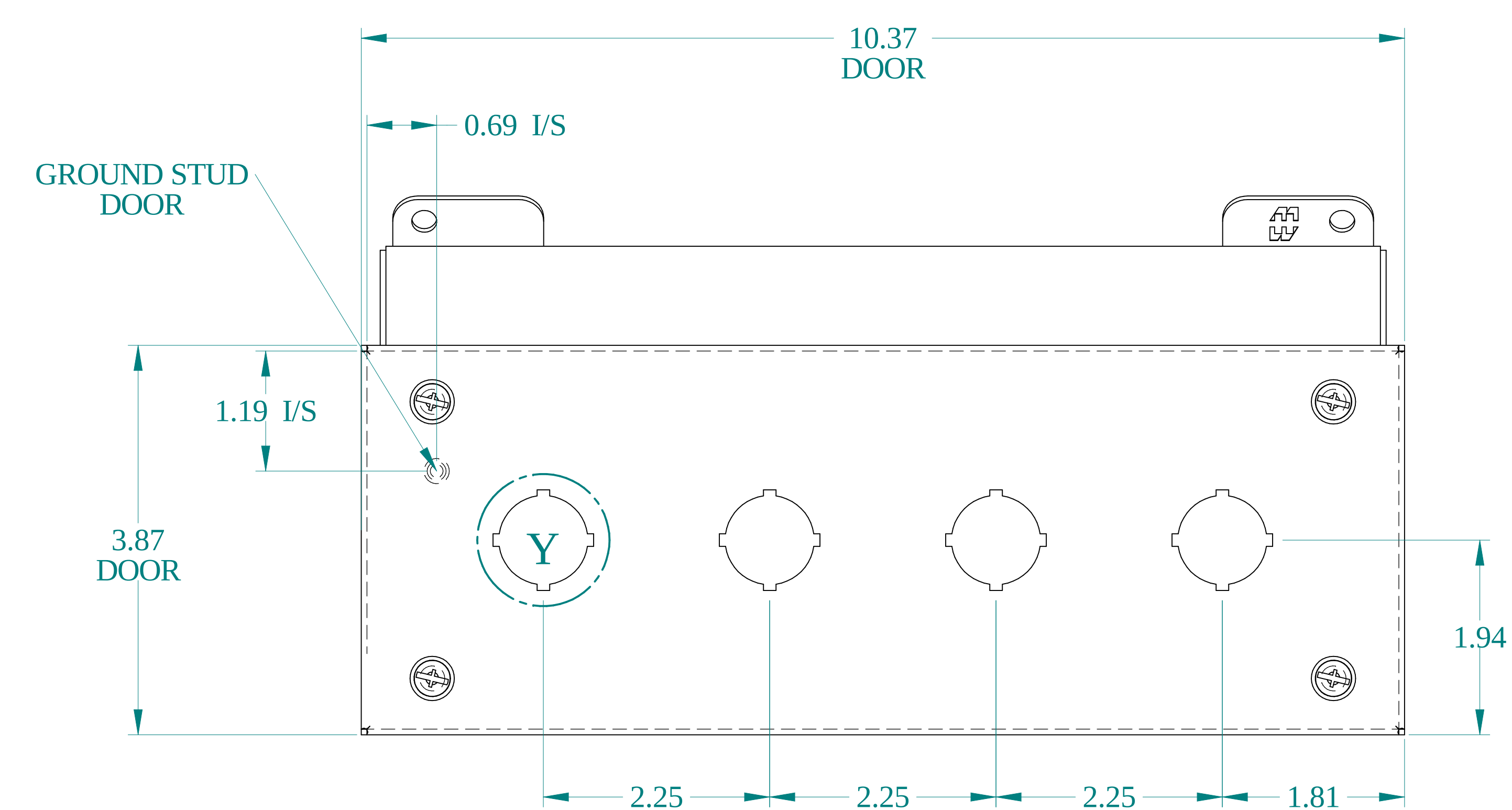
VIEW Z-Z
