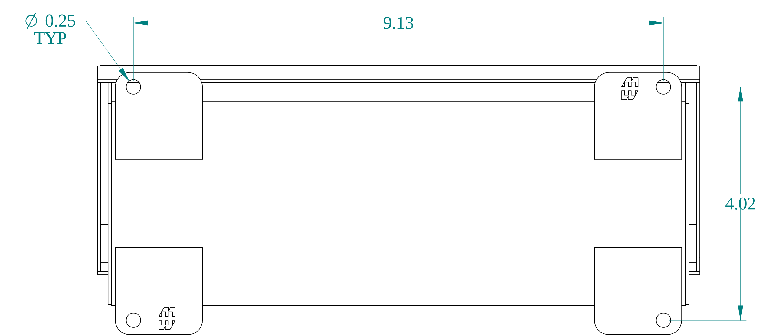
BACK VIEW
