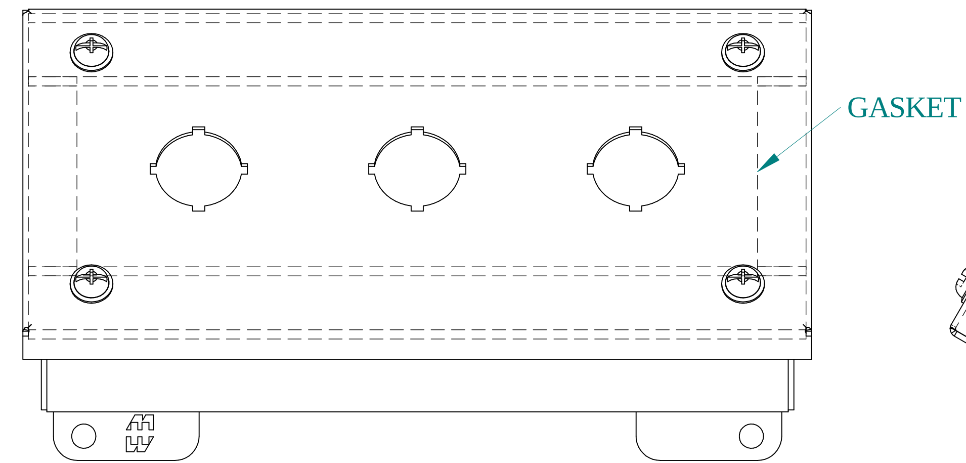
FRONT VIEW
