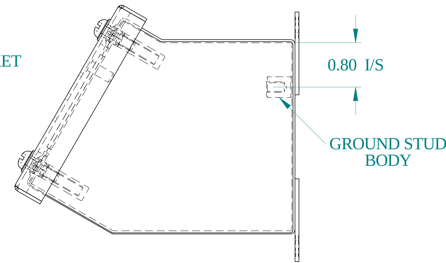
SIDE VIEW
