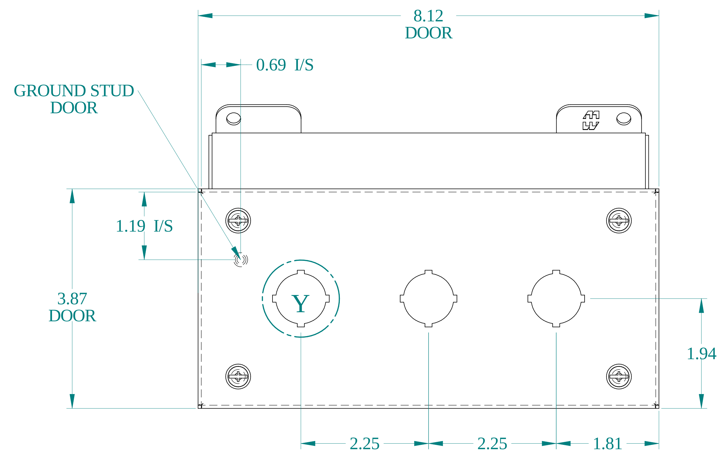
VIEW Z-Z
