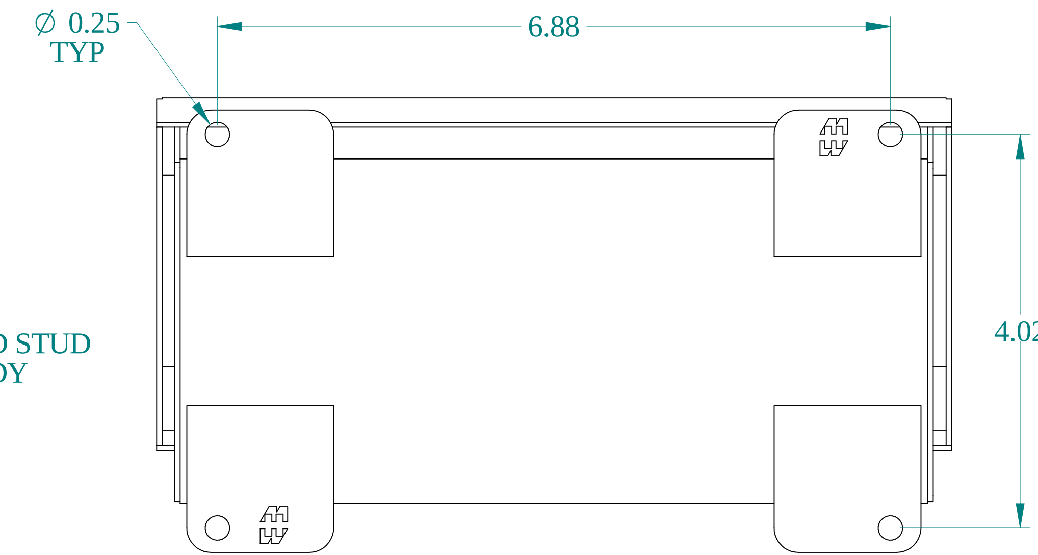
BACK VIEW
