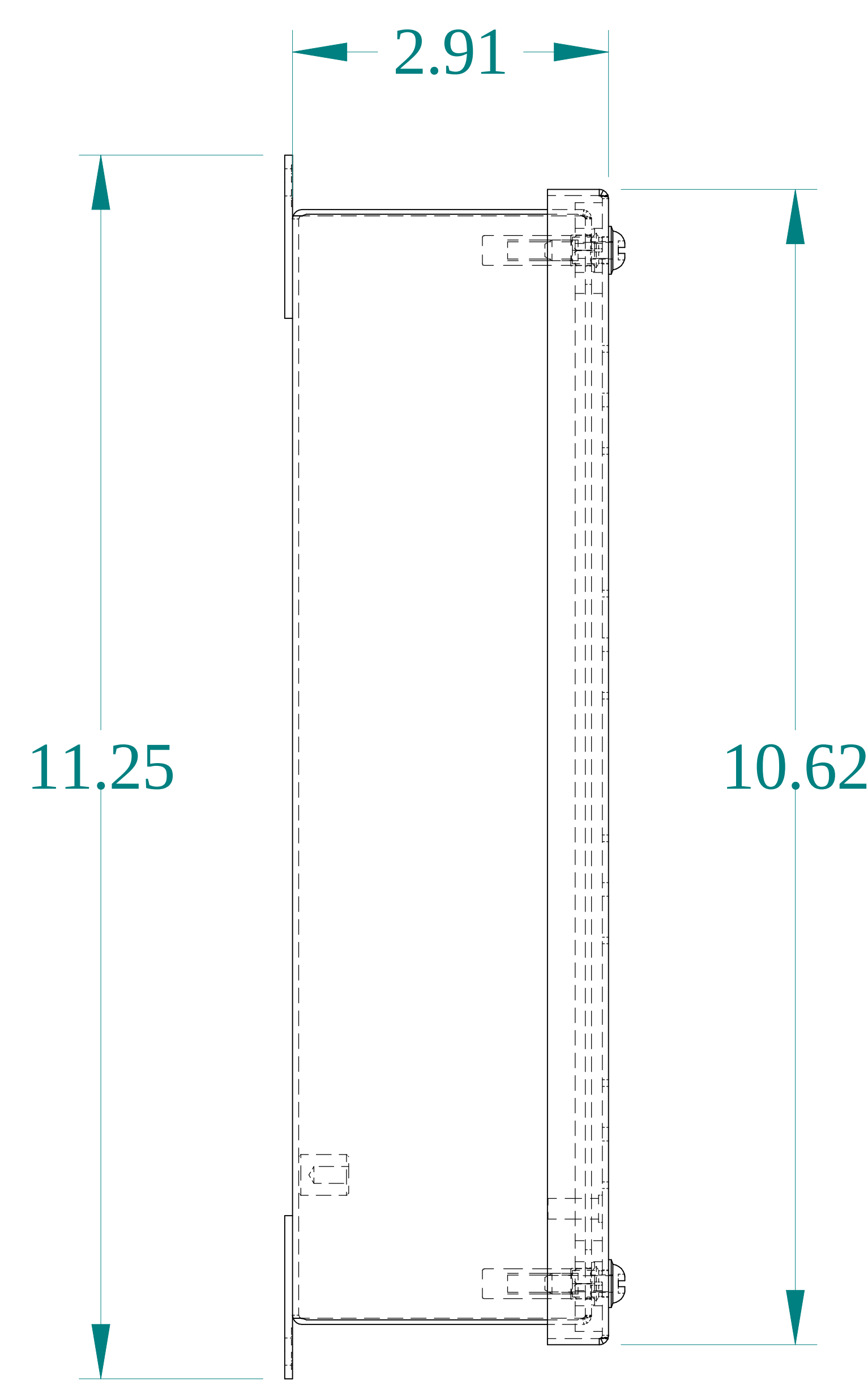
SIDE VIEW
