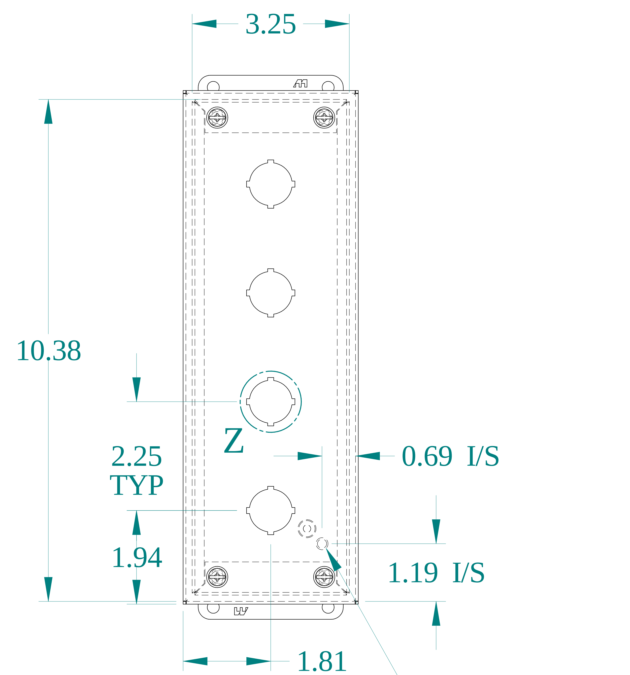
FRONT VIEW
