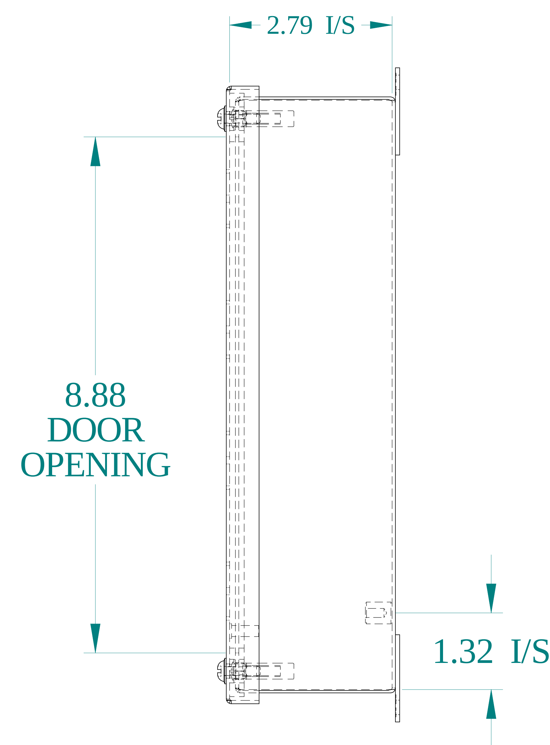
SIDE VIEW
