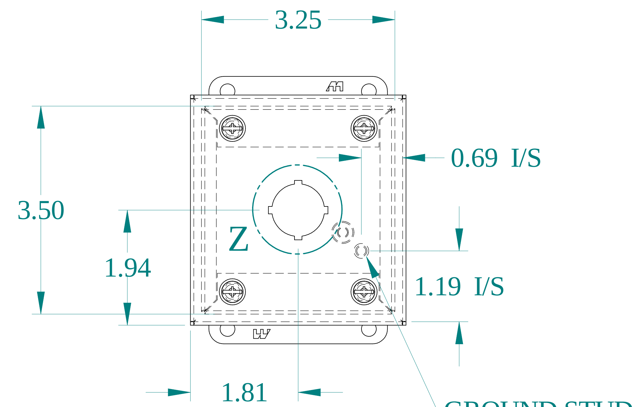
FRONT VIEW
