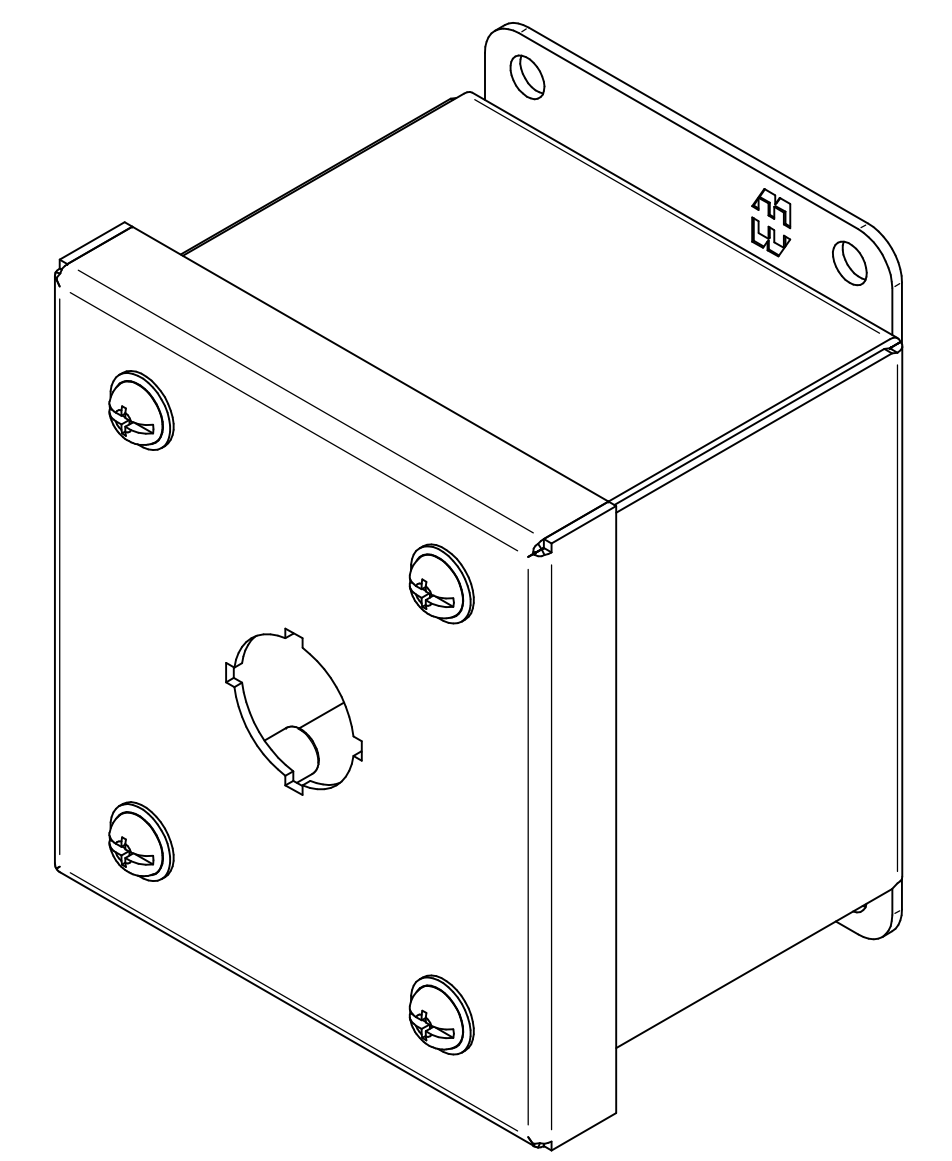
ISOMETRIC VIEWS
