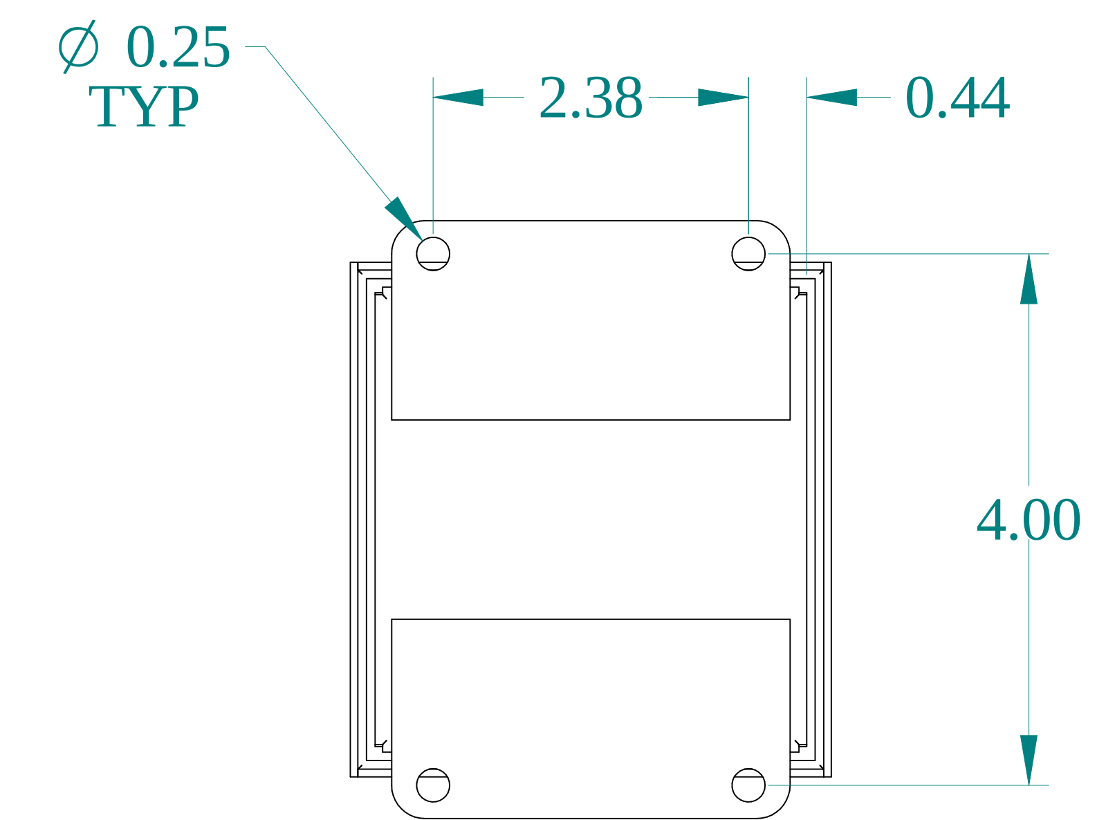
BACK VIEW
