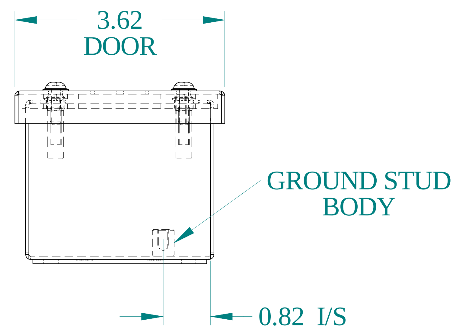
BOTTOM VIEW
