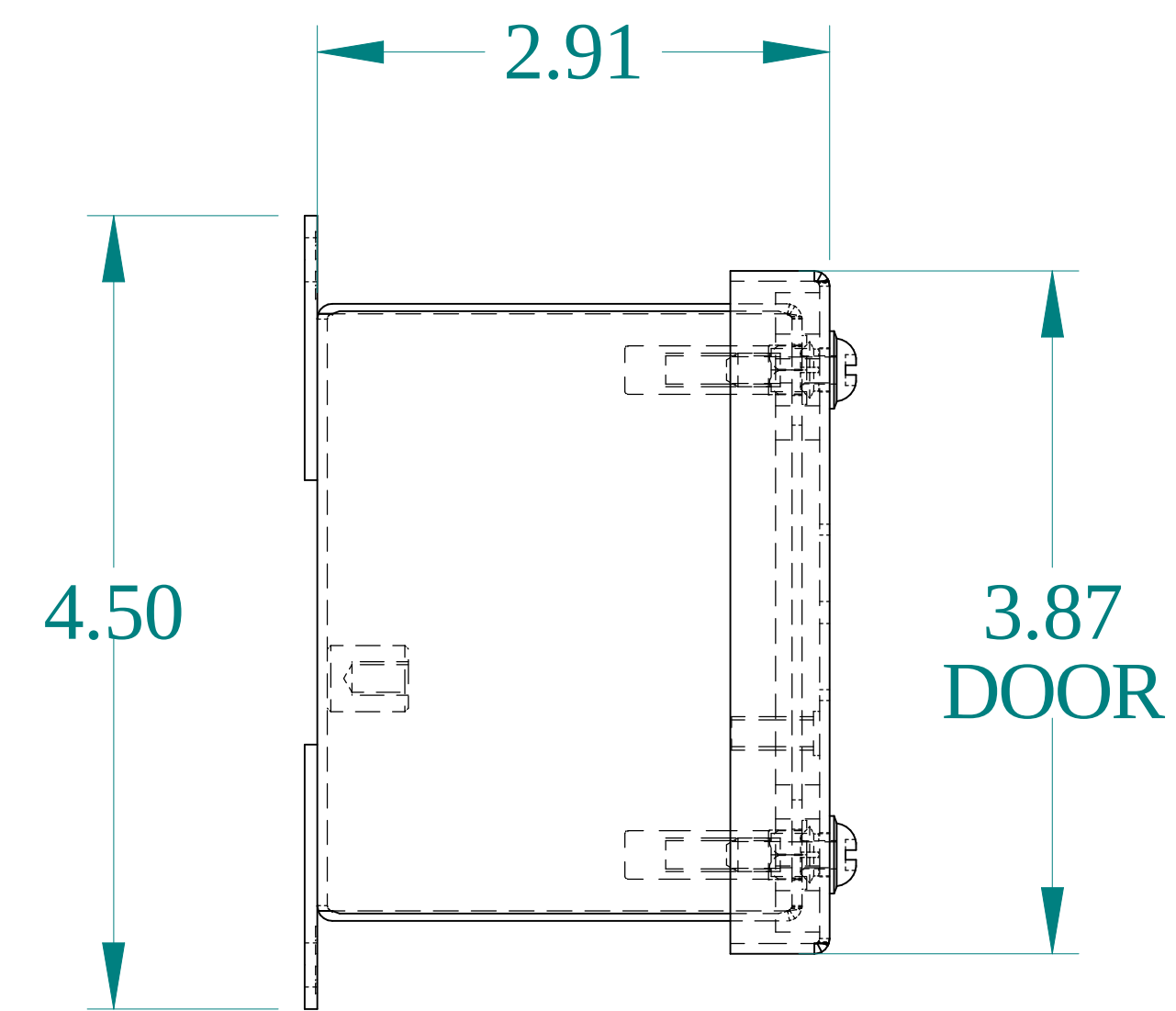
SIDE VIEW
