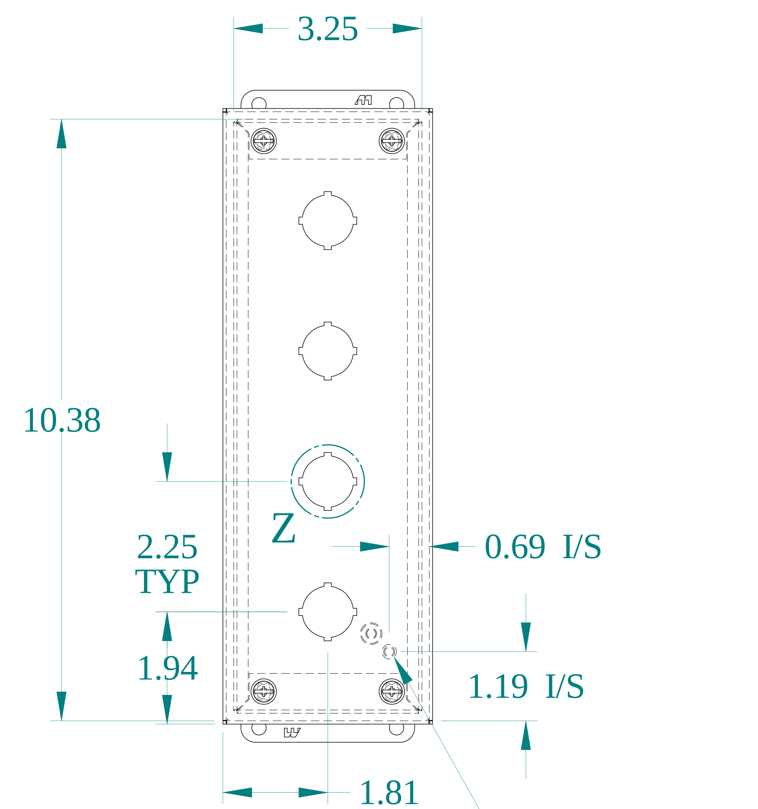
FRONT VIEW
