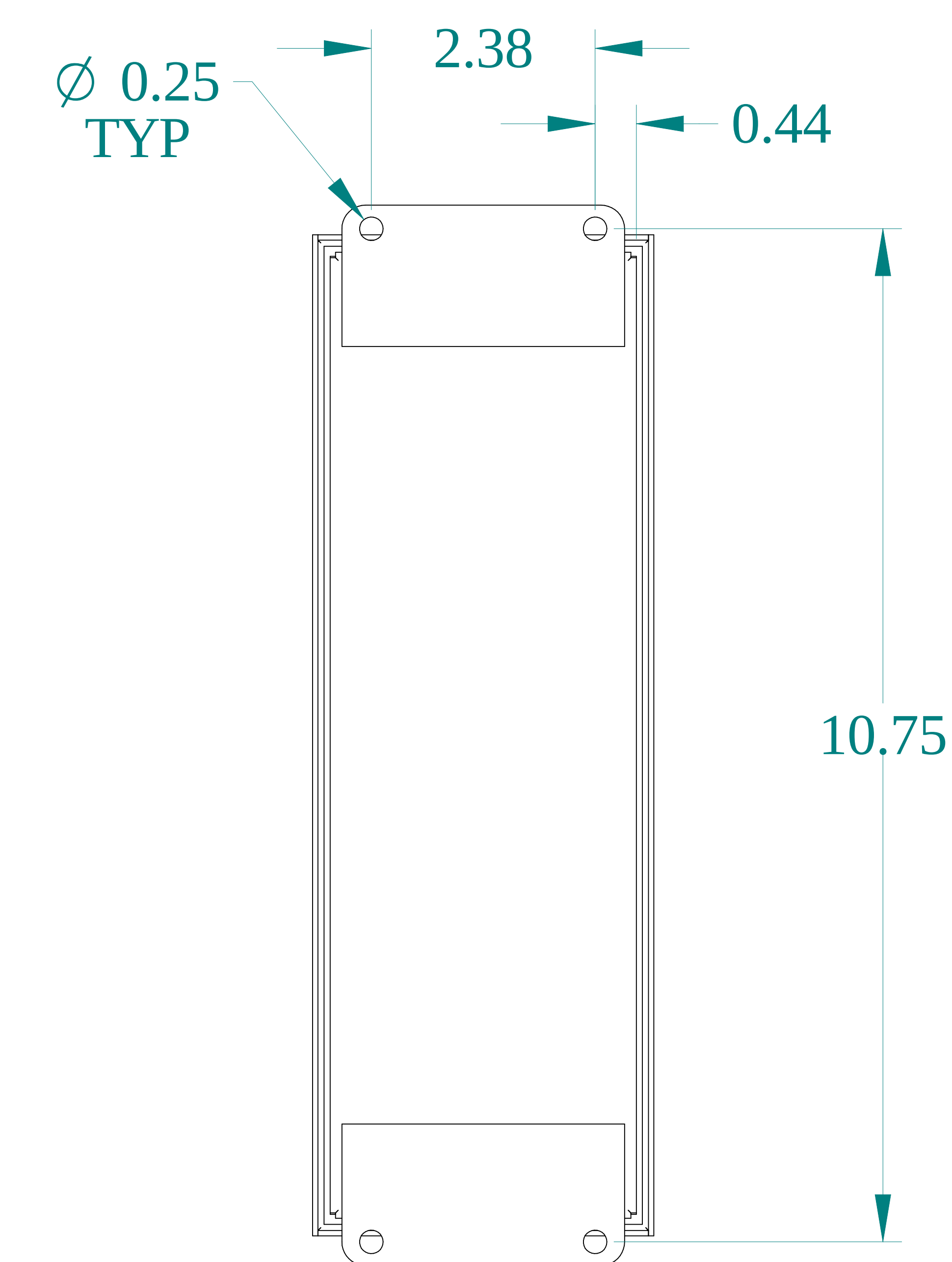
BACK VIEW
